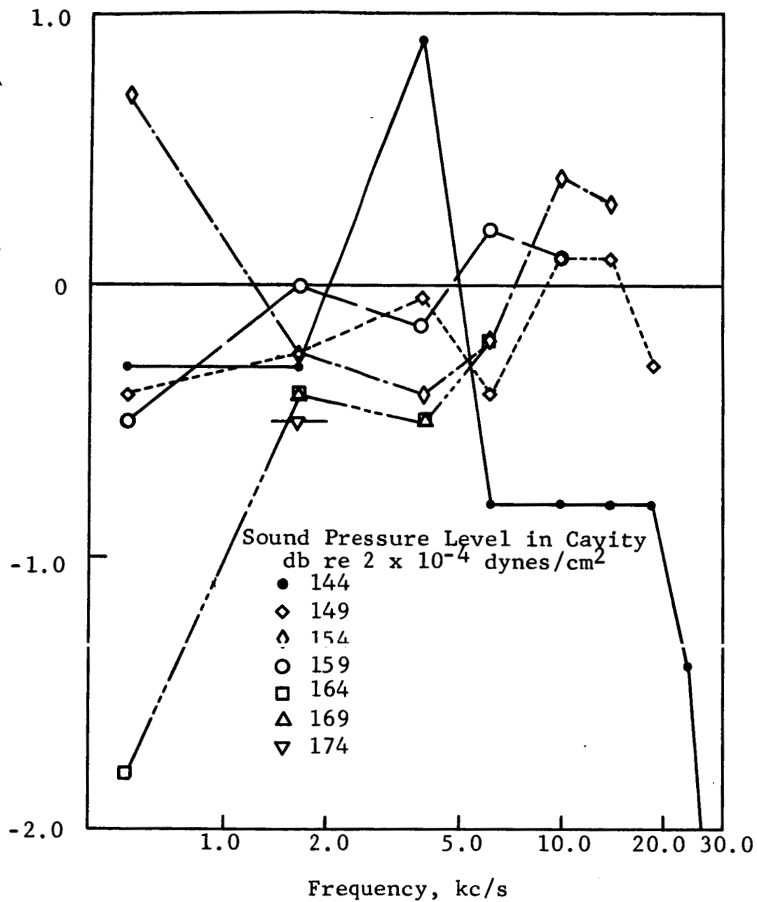
Fig. 19. Comparison of the Sound Pressure Levels in the Acoustic Cavity Measured with Precalibrated Microphone and Instrument.
