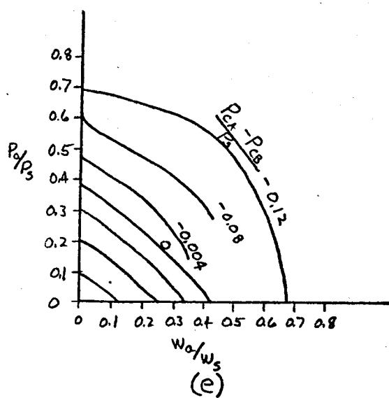
FIG. 19. FLUIDIC ELEMENT CHARACTERISTICS
