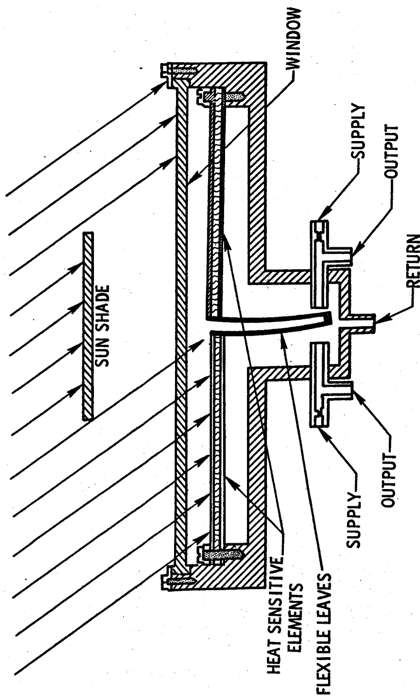
Fig. 11. Sun sensor.
