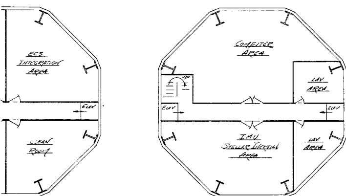
PLAN VIEW FIRST FLOOR
