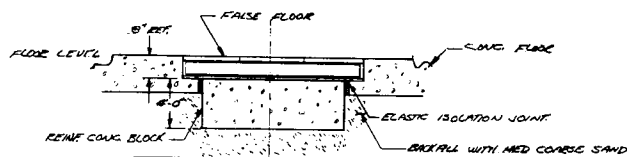
DET 3 CENTRIFUGE PAD (NO SEALS)
