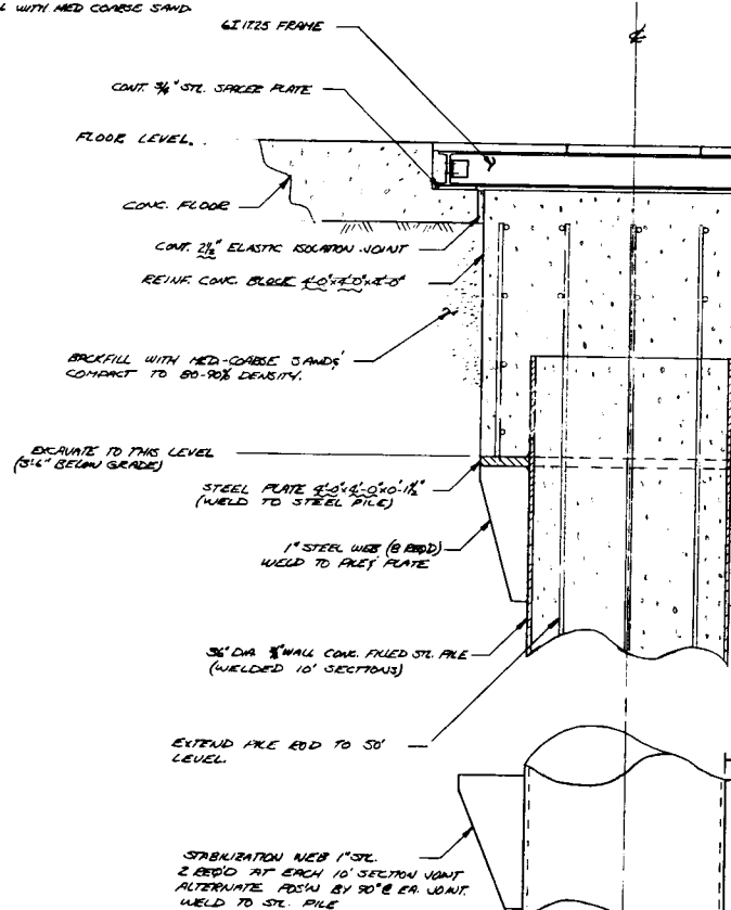
DET 1 STABILIZED TEST PAD
