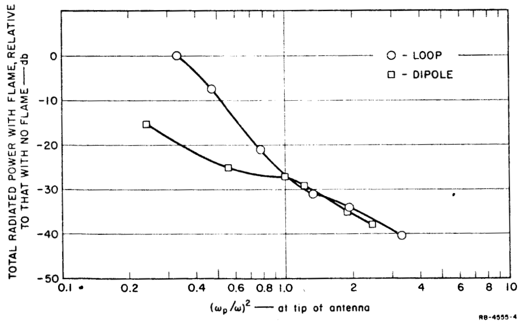
FIG. 6 DROP IN TOTAL RADIATED POWER DUE TO FLAME vs. NORMALIZED PLASMA FREQUENCY
