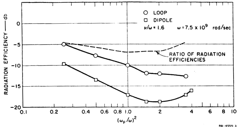
FIG. 7 CALCULATED RADIATION FREQUENCY FOR DIPOLE AND LOOP IN INFINITE, HOMOGENEOUS PLASMA vs. NORMALIZED PLASMA FREQUENCY
