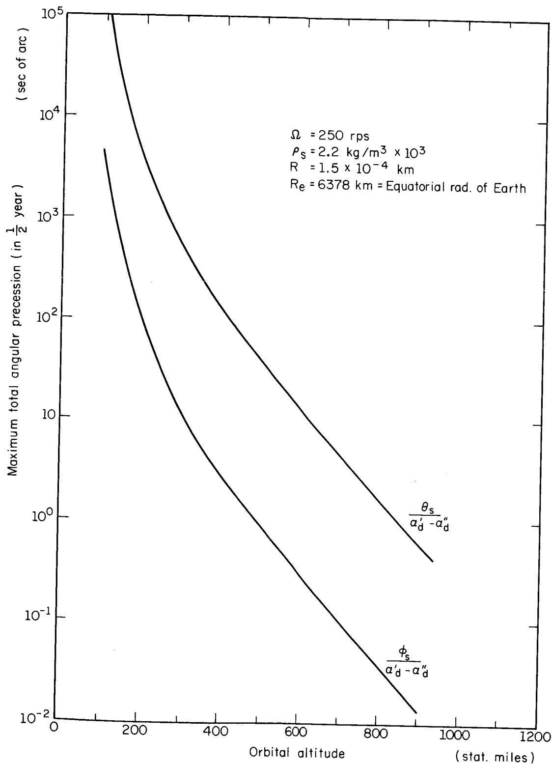
Fig. 6.3. Aerodynamic precession resulting from nonuniform heating plotted as a function of altitude.
