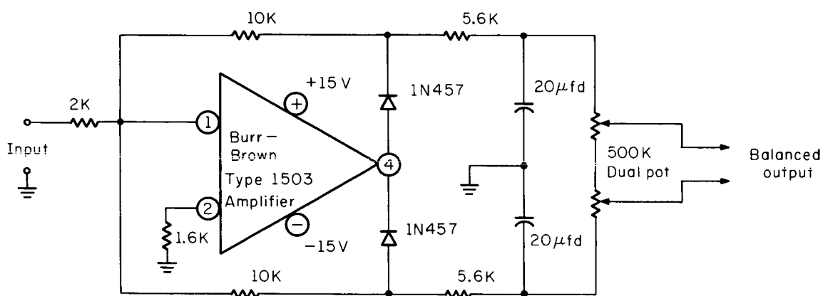
Fig. 6.9. Schematic diagram of the rectifier-filter circuit for the differential-absorption data-reduction system.
