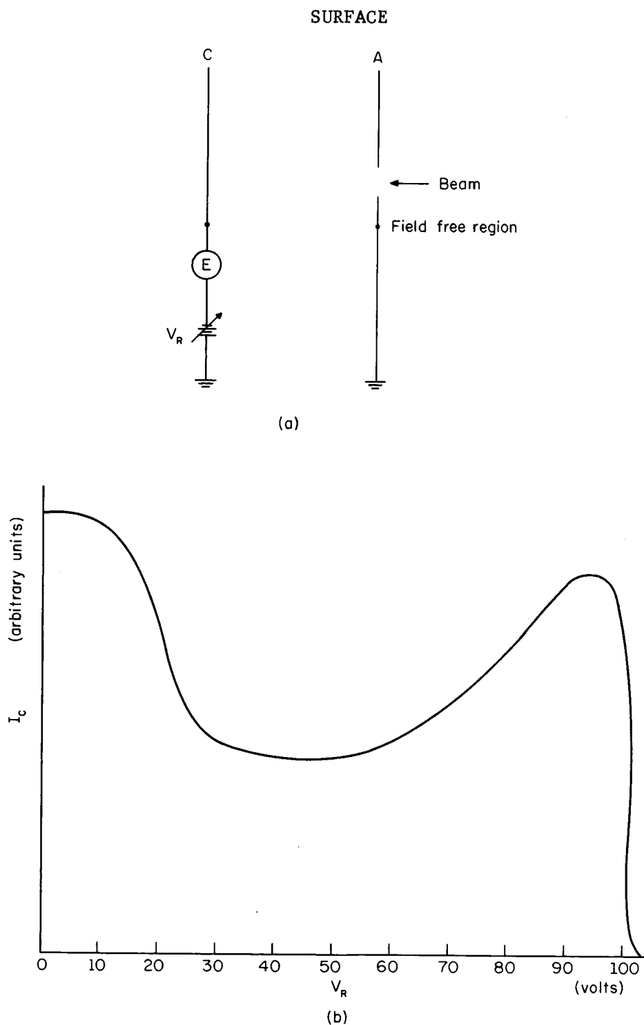
Fig. 1.9. Retarding-potential system and typical retarding-potential curve from the analysis of the distribution in Fig. 1.8(a). The symbols are C = collector plate, A = aperture, V_R = retarding potential, E = electrometer for measurement of current to collector plate.
