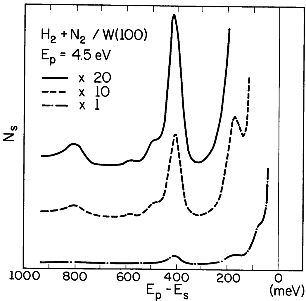
Fig. 1.5. Energy distribution of electrons scattered from 100 W after exposure to H_2 and N_2 .
