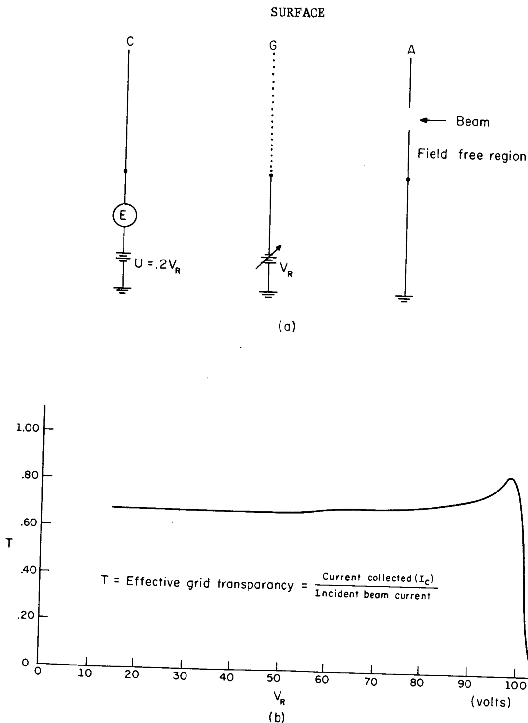
Fig. 1.13. Retarding-potential system and calculated curve resulting from the analysis of a 100-eV beam. The symbols are C = collector plate, A = aperture, V_R = retarding potential, E = electrometer for measurement of current to collector plate, U = accelerating voltage.
