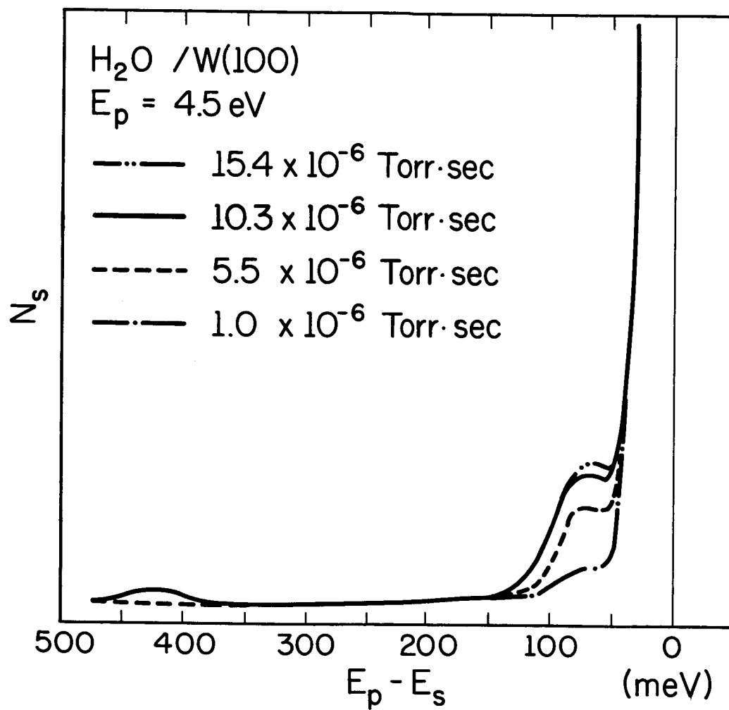
Fig. 1.3. Energy distribution of electrons scattered from 100 W after exposure to H_2O .
