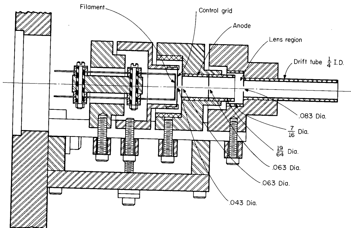
Fig. 1.6 Electron gun.
