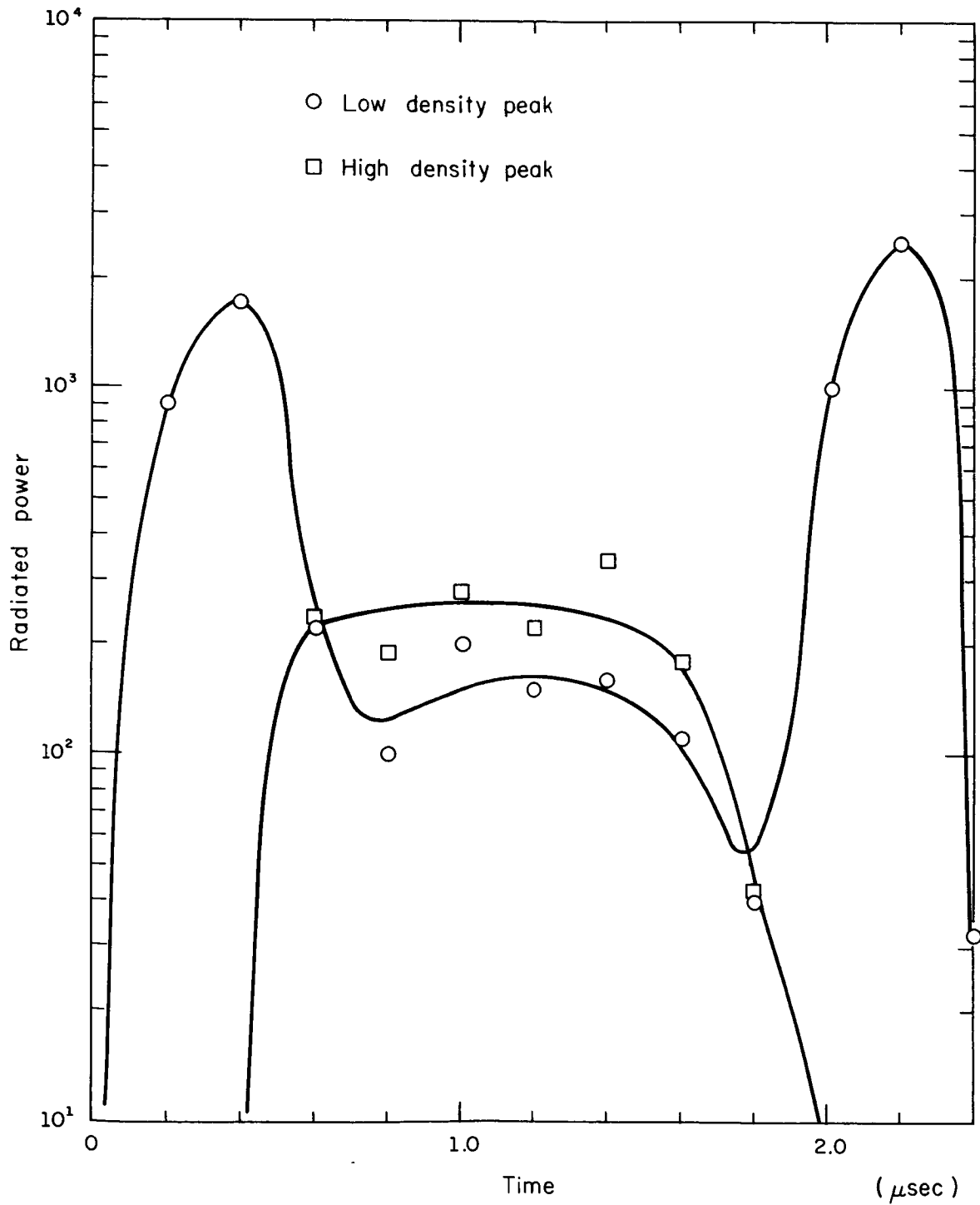
Fig. 3.5. Time-resolved spectrum.
