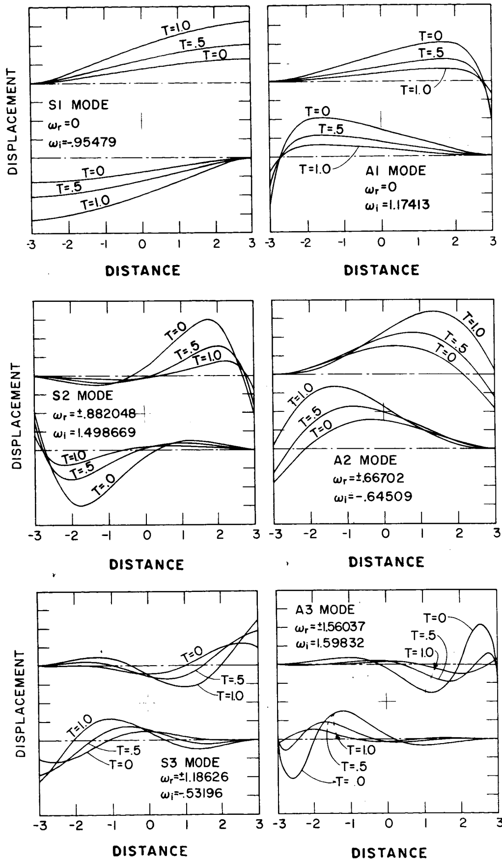
Figure 12. Time dependant eigenfunctions for the three lowest symmetric and antisymmetric modes for the conditions of Figure 10. I\omega_e/V_0 = 3
