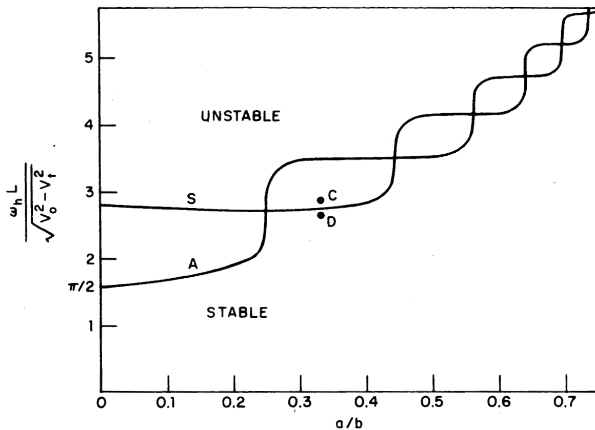
Figure 15. Effect of transverse geometry on the normalized length at the point of impending instability for the fundamental symmetric and antisymmetric modes. The conditions are the same as in Figure 14.
