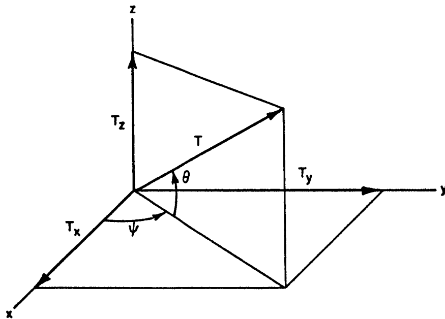
FIGURE A2. THRUST VECTOR COMPONENTS
