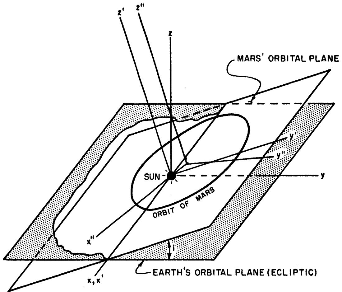
FIGURE A1. COORDINATE SYSTEMS
