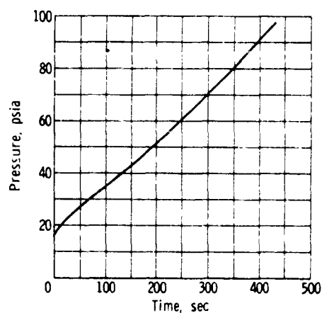
(a) Total pressure as function of time.
