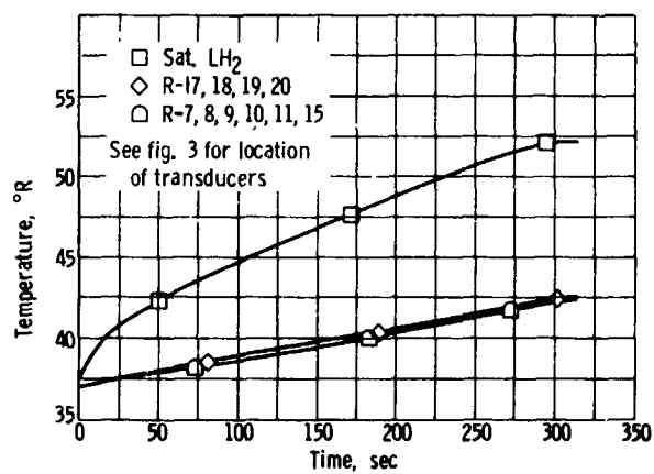
(d) Lower inner sphere temperature as function of time.
