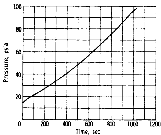
(a) Total pressure as function of time.
