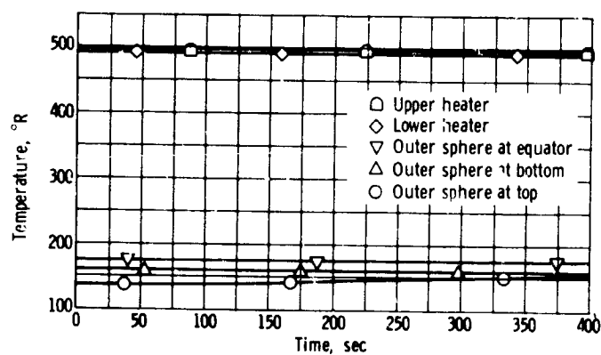
(b) Outer sphere and heater temperature as function of time.
