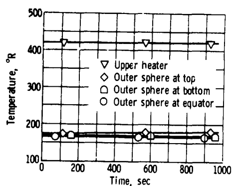
(b) Outer sphere and heater temperature as function of time.
