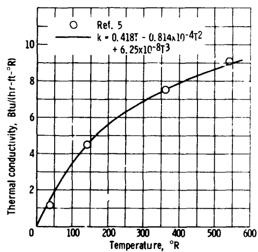
Figure 21. - Stainless steel thermal conductivity as function of temperature.
