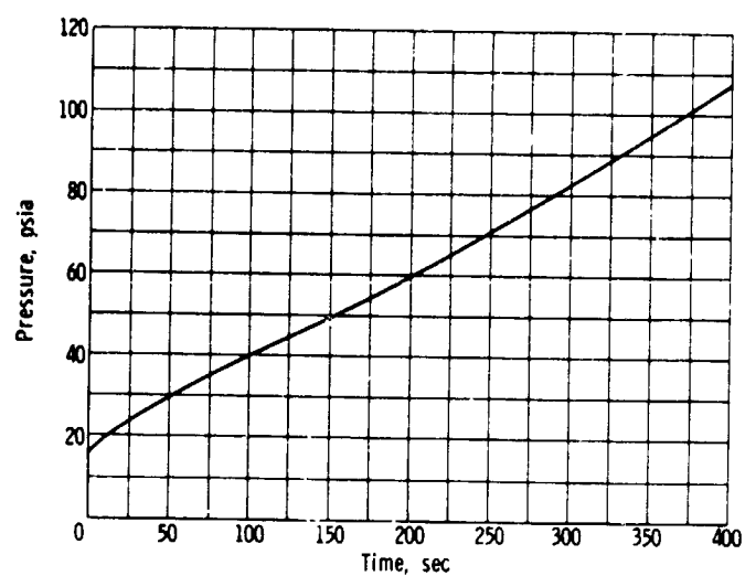
(a) Total pressure as function of time.
