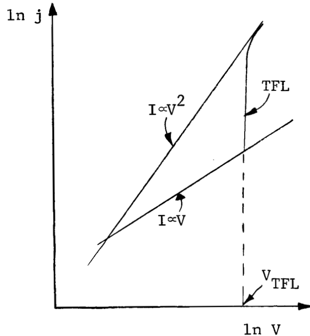
Graph (6). The "Lampert Triangle".
