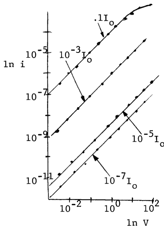
Figure (18). I-V curve for ohmic aluminum electrodes.
