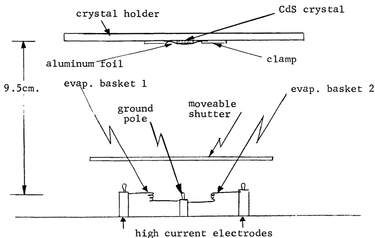
Figure (8). Schematic of components used for evaporation.
