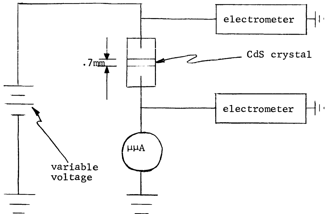
Figure (11). Electrical circuit used in I-V measurements.
