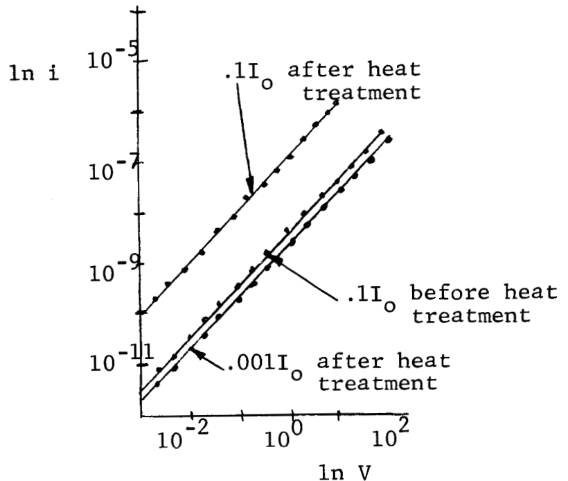
Figure (15). I-V curve for an indium electrode.
