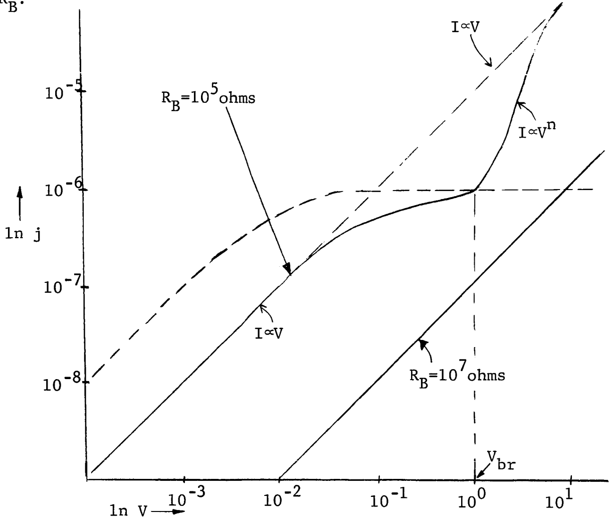
Graph (4). I-V profile for j'_0 = 10^{-6} \text{ amps/cm}^2 , assuming that barrier thickness is 10^{-6} \text{ cm} , shown for cases when bulk resistance is 10^5 \text{ ohms} and 10^7 \text{ ohms} .
