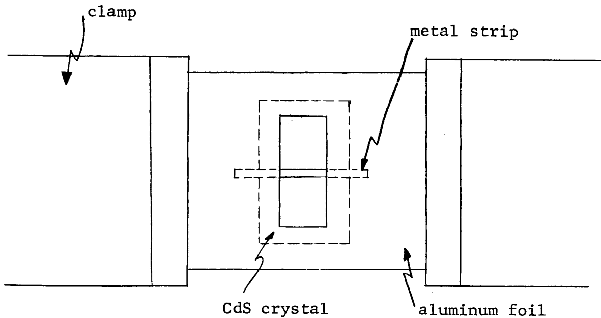
Figure (6). Top and side view of crystal as it is positioned on the crystal holder.
