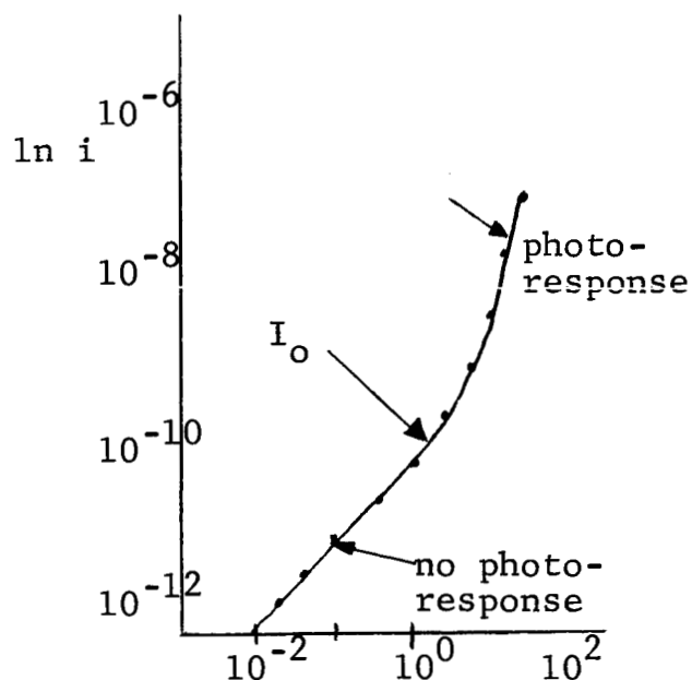
Figure (17). I-V curve for non-ohmic aluminum electrodes.
