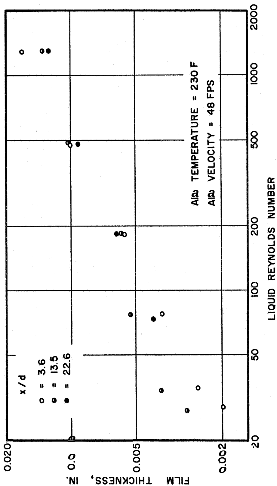
Fig. 16 Mean Film Thickness as a Function of Liquid Reynolds Number
