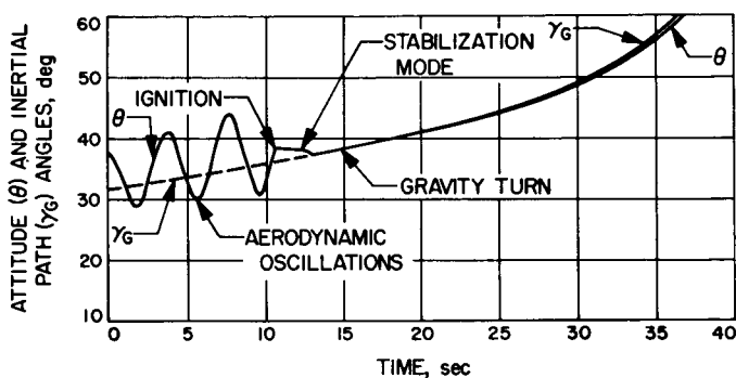
Fig. 3. Three-deg-of-freedom data
