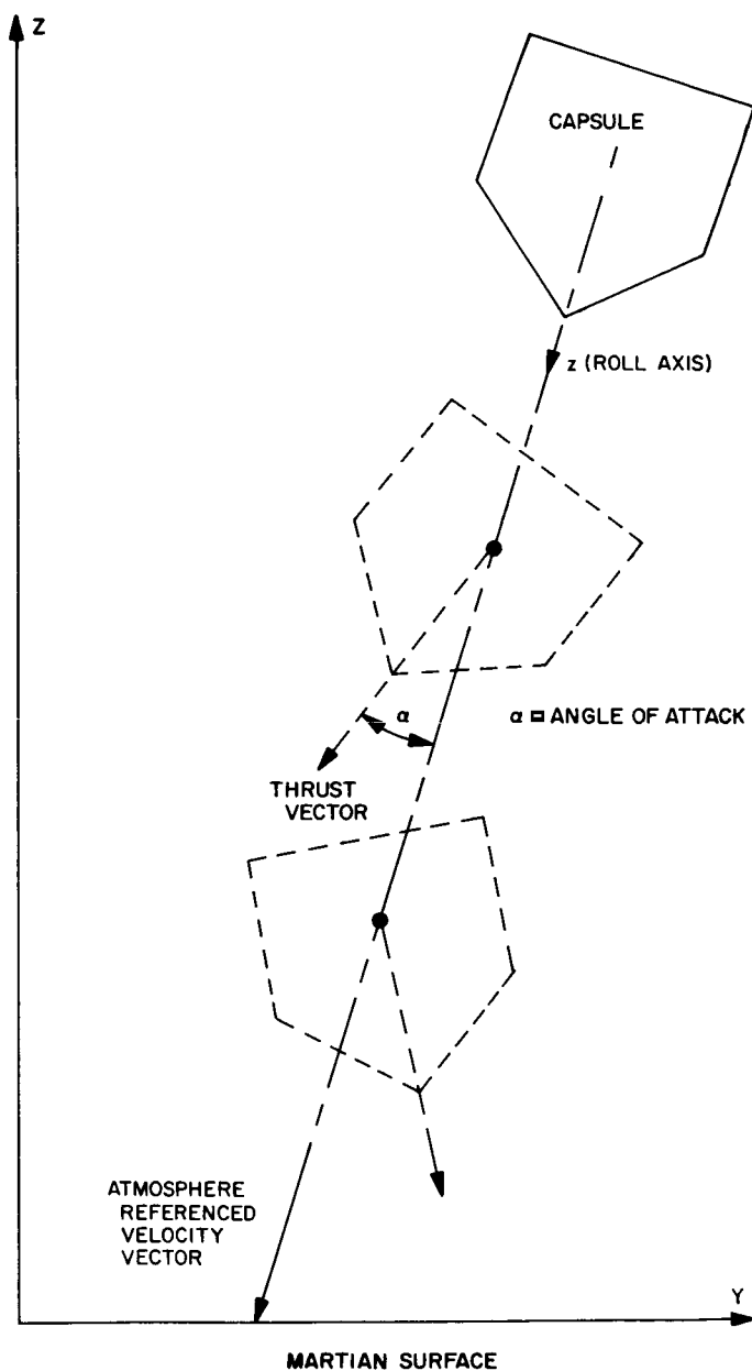
Fig. 2. Aerodynamic oscillations
