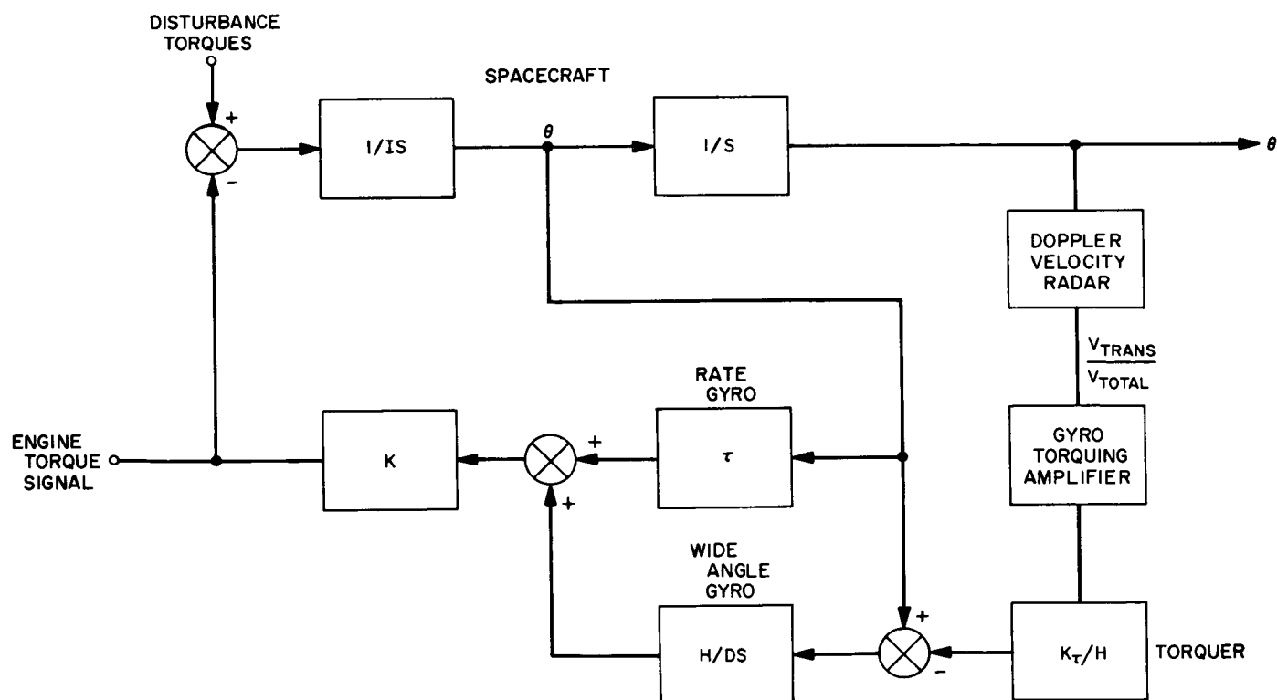
Fig. 14. Pitch and yaw control loop for gravity turn
