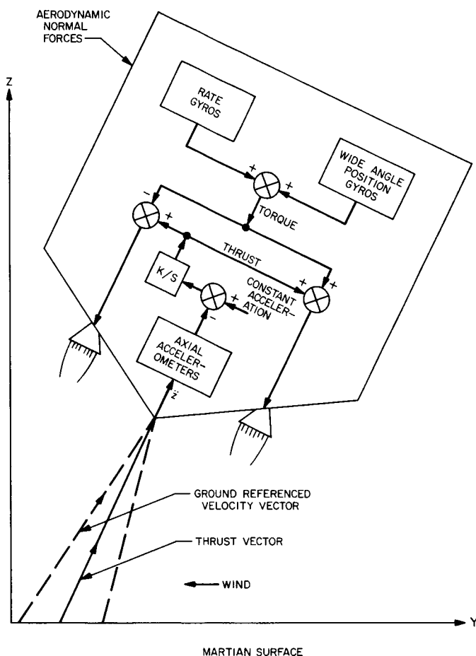
Fig. 4. Stabilization mode
