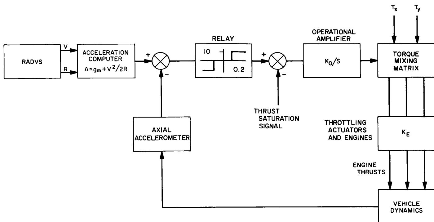
Fig. 13. Simplified gravity turn thrust control loop
