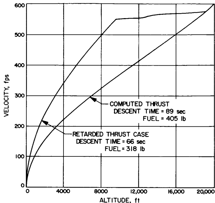
Fig. 16. AM-10 retarded thrust comparison
