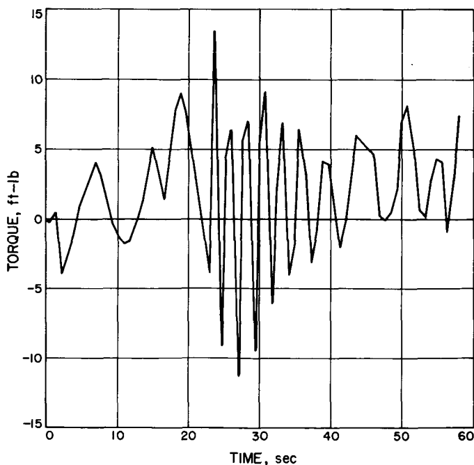
Fig. 12. AM-10 fuel slosh torque
