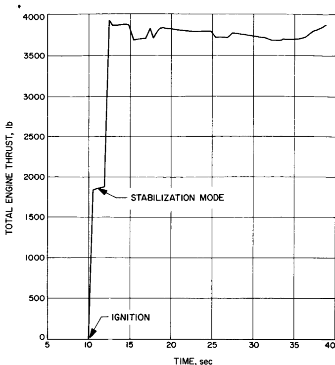
Fig. 15. Thrust profile
