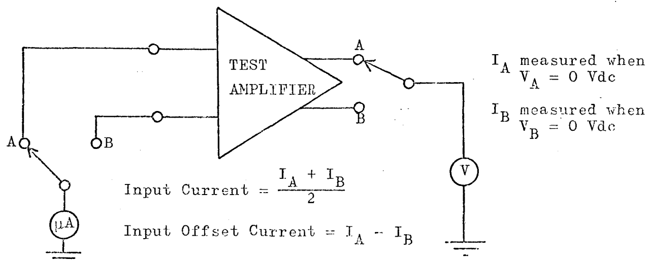
Figure 3-2. Input Current ( I_i ) and Input Offset Current ( I_{io} )
