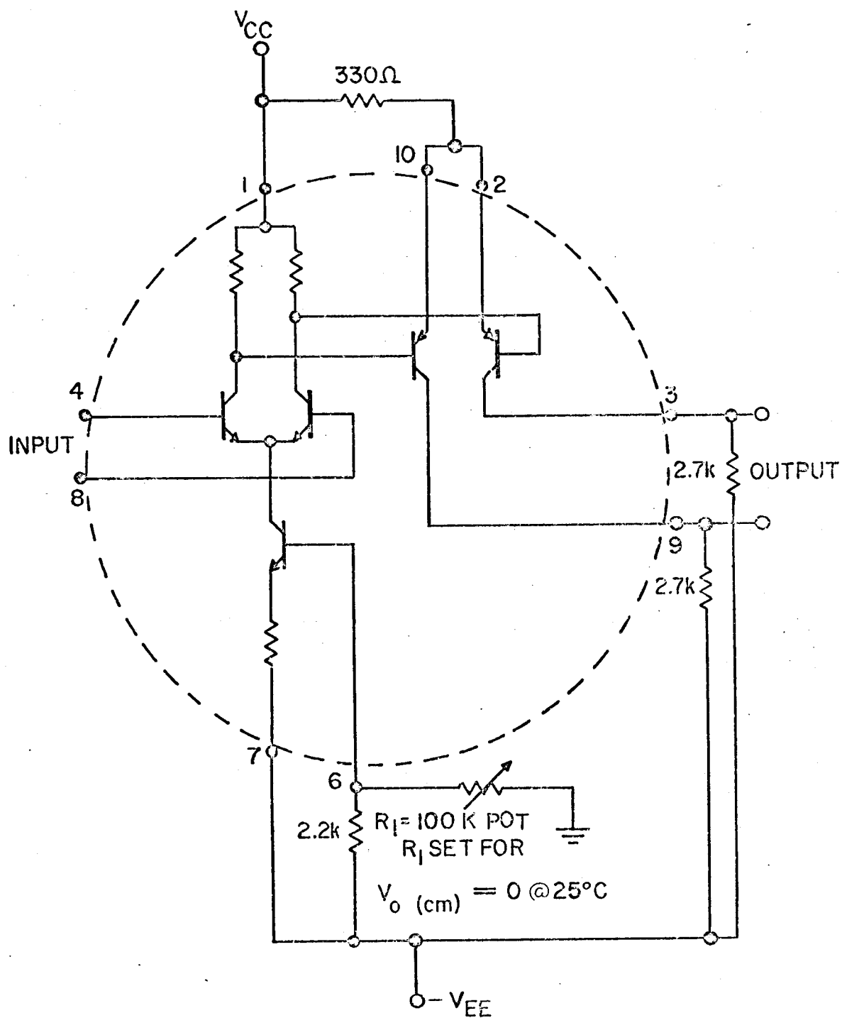
Figure 2-2. MC-1519 in Common Emitter (CE) Mode
