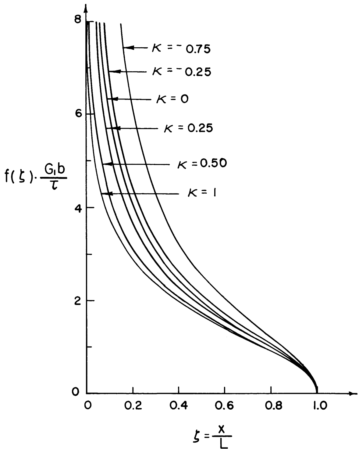
Figure III-2: f(\xi) , the dislocation distribution function, versus \xi = x/L for different relative rigidity ratios ( K ).
