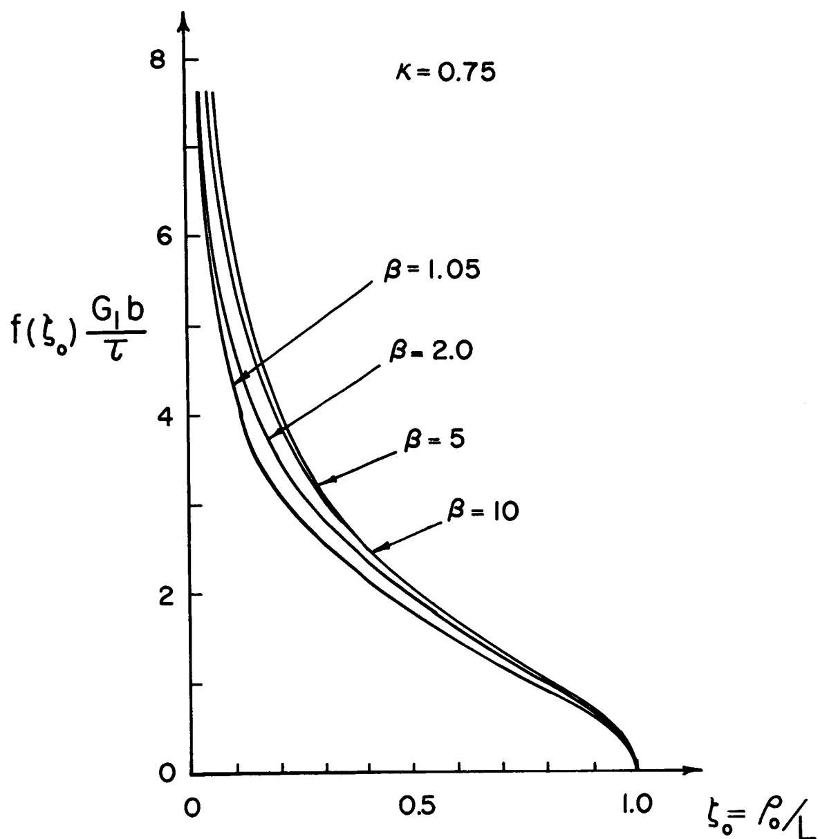
Figure IV-3: f(\xi_0) , the dislocation distribution function, vs. \xi_0 for a fixed relative rigidity ( \kappa ) and various L/R ratios. The pileup is in the softer phase ( G_2 > G_1 ). \rho_0 is the distance from the leading edge of the pileup to any point in the array.
