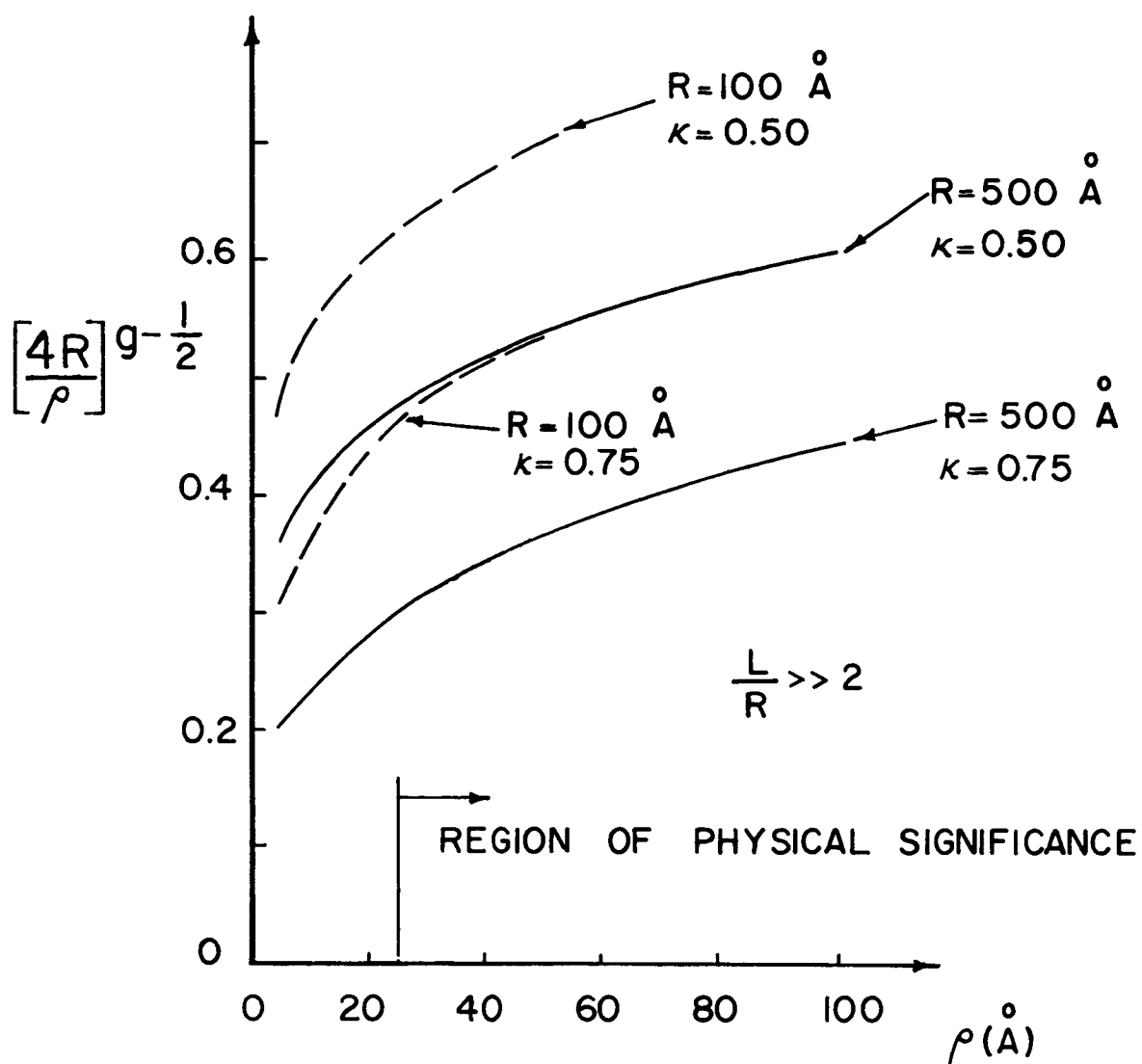
Figure IV-11: The "correction factor" for the local stresses in the second phase as a function of \rho for two particles of different size and different relative rigidities.
