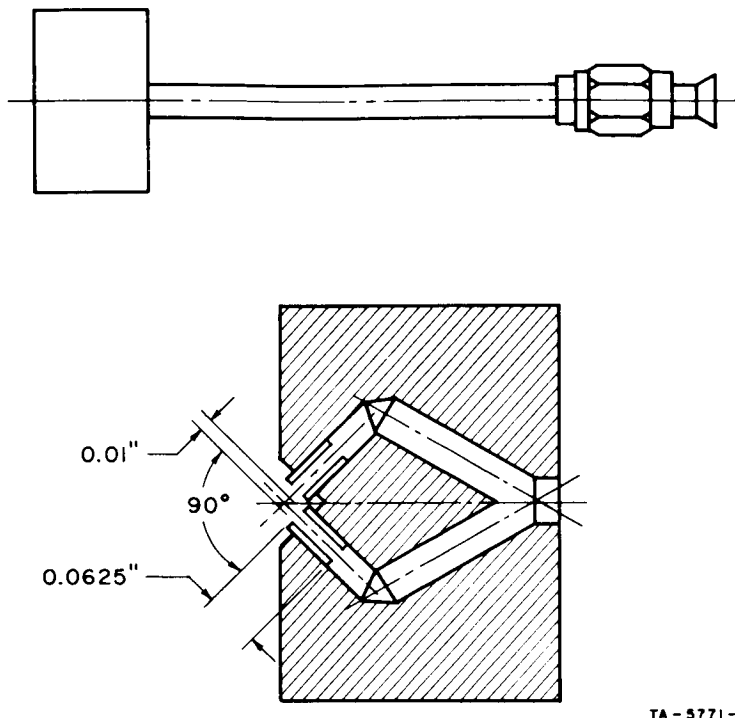
FIG. 29 DIAGRAM OF THE IMPINGING JET ATOMIZER
