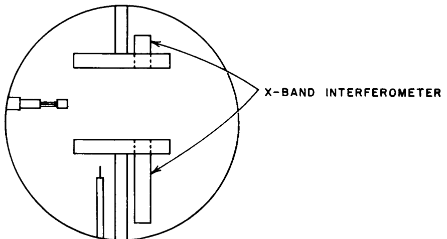
FIG. 12 SKETCH SHOWING X-BAND MICROWAVE INTERFEROMETER AND HARP STRUCTURE MOUNTED IN THE SHOCK TUBE
