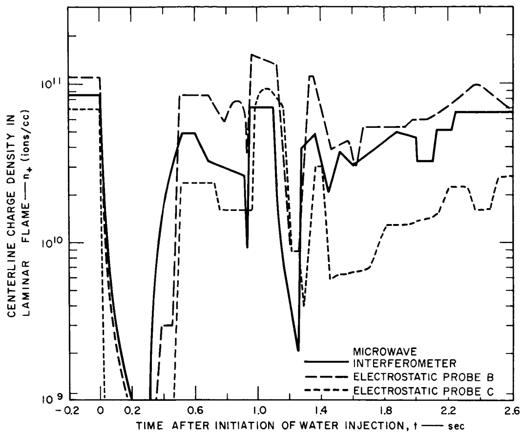
FIG. 34 ABSOLUTE CHARGE DENSITY LEVELS IN THE LAMINAR FLAME AFTER WATER INJECTION AS INFERRED FROM MICROWAVE INTERFEROMETER MEASUREMENTS AND ELECTROSTATIC PROBES ( P_\infty \approx 10 Torr, U_{Gas} \sim 20 m/sec, P_{inj} = 40 Psig)
