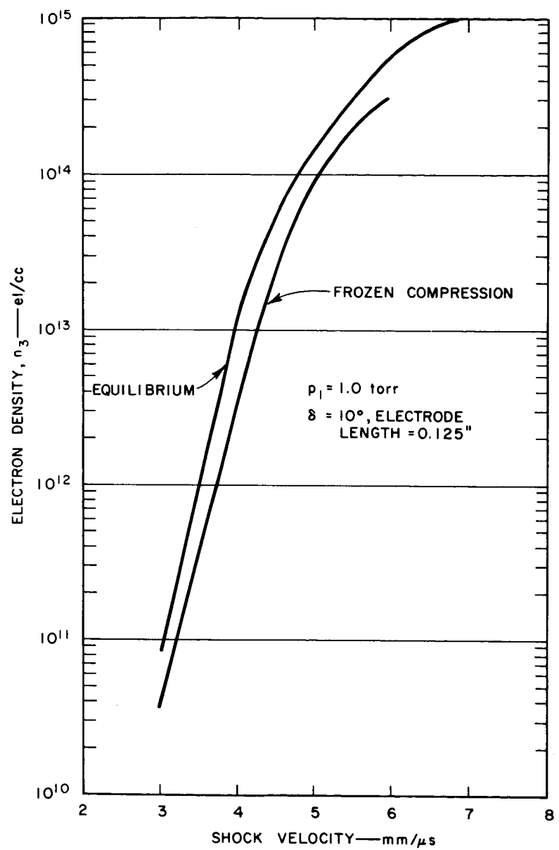
FIG. 8 EQUILIBRIUM ELECTRON DENSITY BEHIND AN OBLIQUE SHOCK
