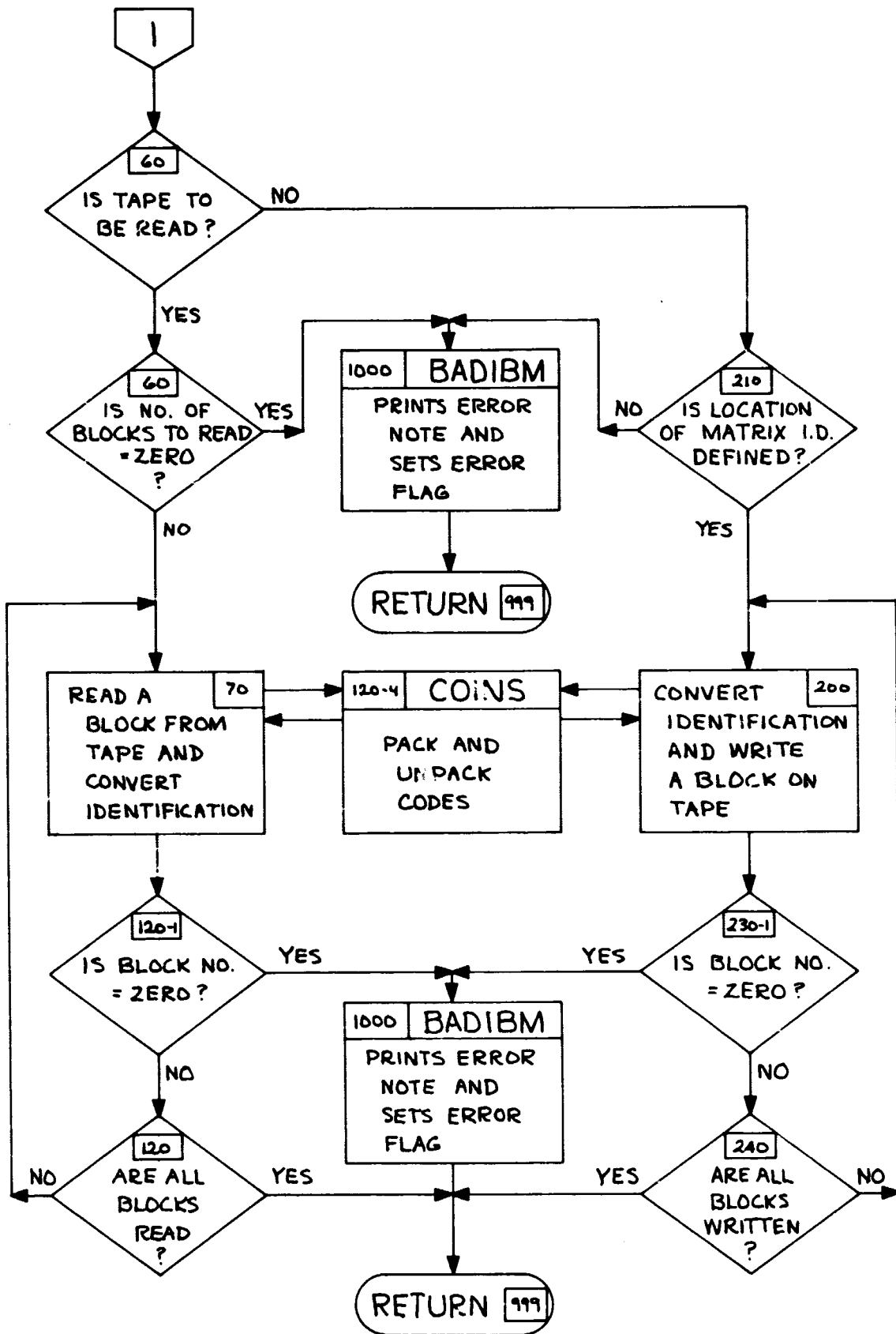
Figure 8-4.7 "TAPES" FLOW
