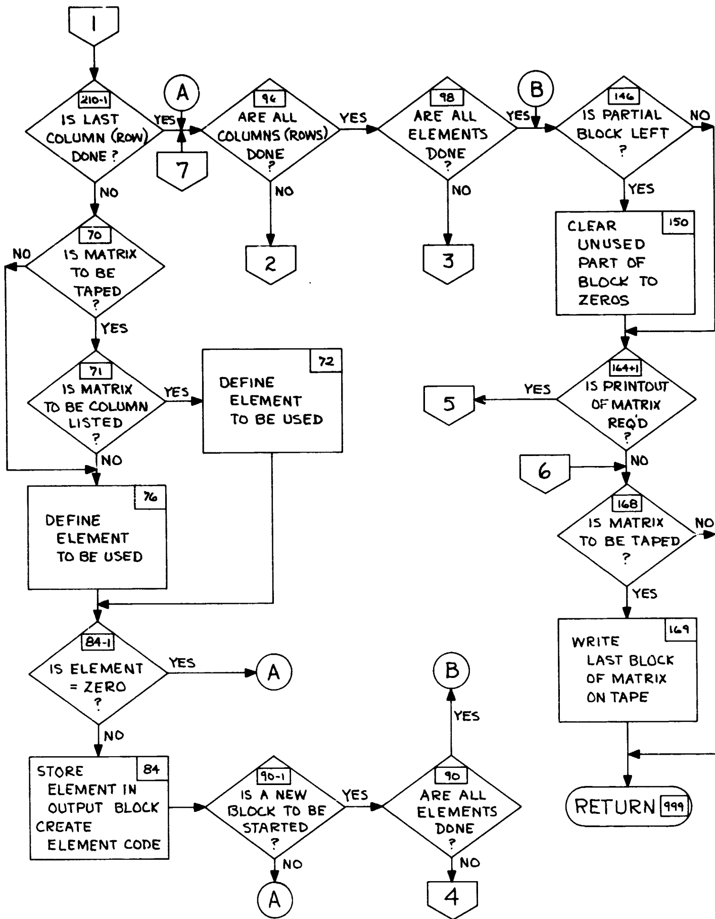
Figure 8-5.5 "COES" FLOW
