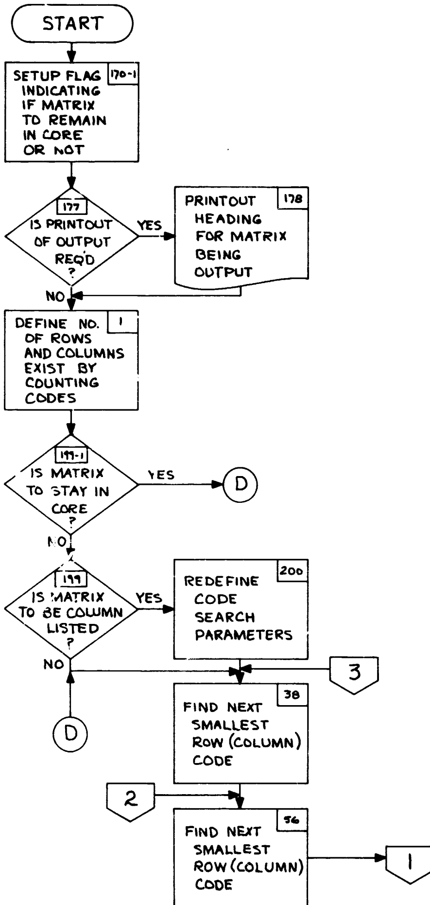
Figure 8-5.5 "COES" FLOW
