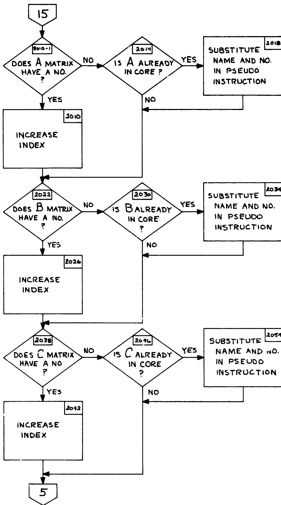
Figure 8-4.5 "MINTS" FLOW
