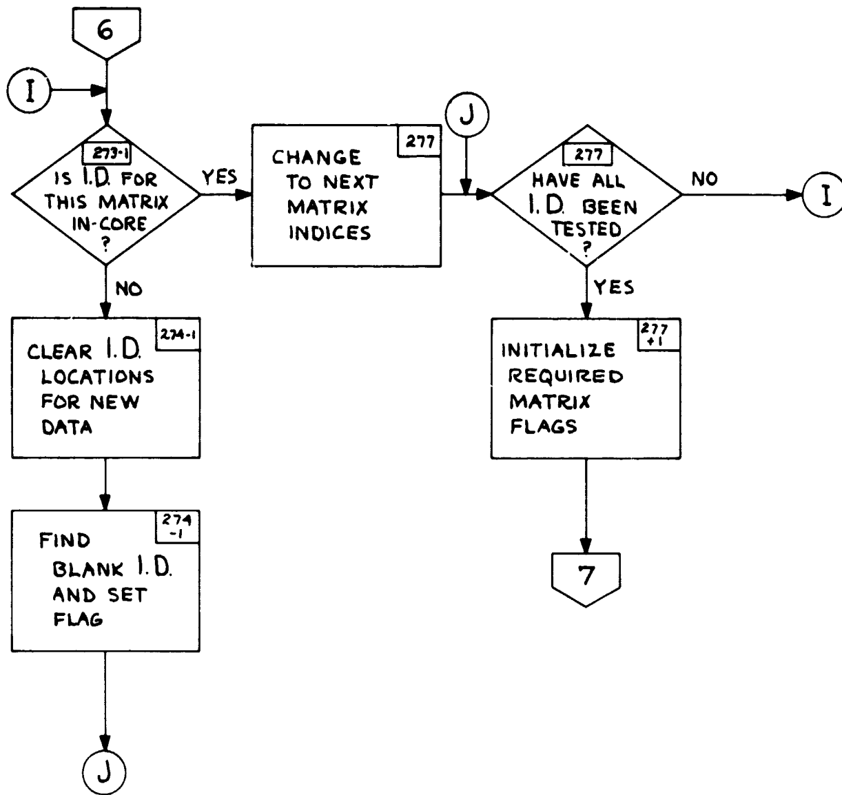
Figure 8-4.5 "MINTS" FLOW
