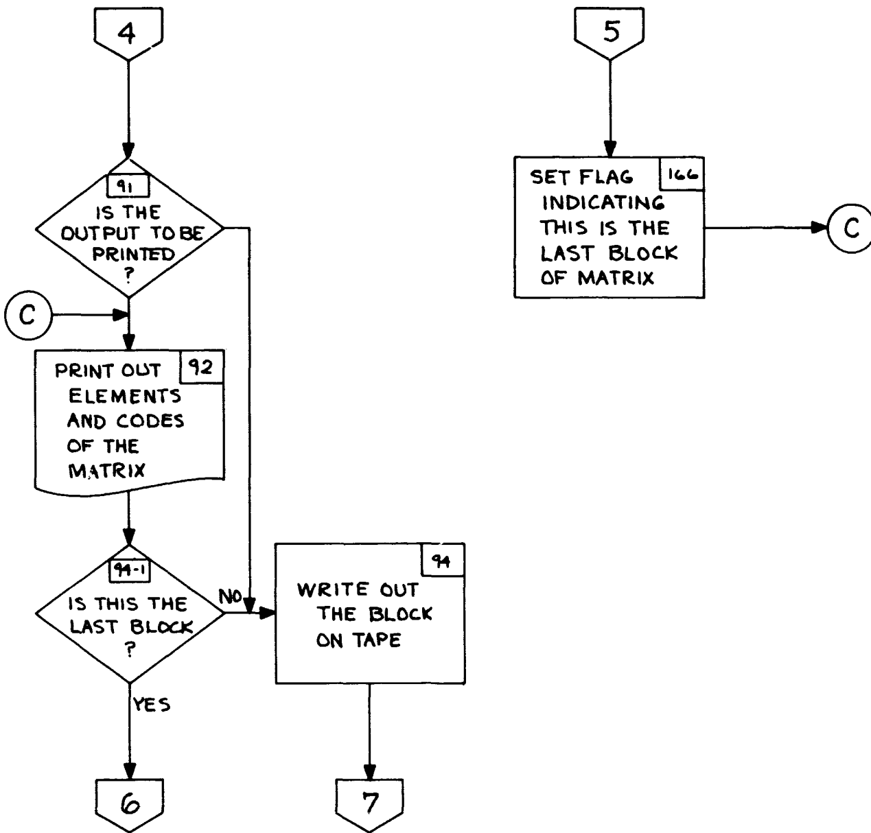
Figure 8-5.5 "COES" FLCW
