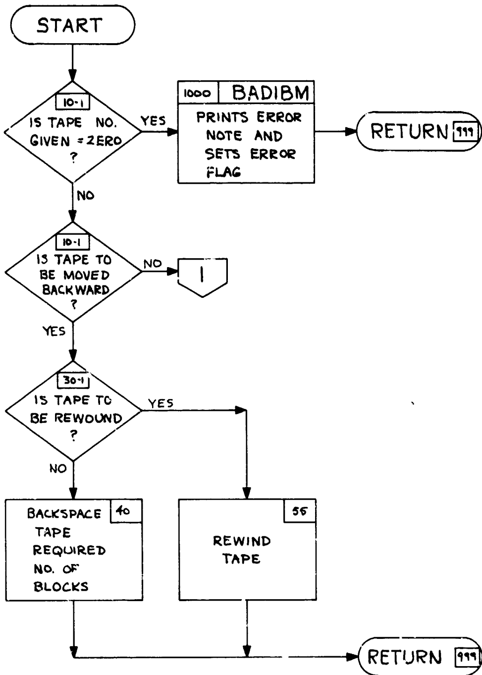
Figure 8-4.7 "TAPES" FLOW
