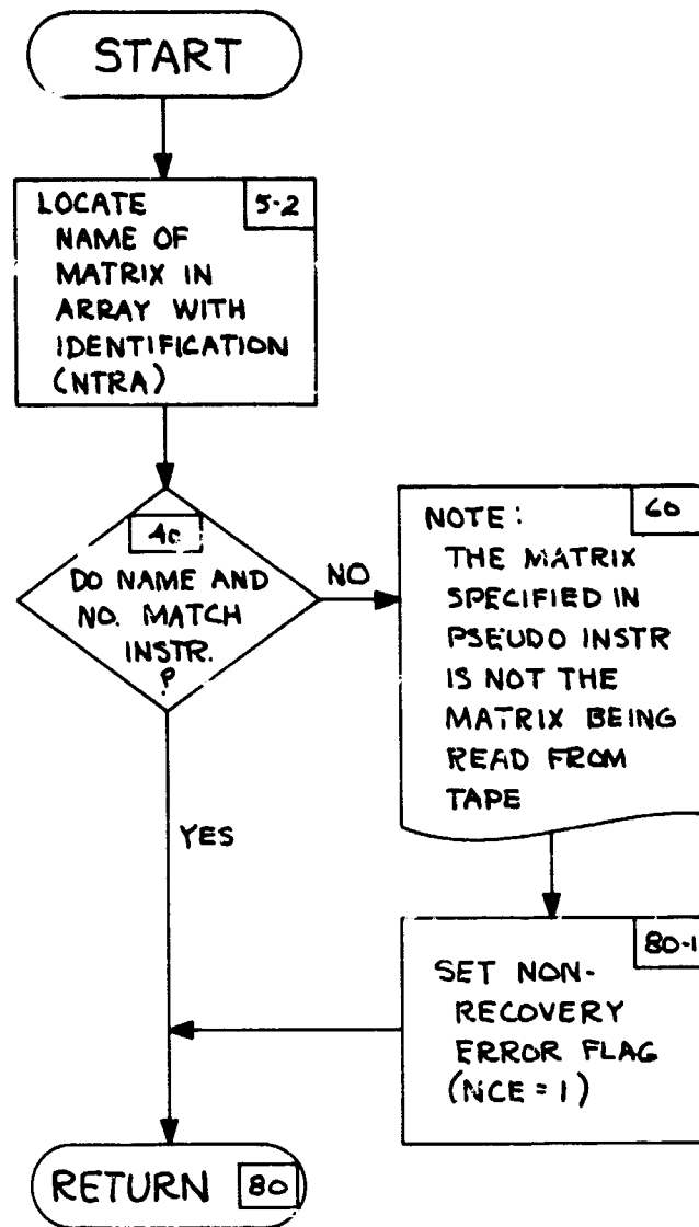
Figure 8-4.6 "TSNAM" FLOW
