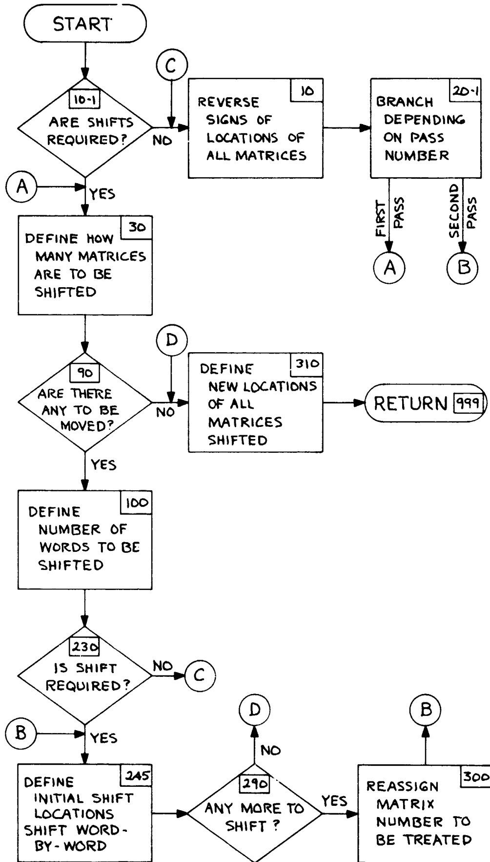
Figure 8-4.3 "SHIFT" FLOW
