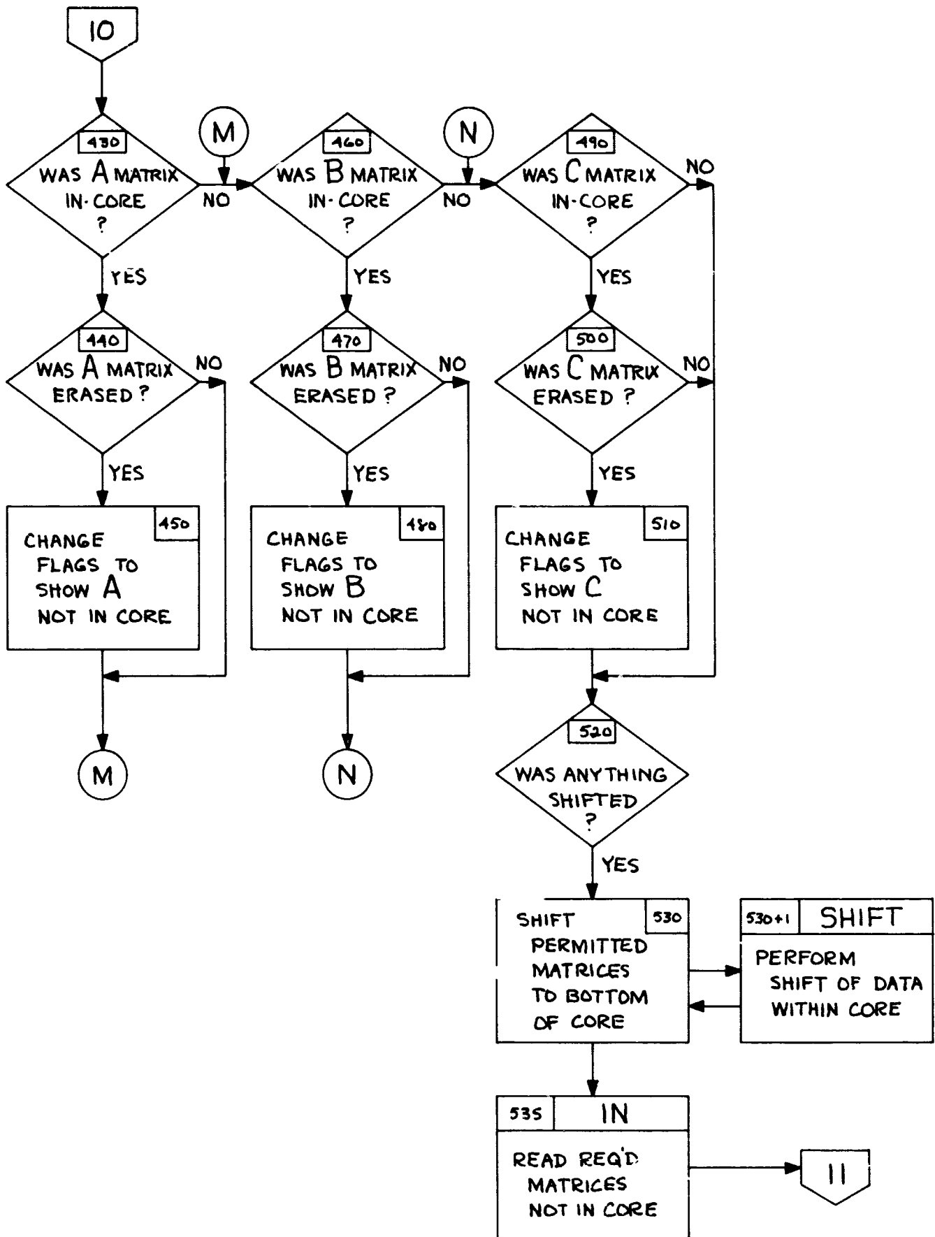
Figure 8-4.5 "MINTS" FLOW
