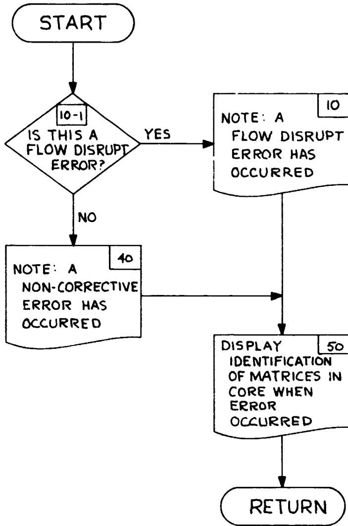
Figure 8-4.1 "ERROR" FLOW
