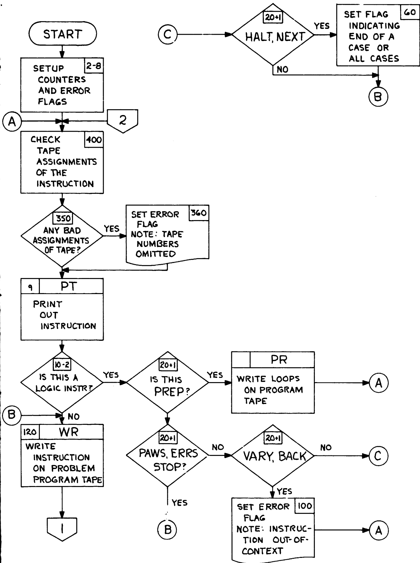
Figure 8-3.2 "MAKER" FLOW
