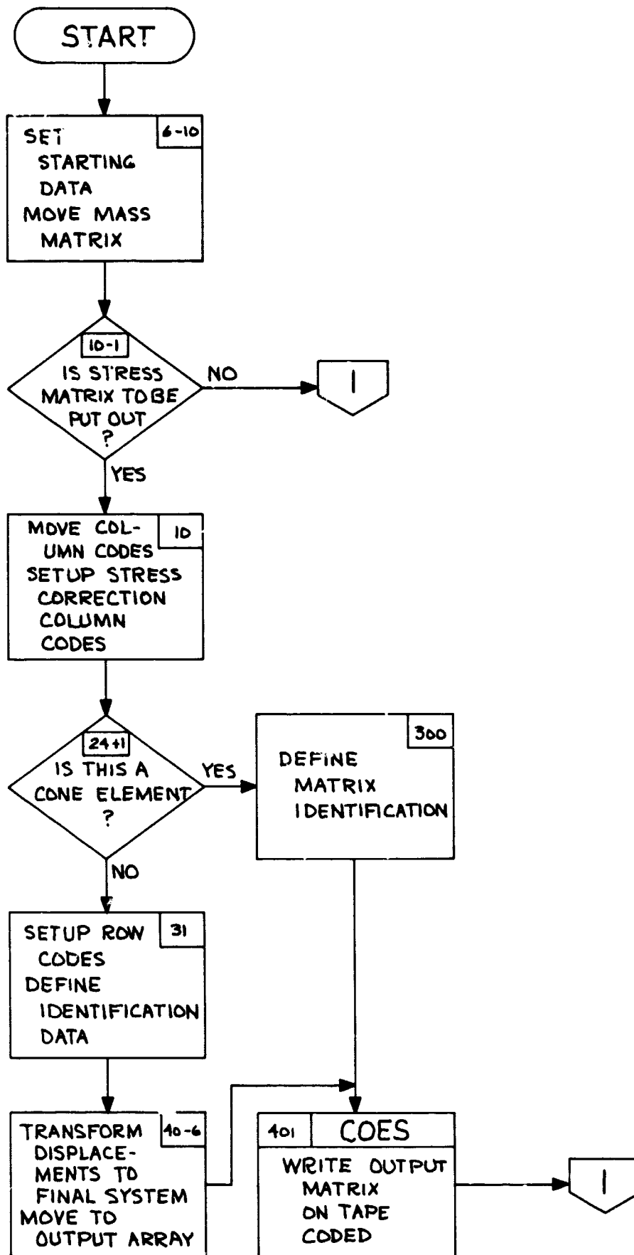
Figure 8-5.2 "SFT" FLOW
