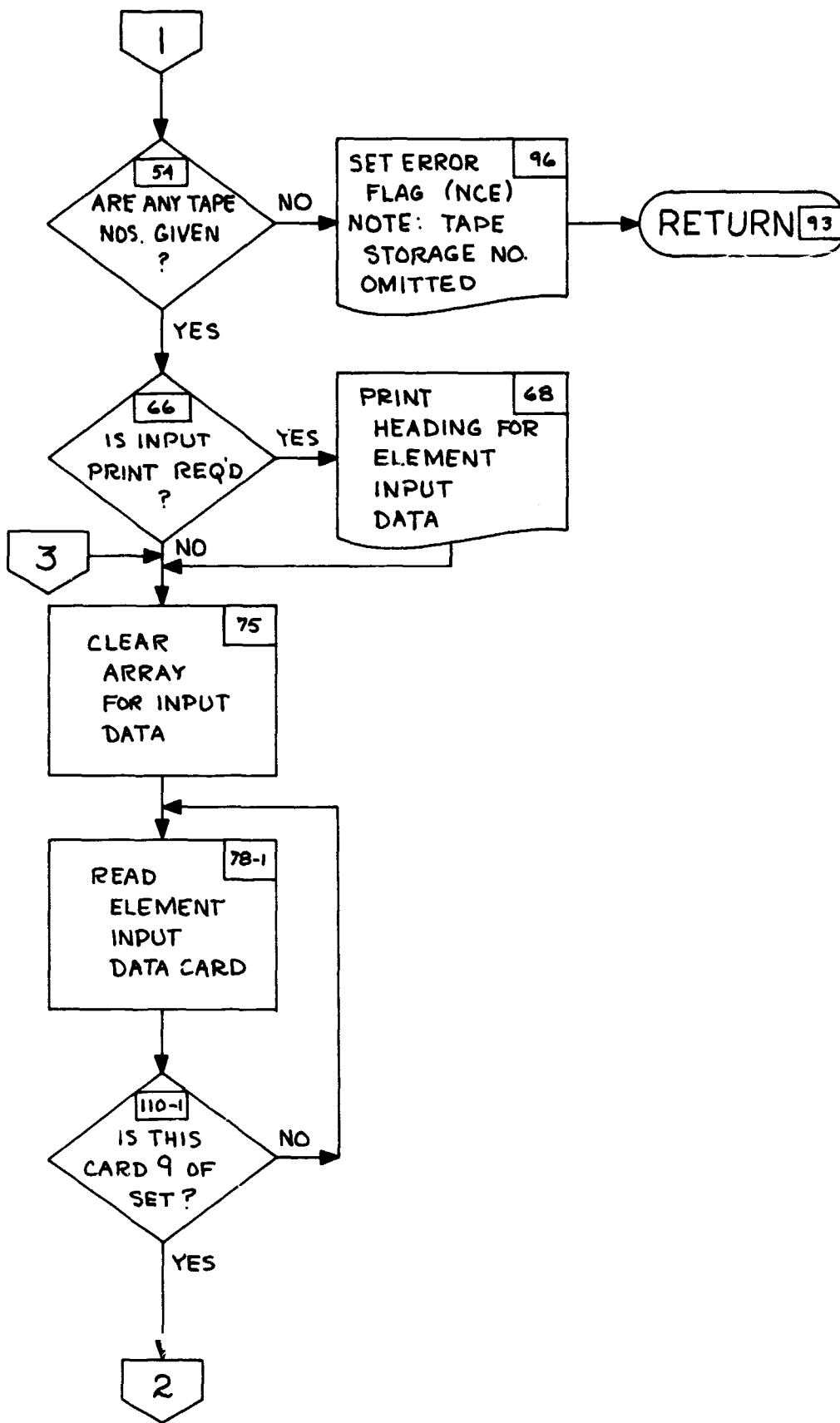
Figure 8-5.1 "BILD" FLOW
