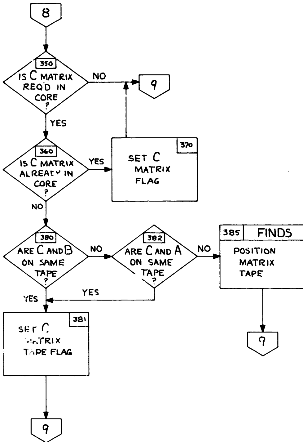
Figure 8-4.5 "MINTS" FLOW
