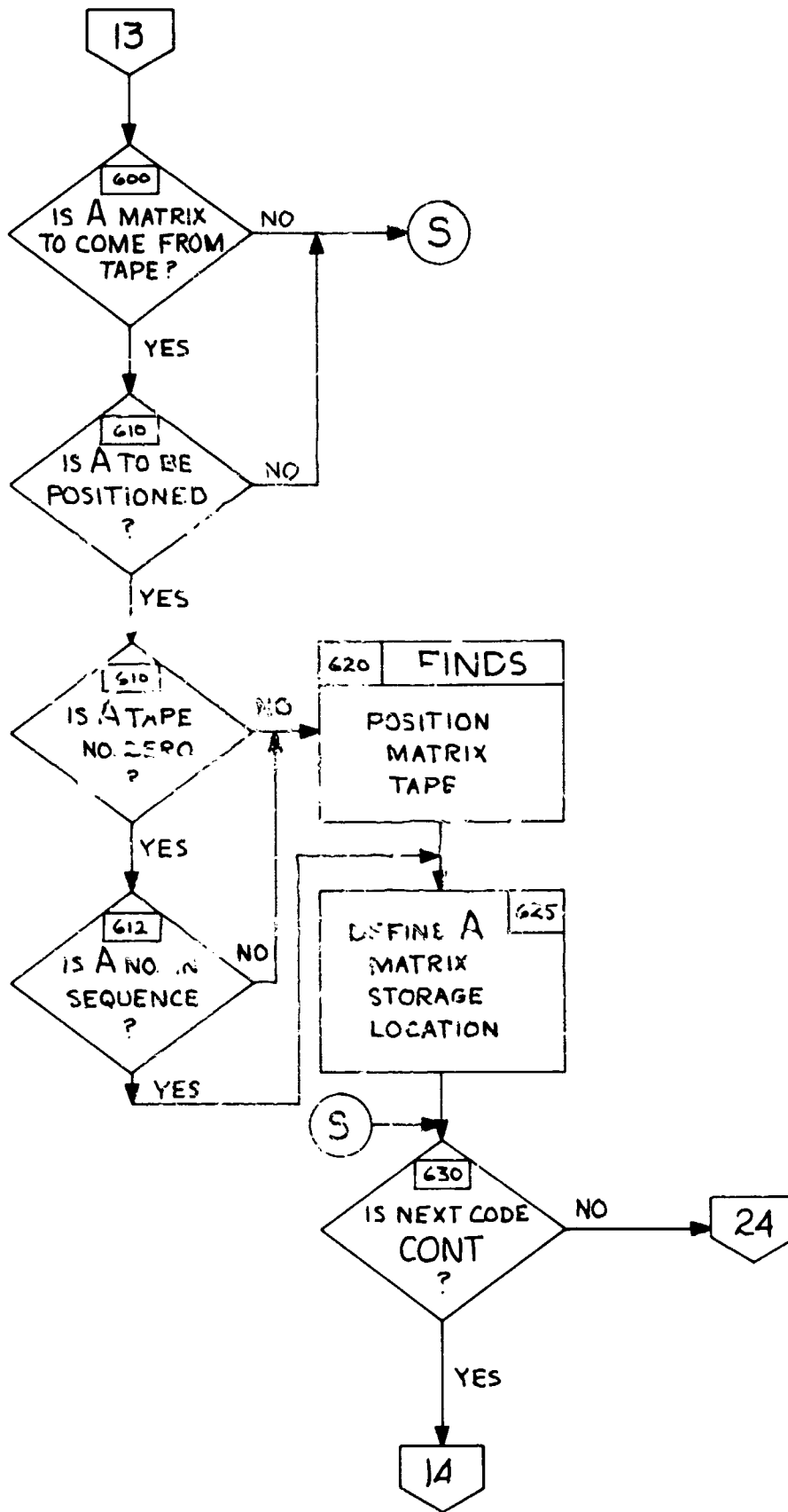
Figure 8-4.5 "MINTS" FLOW
