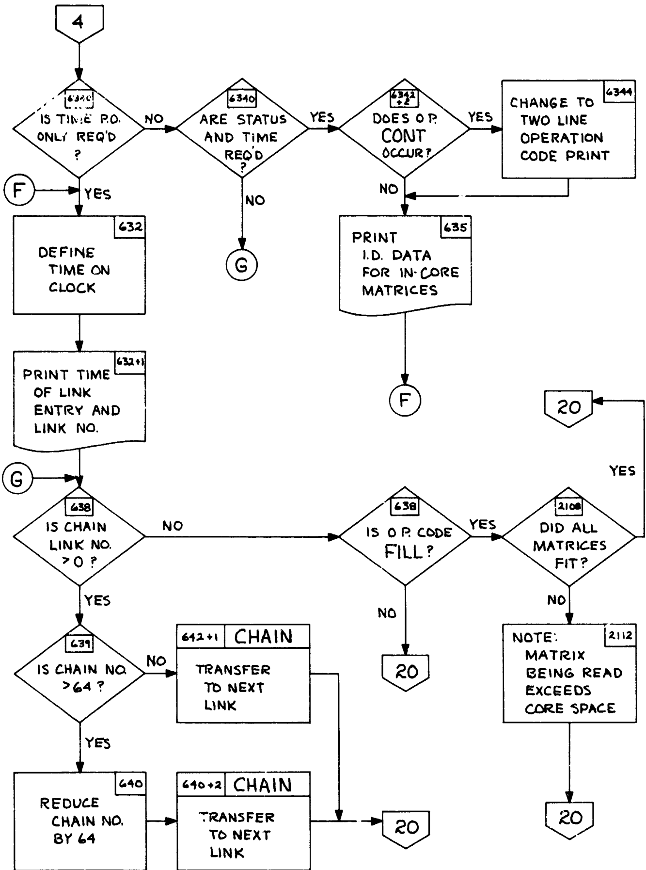
Figure 8-4.5 "MINTS" FLOW
