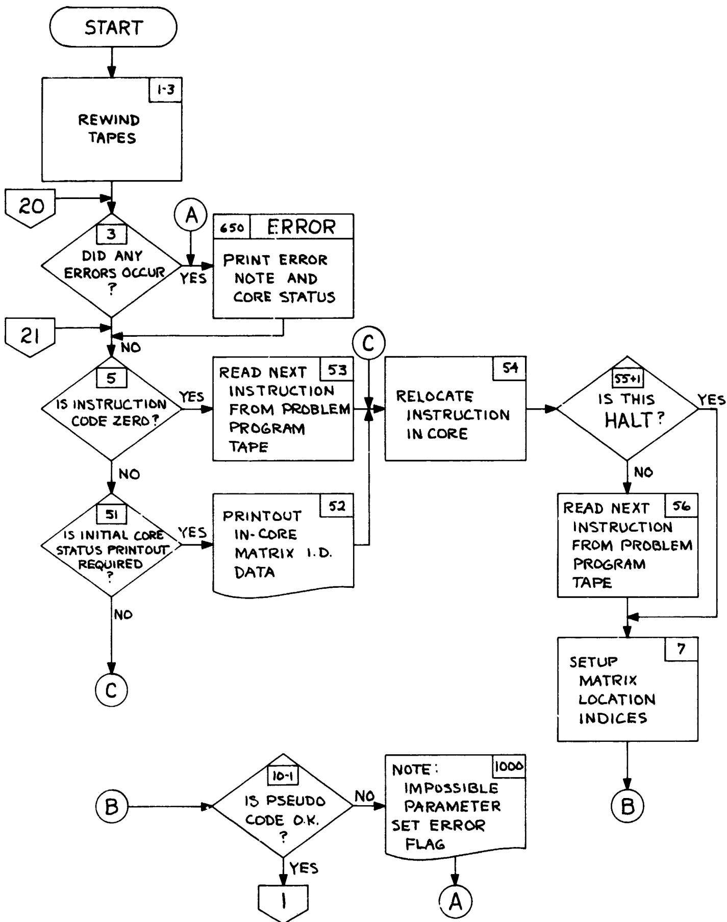
Figure 8-4.5 "MINTS" FLOW
