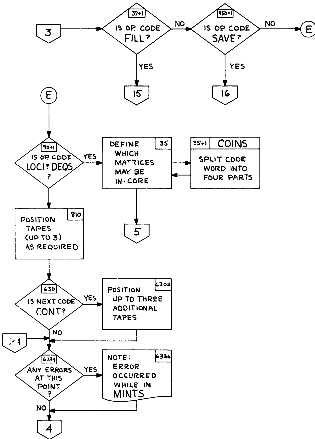
Figure 8-4.5 "MINTS" FLOW
