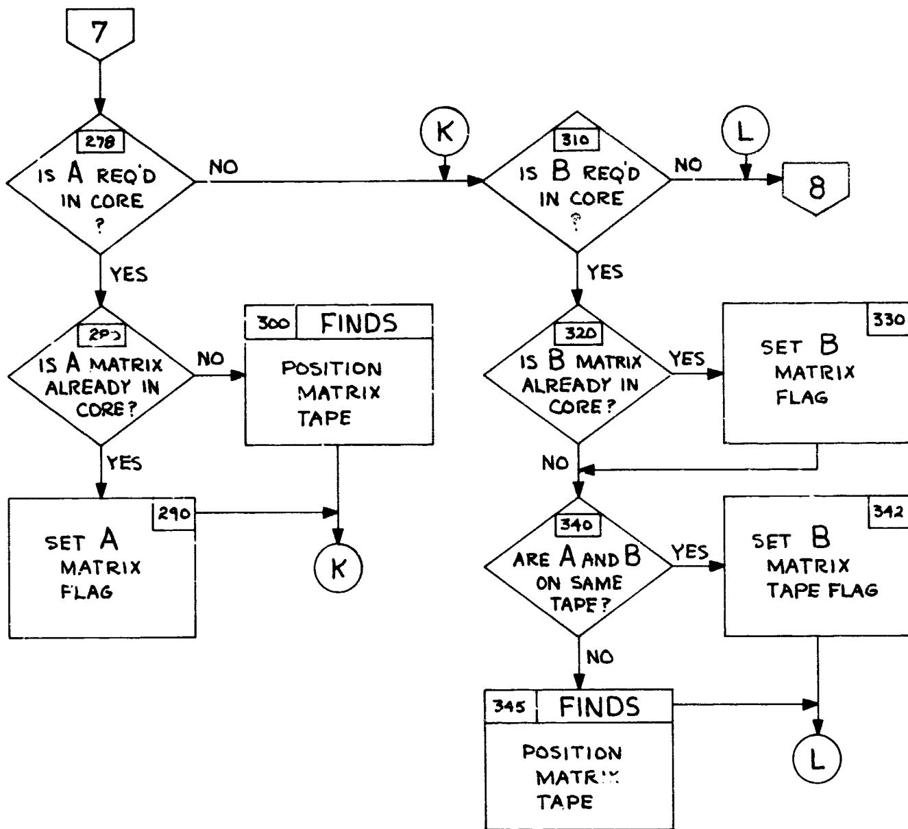
Figure 8-4.5 "MINTS" FLOW
