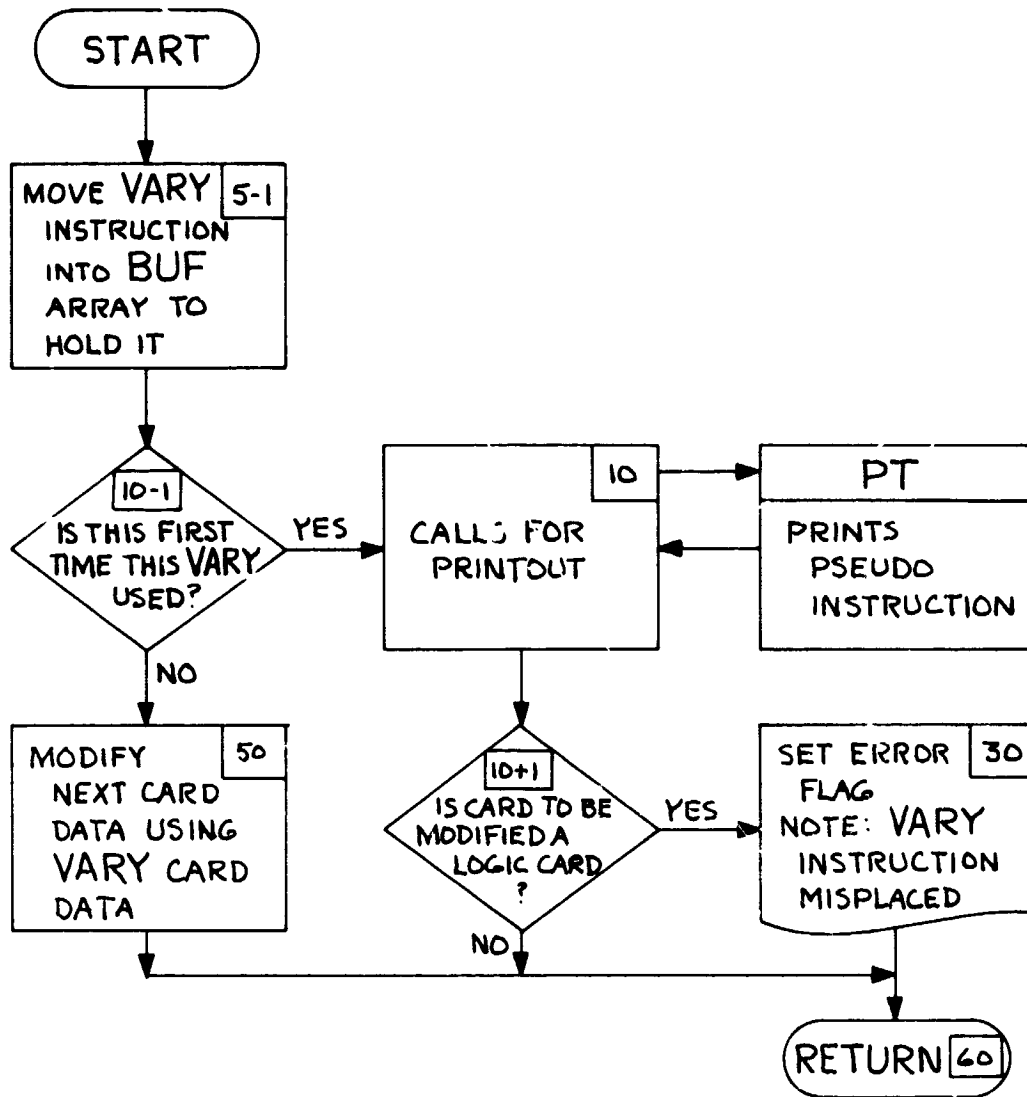
Figure 8-3.5 "VA" FLOW
