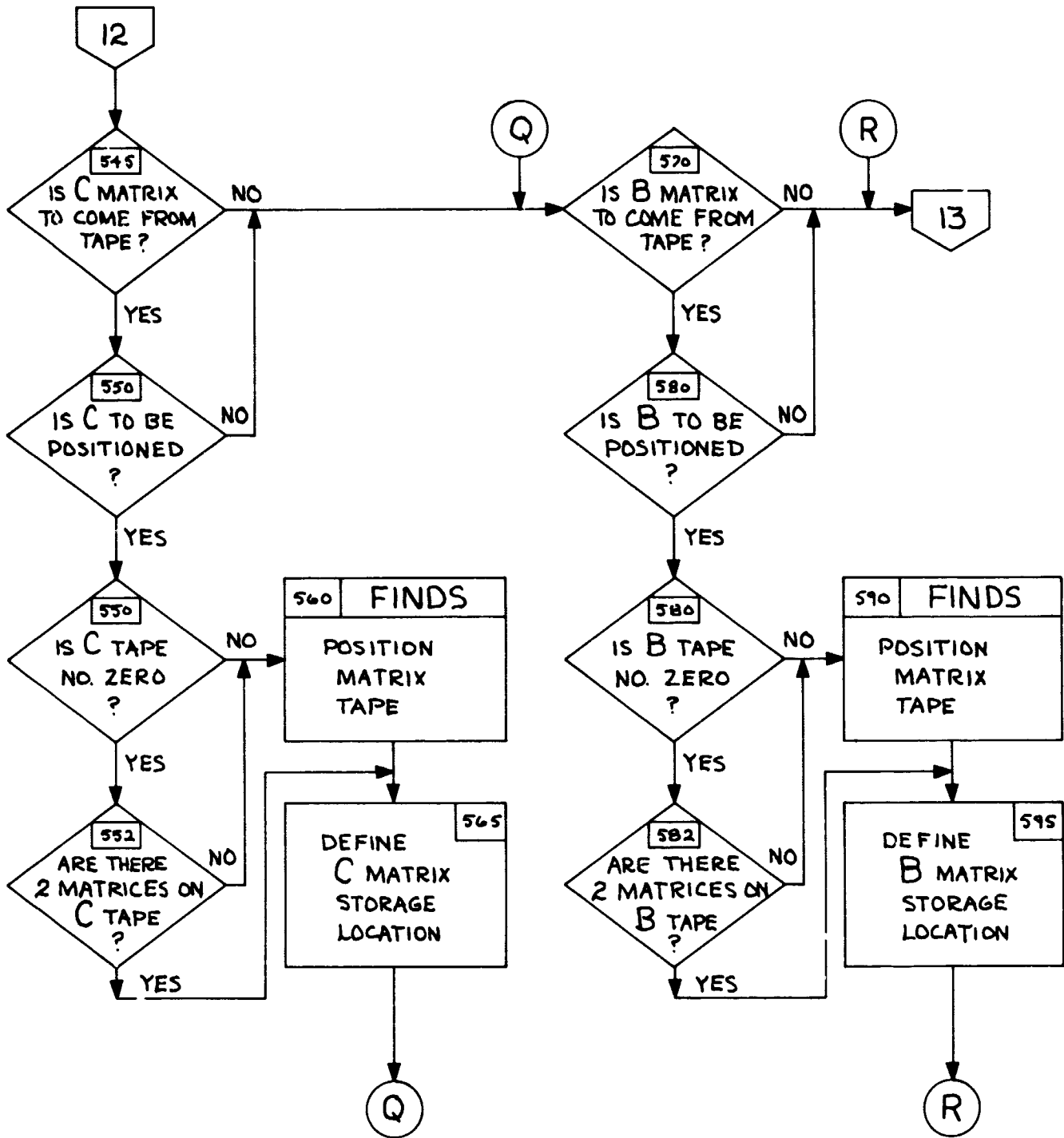
Figure 8-4.5 "MINTS" FLOW
