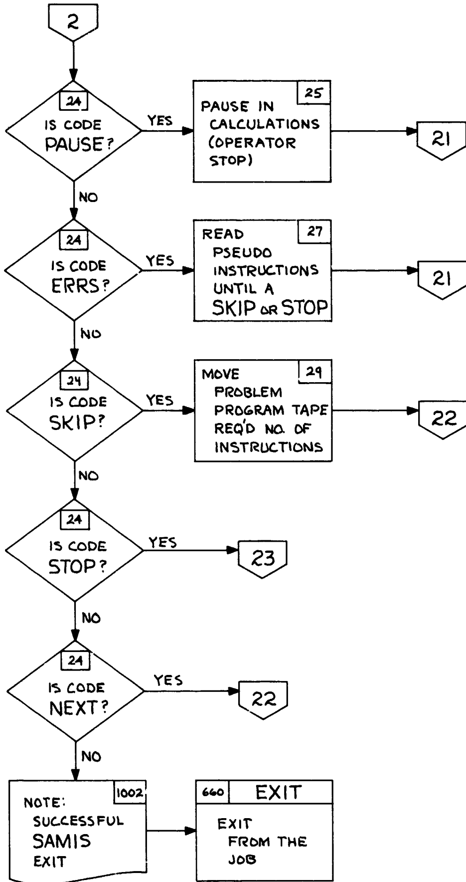
Figure 8-4.: "MINTS" FLOW
