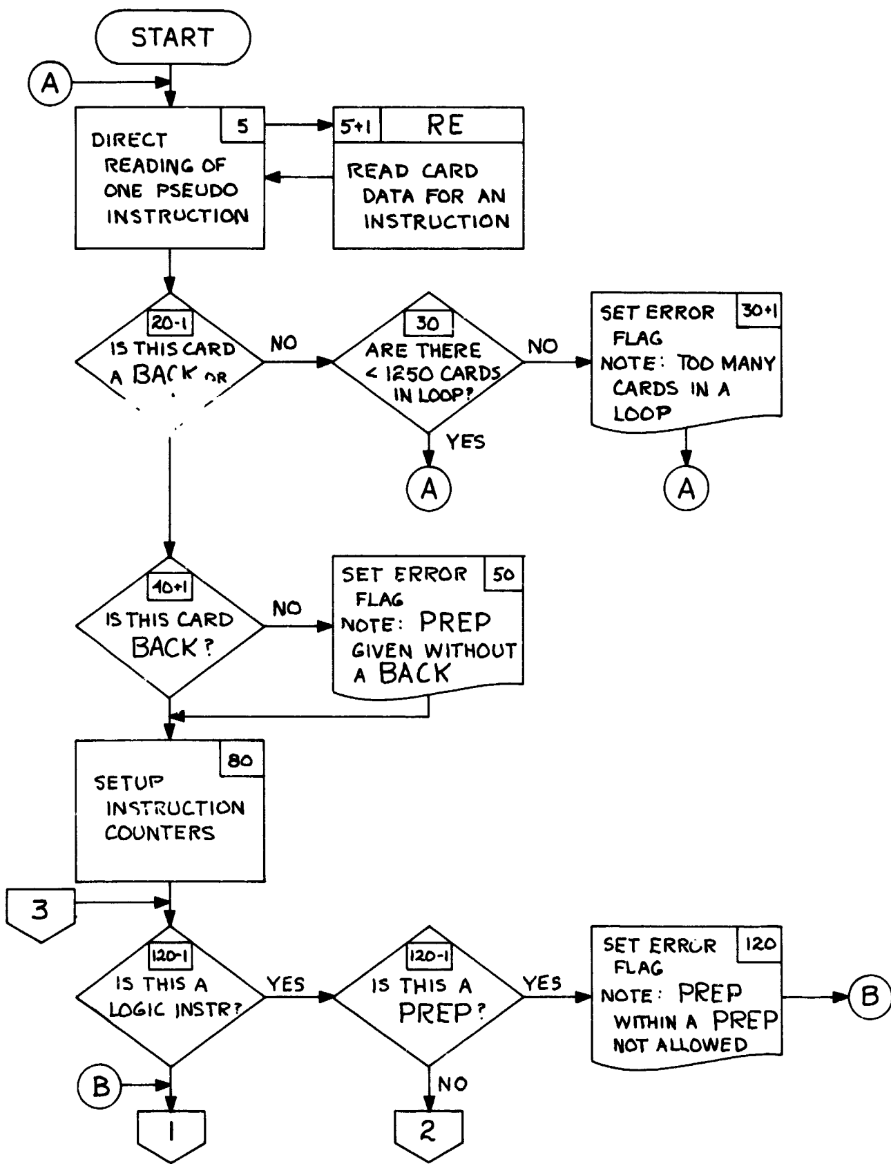
Figure 8-3.4 "PR" FLOW
