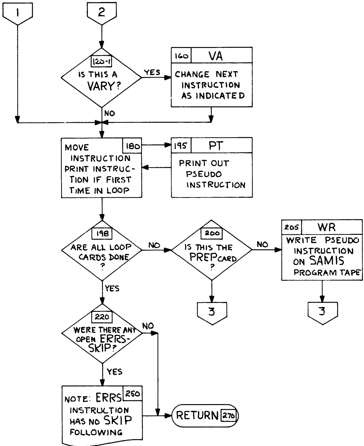
Figure 8-3.4 "PR" FLOW
