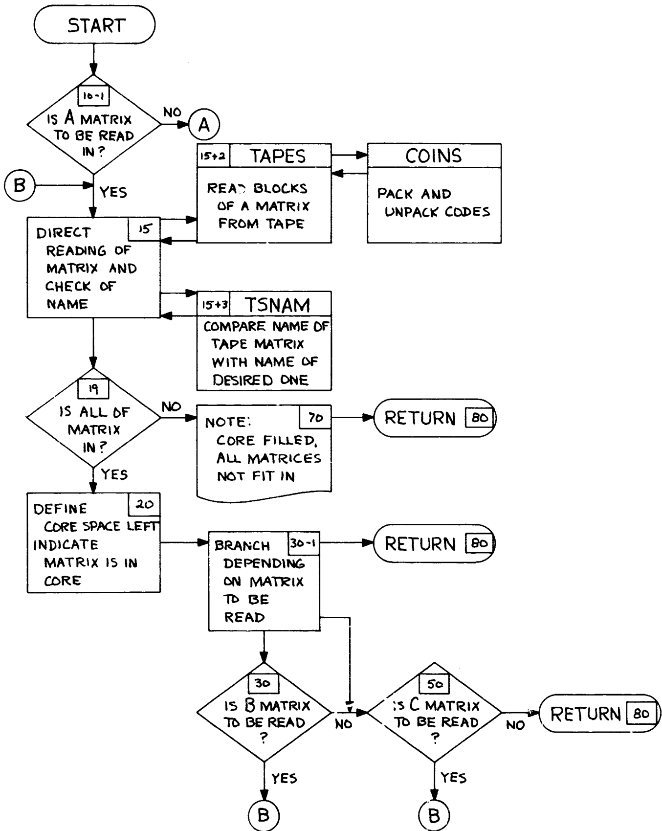
Figure 8-4.2 "IN" FLOW
