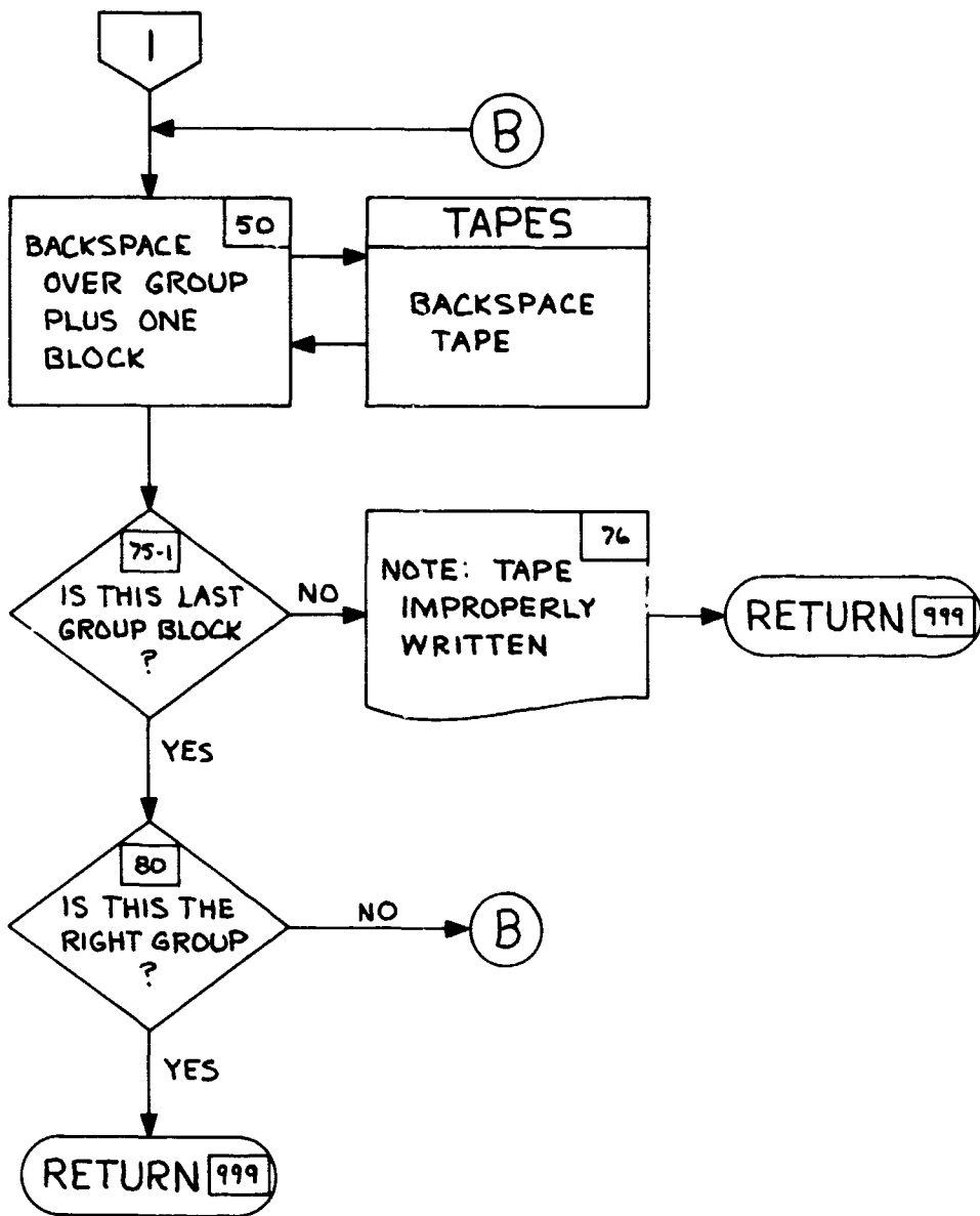
Figure 8-4.4 "FINDS" FLOW
