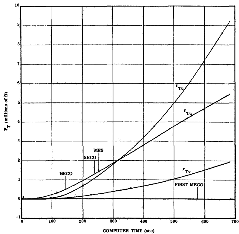
Figure 3-6. Thrust Position, \bar{r}_T
