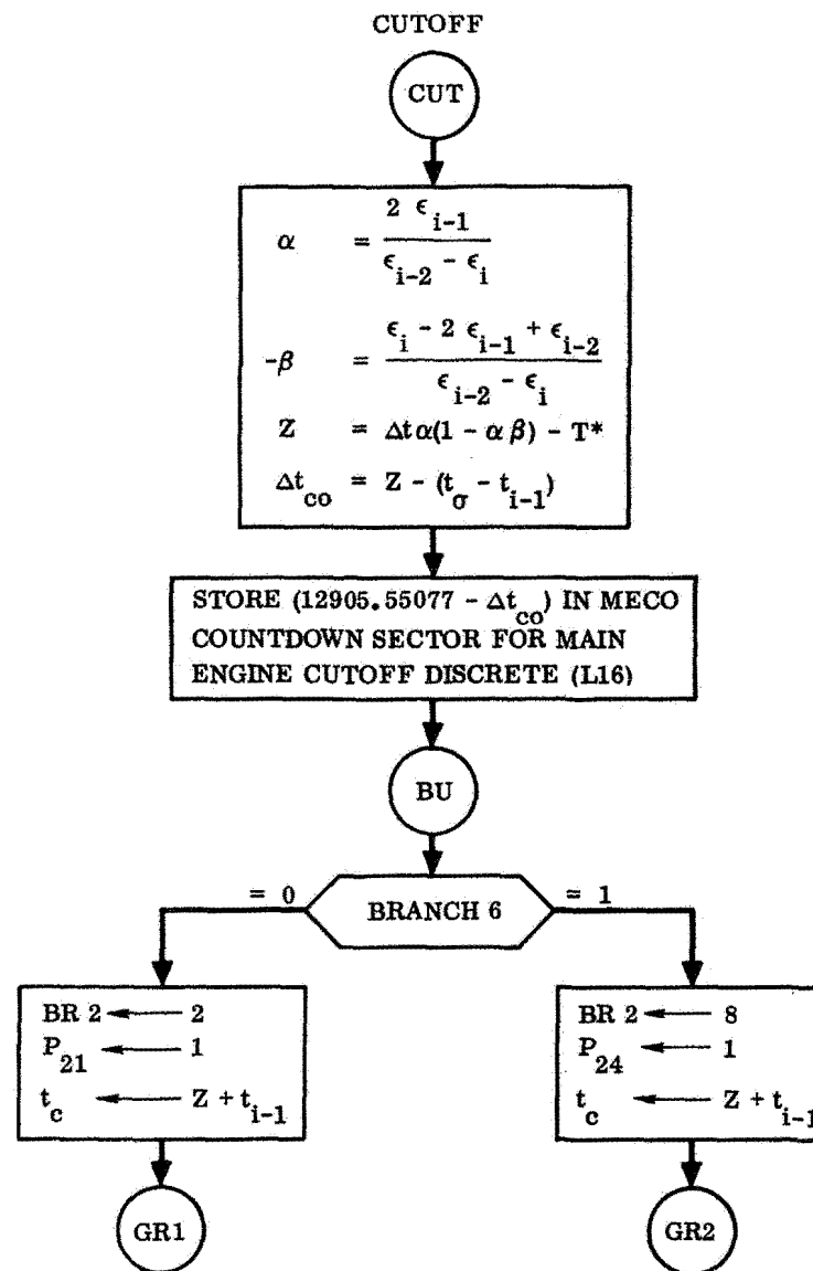
Figure A-9. Centaur Second Burn and Cutoff Extrapolation
