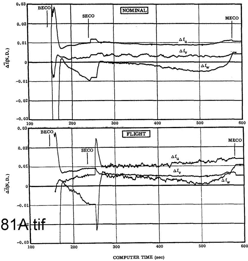
Figure 4-7. Integral Control Term, \Delta f
