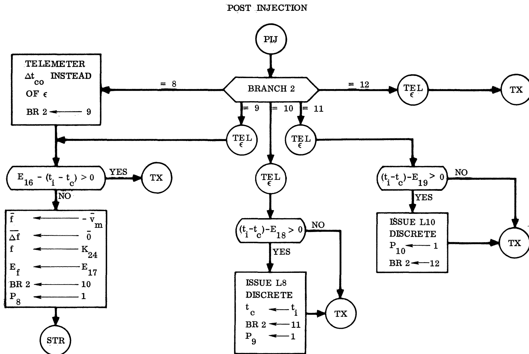
Figure A-10. Post Injection
