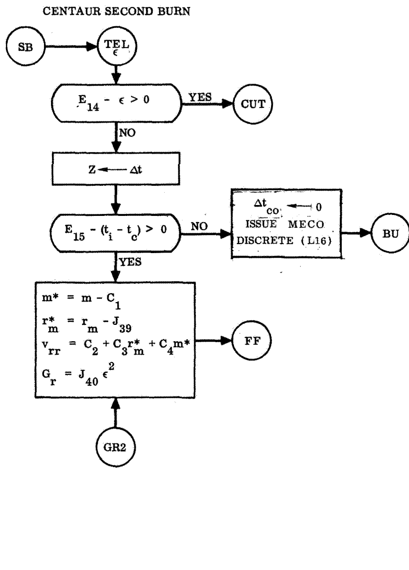
Figure A-9. Centaur Second Burn and Cutoff Extrapolation
