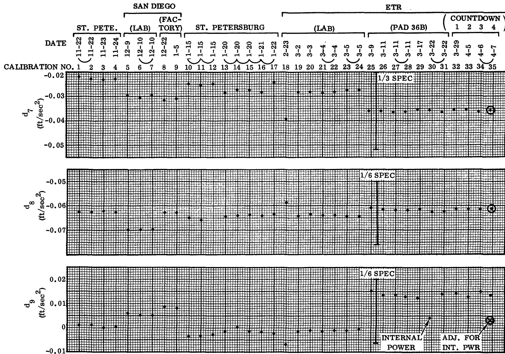
Figure 10-3. Accelerometer Bias
