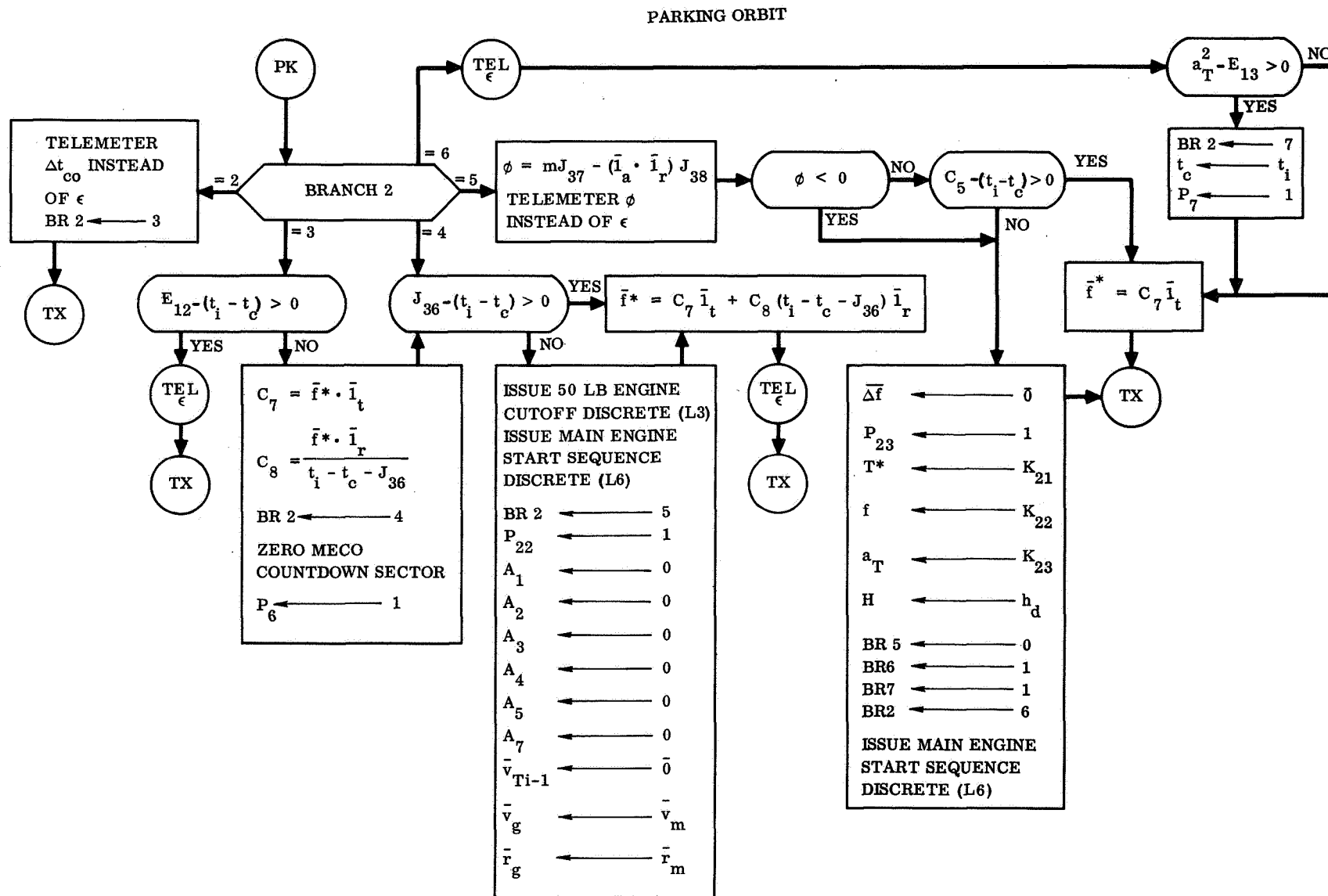
Figure A-8. Parking Orbit
