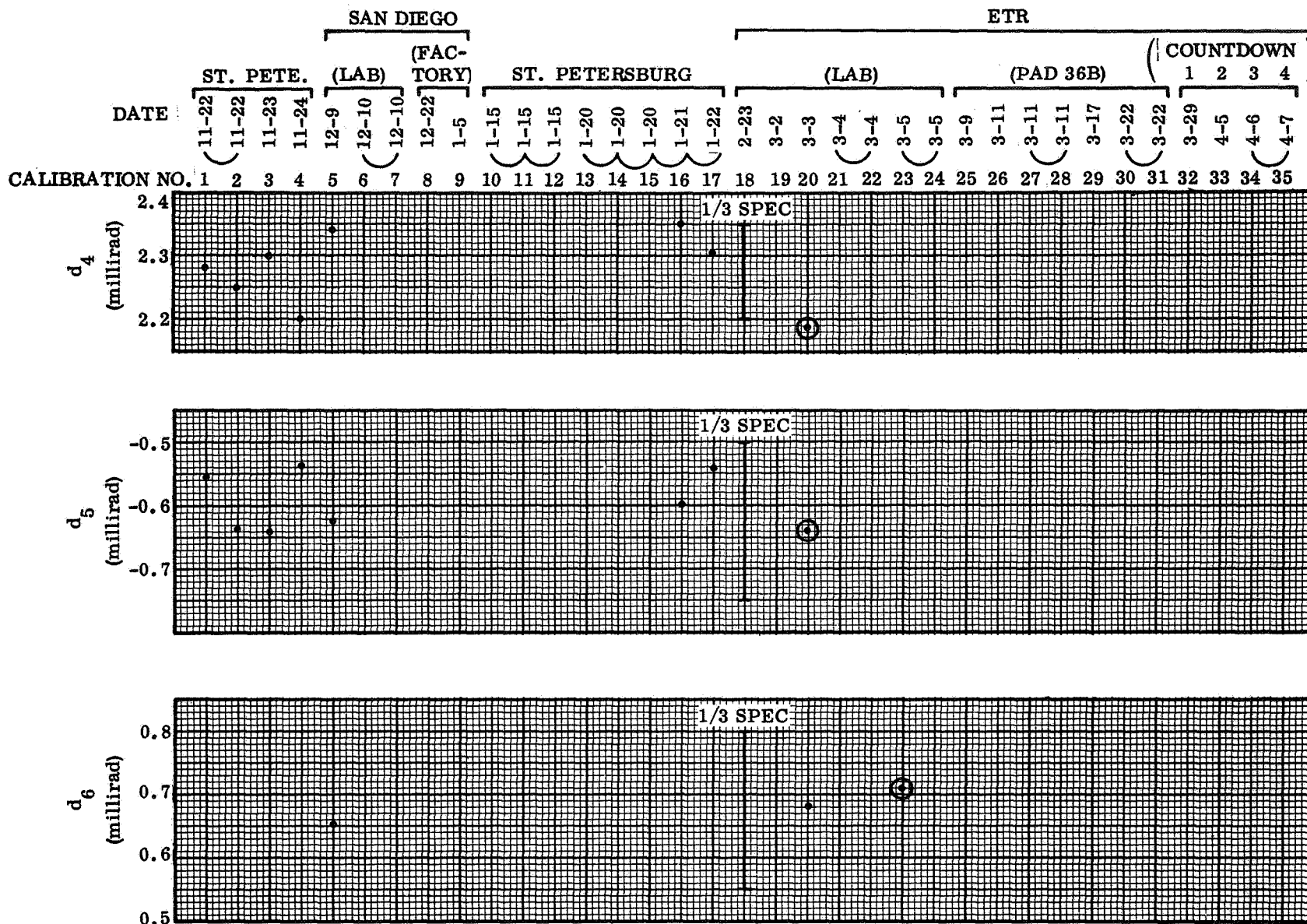
Figure 10-2. Accelerometer Misalignment
