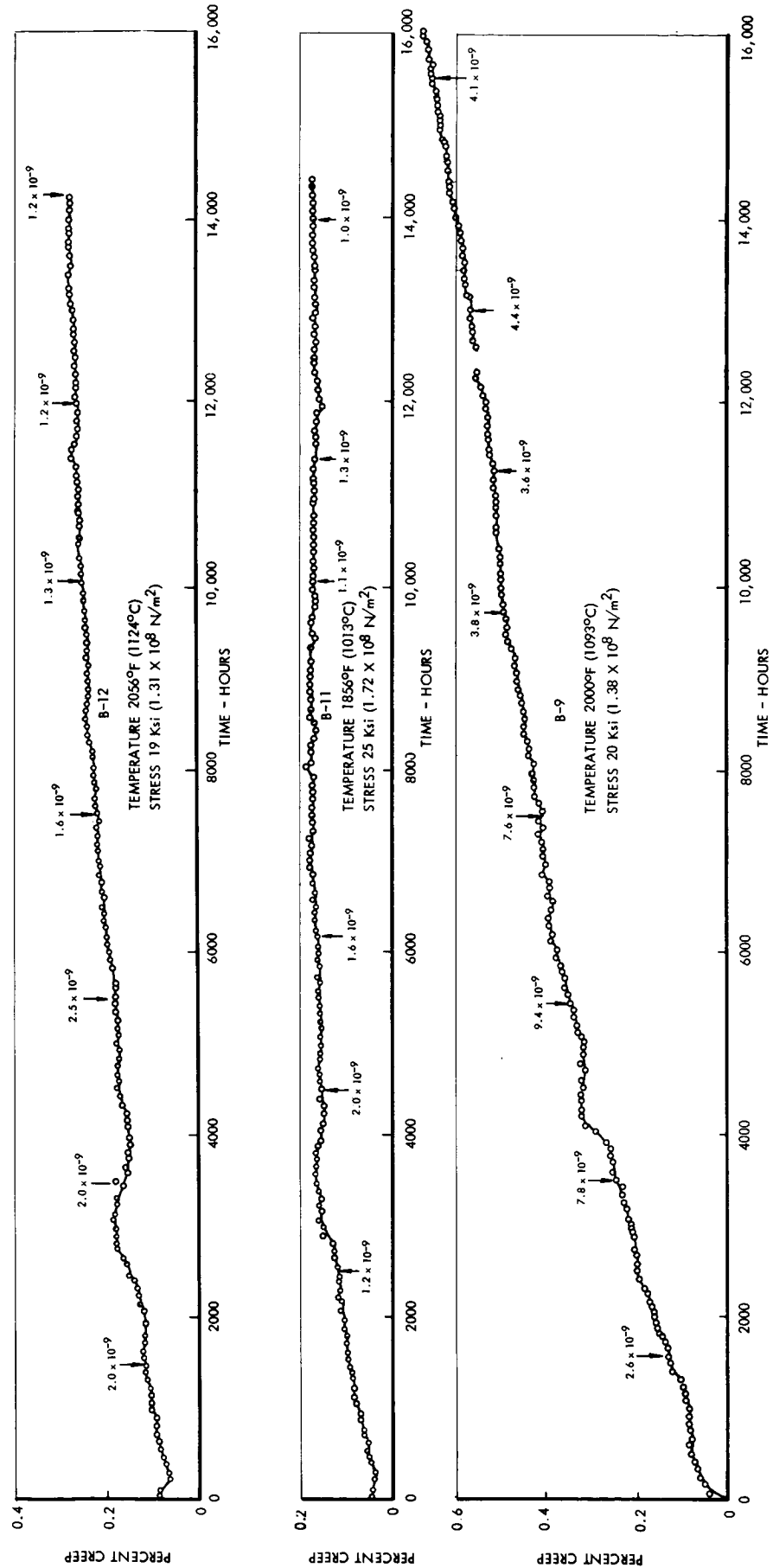
FIGURE 11 CREEP TEST DATA, TZC (HEAT M-80), ANNEALED 3092 F (1700 C), 1 HOUR TESTED IN VACUUM ENVIRONMENT <1 \times 10^{-8} TORR.
