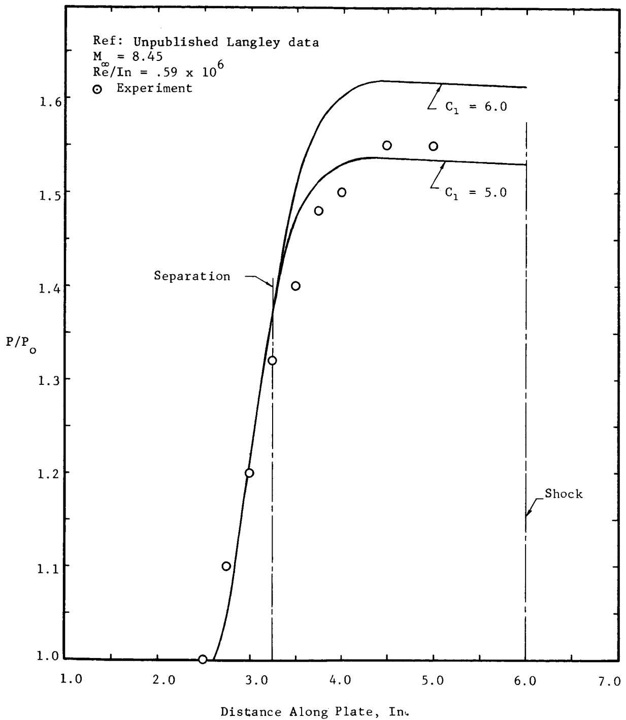
Figure 11. Pressure Correlation at Mach 8.45
