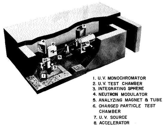
FIGURE 1. MSFC VAN DE GRAAFF FACILITY
