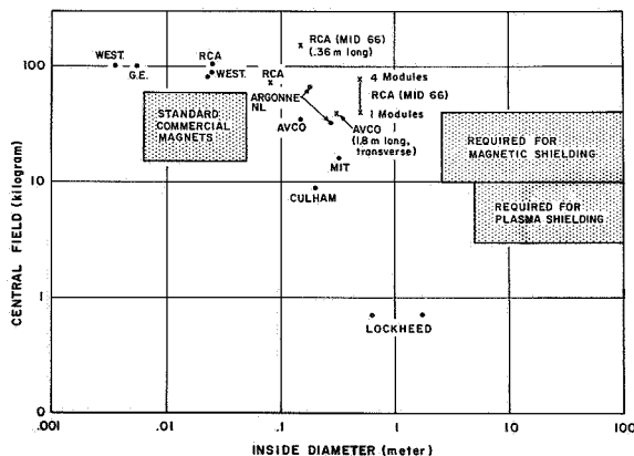
FIGURE 20. SUPERCONDUCTING MAGNETS, JANUARY 1966
