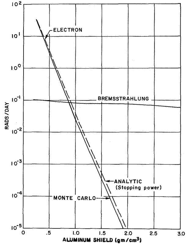
FIGURE 28. SYNCHRONOUS ORBIT ELECTRON DOSE
