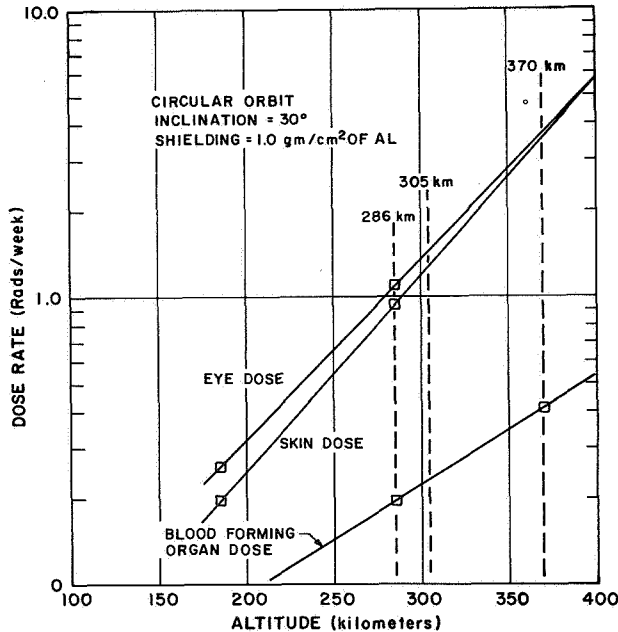
FIGURE 27. SPACE RADIATION DOSE FOR ONE WEEK EXPOSURE IN THE S-IVB HYDROGEN TANK
