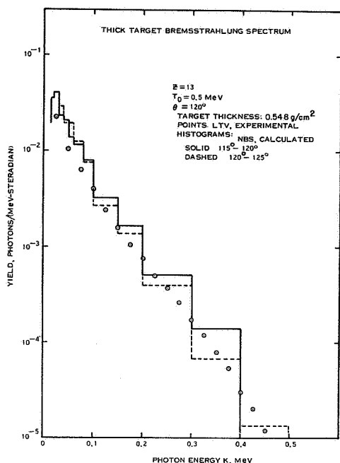
FIGURE 12. THICK TARGET BREMSSTRAHLUNG SPECTRUM
