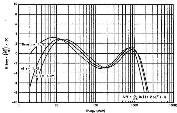
FIGURE 9. PROTON RANGE ERROR CURVE
