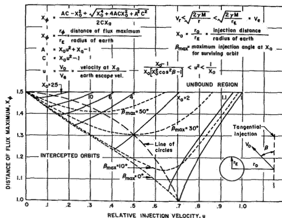
FIGURE 23. RADIAL DISTANCE OF FLUX MAXIMUM FOR BOUNDED PARTICLES
