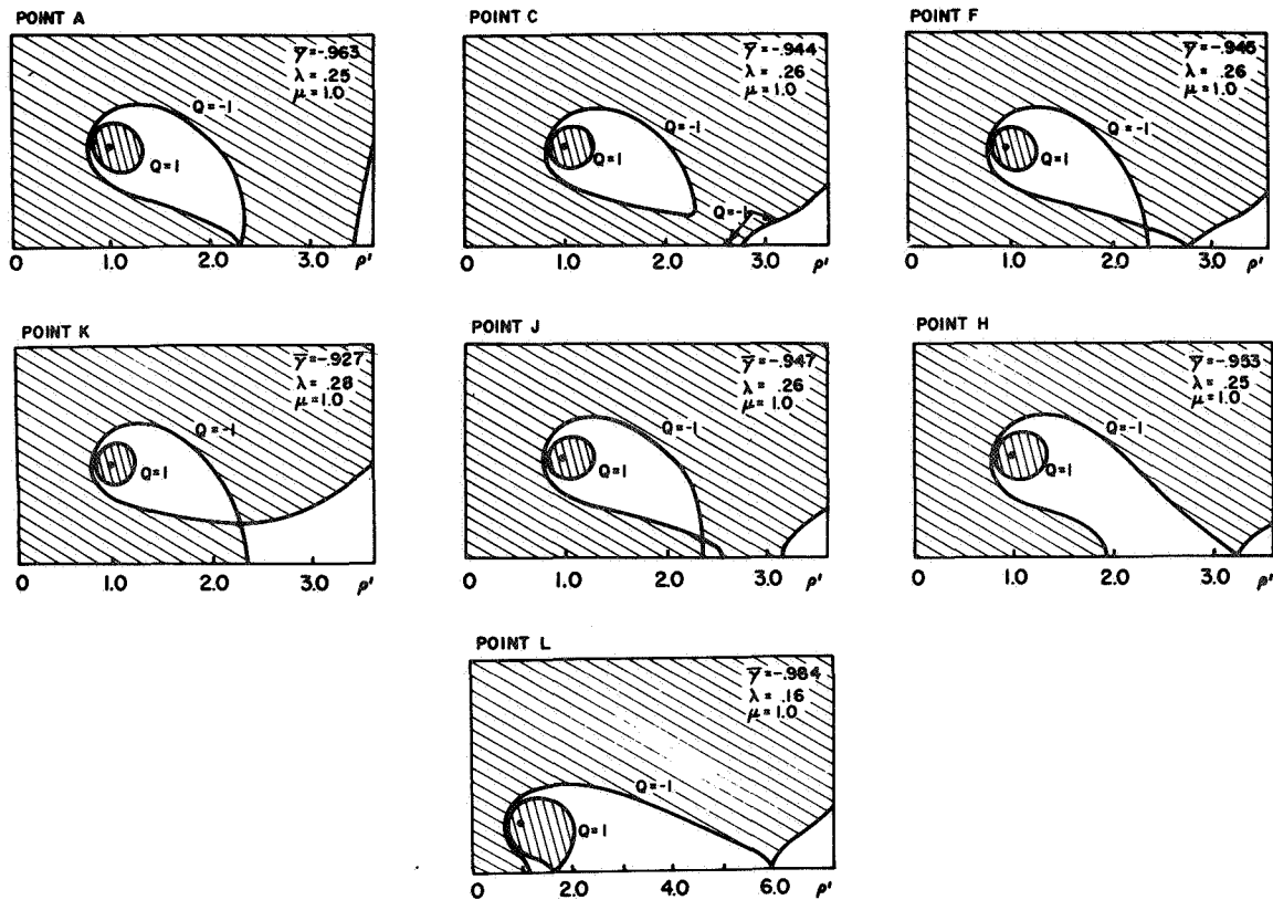
FIGURE 19. CRITICAL POINTS IN THE (\rho, \theta) PLANE OF A DOUBLE-PARALLEL LOOP SYSTEM
