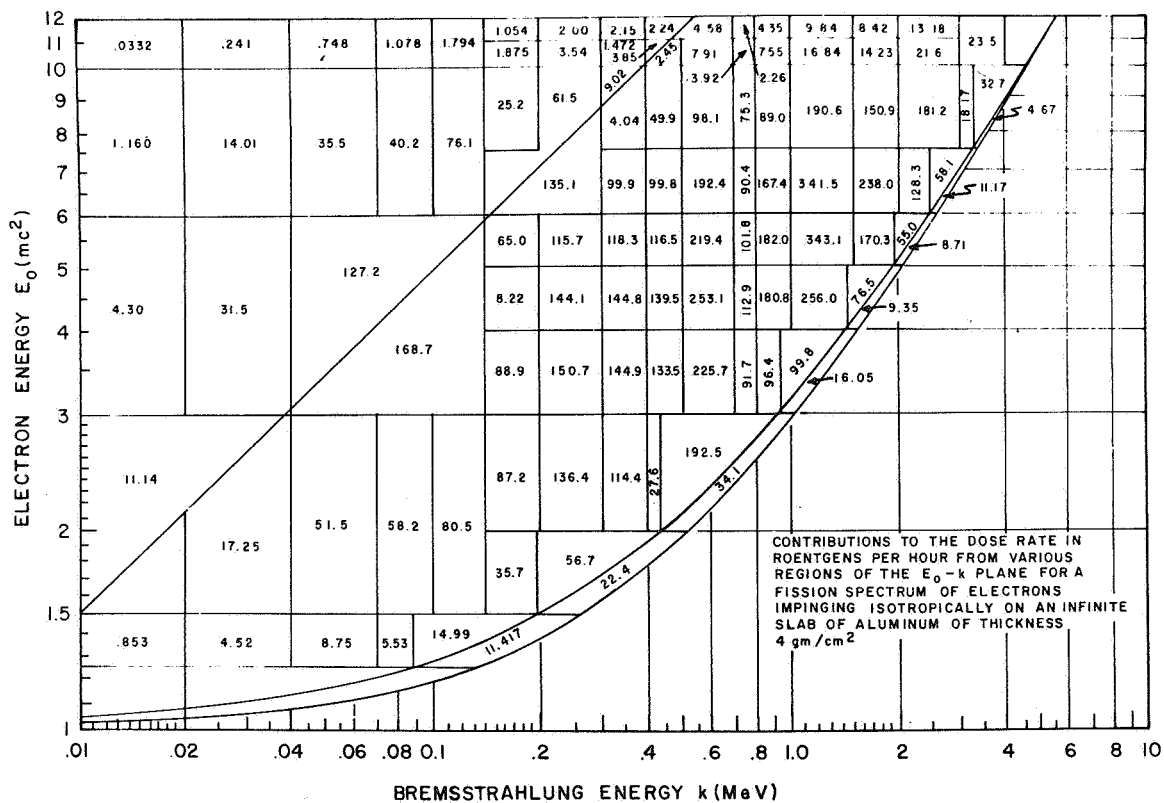
FIGURE 14. ERRORS IN BREMSSTRAHLUNG DOSE CALCULATION DUE TO INACCURACIES IN INPUT CROSS SECTION DATA
