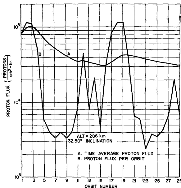
FIGURE 15. PROTON FLUX CURVES FOR EARTH ORBITS
