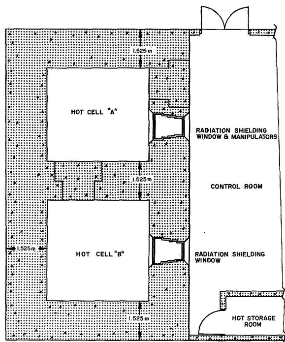
FIGURE 3. SCHEMATIC OF ASTRIONICS LABORATORY'S HOT CELL RADIATION FACILITY
