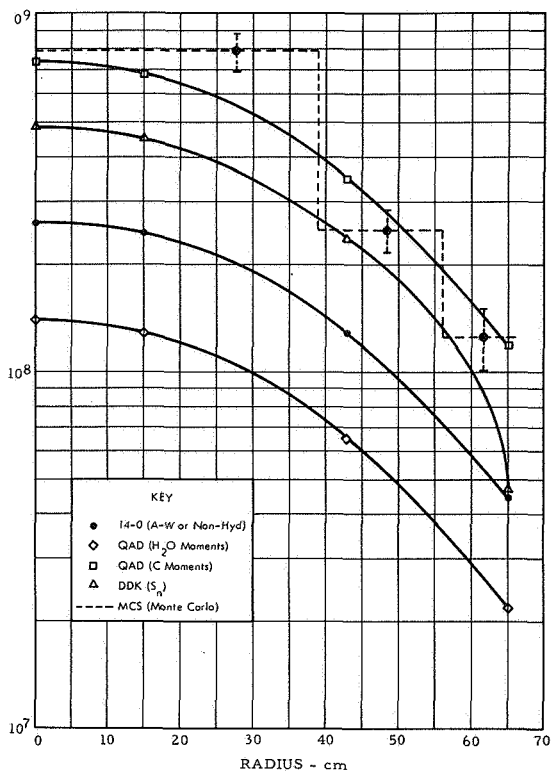
FIGURE 17. NEUTRON DOSE RATE TRAVERSE USING DIFFERENT CALCULATION METHODS
