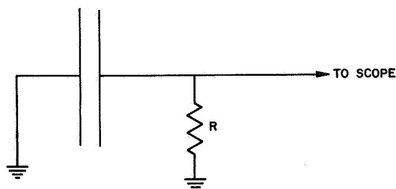
FIGURE 26. PEGASUS OSCILLOSCOPE CIRCUITS
