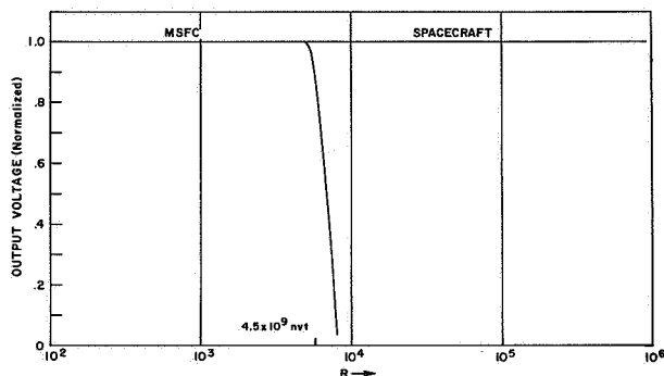
FIGURE 6. PERFORMANCE OF IRRADIATED UNHARDENED POWER SUPPLY
