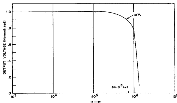
FIGURE 7. PERFORMANCE OF IRRADIATED HIGH-VOLTAGE POWER SUPPLY MODIFIED FOR RADIATION ENVIRONMENT
