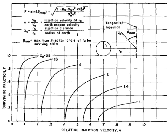
FIGURE 24. FRACTION OF PARTICLES IN SURVIVING ORBITS TO TOTAL PARTICLES INJECTED ISOTROPICALLY AT r_0
