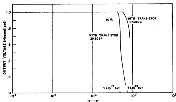
FIGURE 8. PERFORMANCE OF IRRADIATED SERVOAMPLIFIERS WITH SPECIAL DESIGN FOR RADIATION ENVIRONMENT
