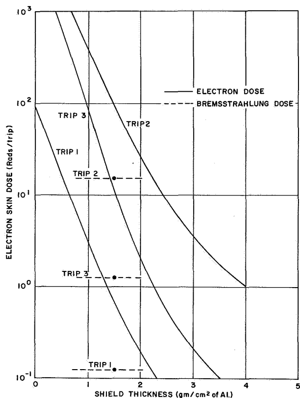
FIGURE 29. ELECTRON AND BREMSSTRAHLUNG DOSE CURVES
