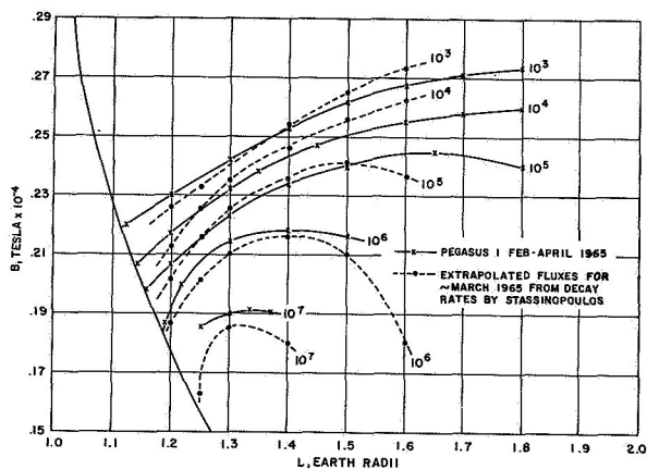
FIGURE 31. PEGASUS ISOFLUX CONTOURS FOR ELECTRONS
