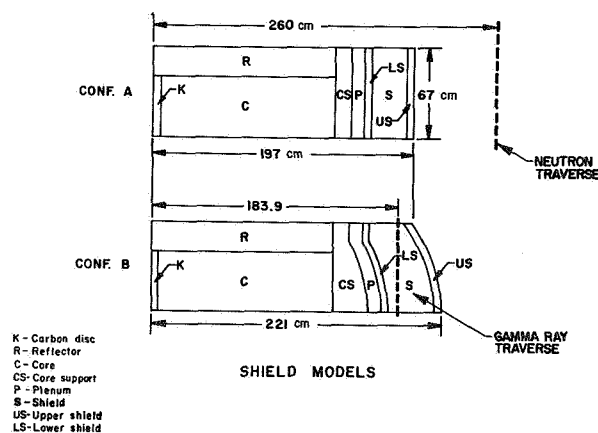
FIGURE 16. RADIATION SHIELD MODELS USED IN COMPUTING NUCLEAR ROCKET RADIATION FIELDS
