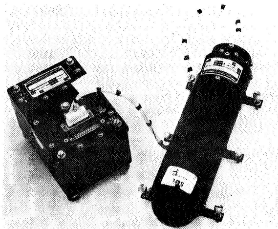
FIGURE 30. PEGASUS ELECTRON SPECTROMETER
