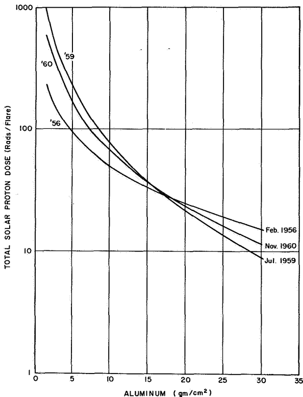
FIGURE 10. ACCUMULATIVE DOSE THROUGH VARIED THICKNESSES OF ALUMINUM FROM SOLAR PROTONS AND COSMIC RAYS
