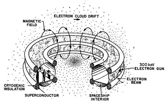
FIGURE 21. SCHEMATIC DIAGRAM OF A SPACE VEHICLE USING A PLASMA RADIATION SHIELD
