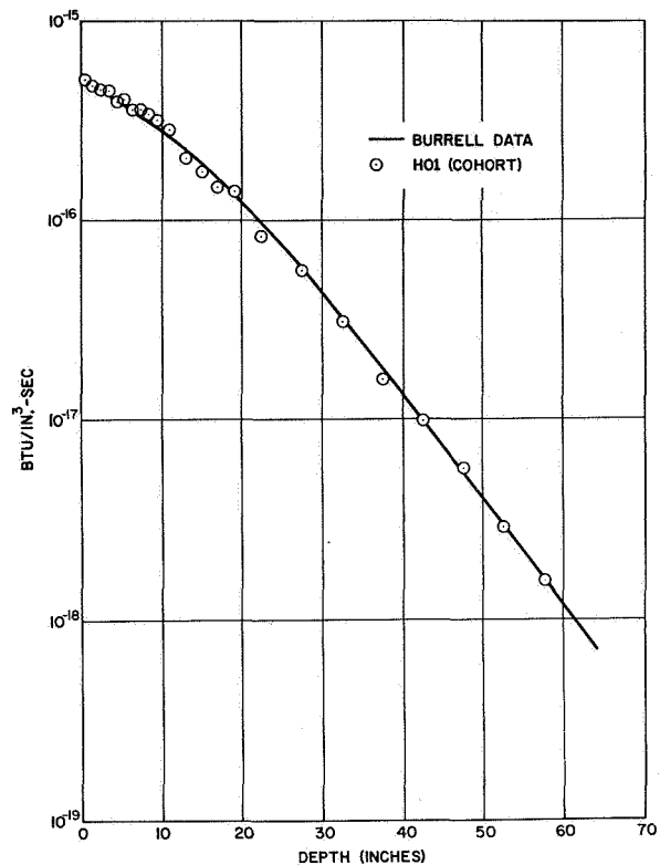
FIGURE 18. HEAT DEPOSITION VERSUS DEPTH FOR 7 MeV NEUTRONS IN A LIQUID HYDROGEN SLAB
