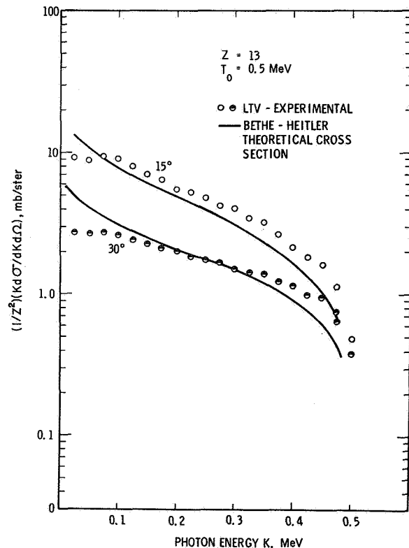
FIGURE 11. THIN TARGET DIFFERENTIAL CROSS SECTIONS
