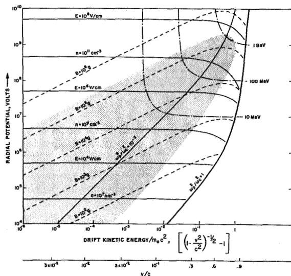
FIGURE 22. MAP OF ONE-METER ELECTRON PLASMA CONTAINMENT DEVICE
