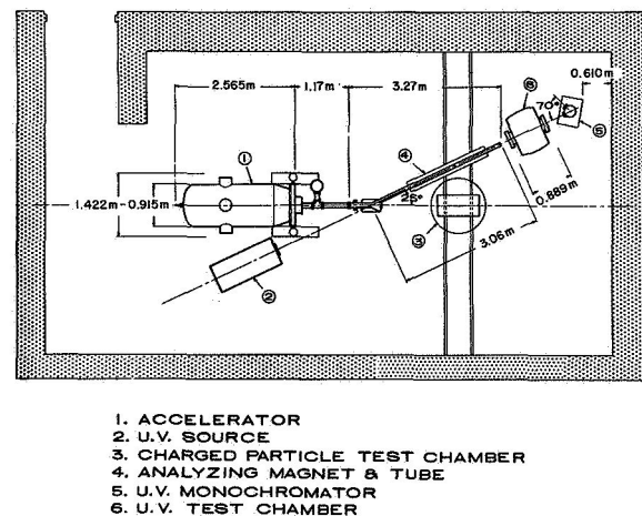
FIGURE 2. SCHEMATIC OF VAN DE GRAAFF FACILITY
