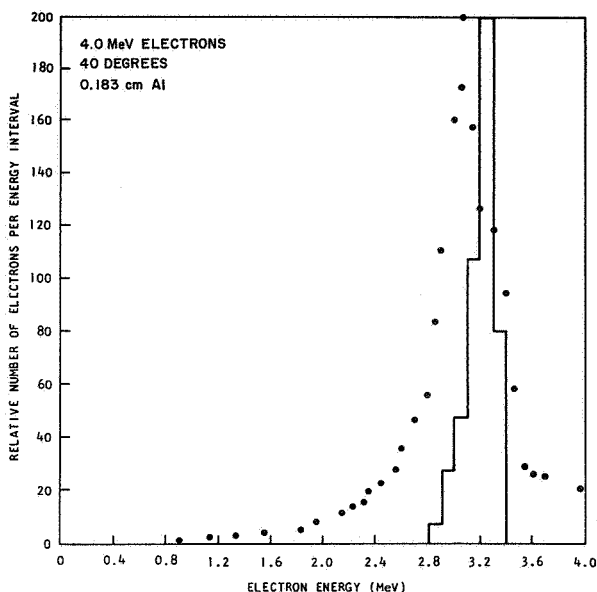
FIGURE 13. ELECTRON ENERGY SPECTRUM AT FORTY DEGREES FOR A 0.183-CM THICK ALUMINUM SLAB TARGET
