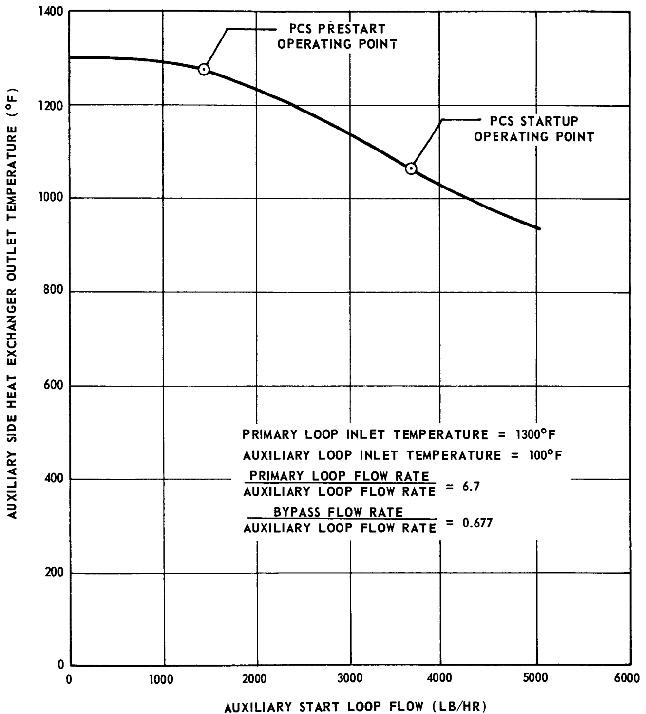
PCS Start Performance - Heat Exchanger Outlet Temperature
