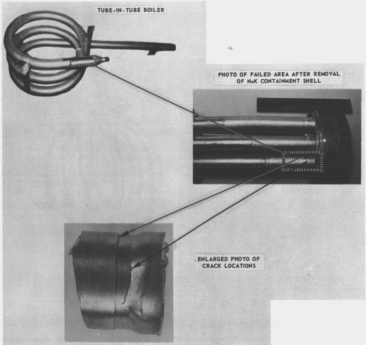
Tube-in-Tube Boiler Failure (P/N 097444-7, S/N A-2)
