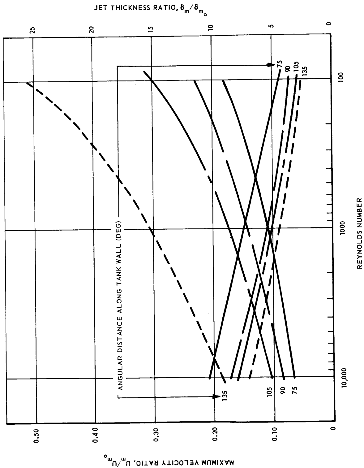
Fig. II-19 Effect of Jet Reynolds Number on Wall-Bound Jet Degradation (Radius Ratio, R/\delta m_o = 300 )
