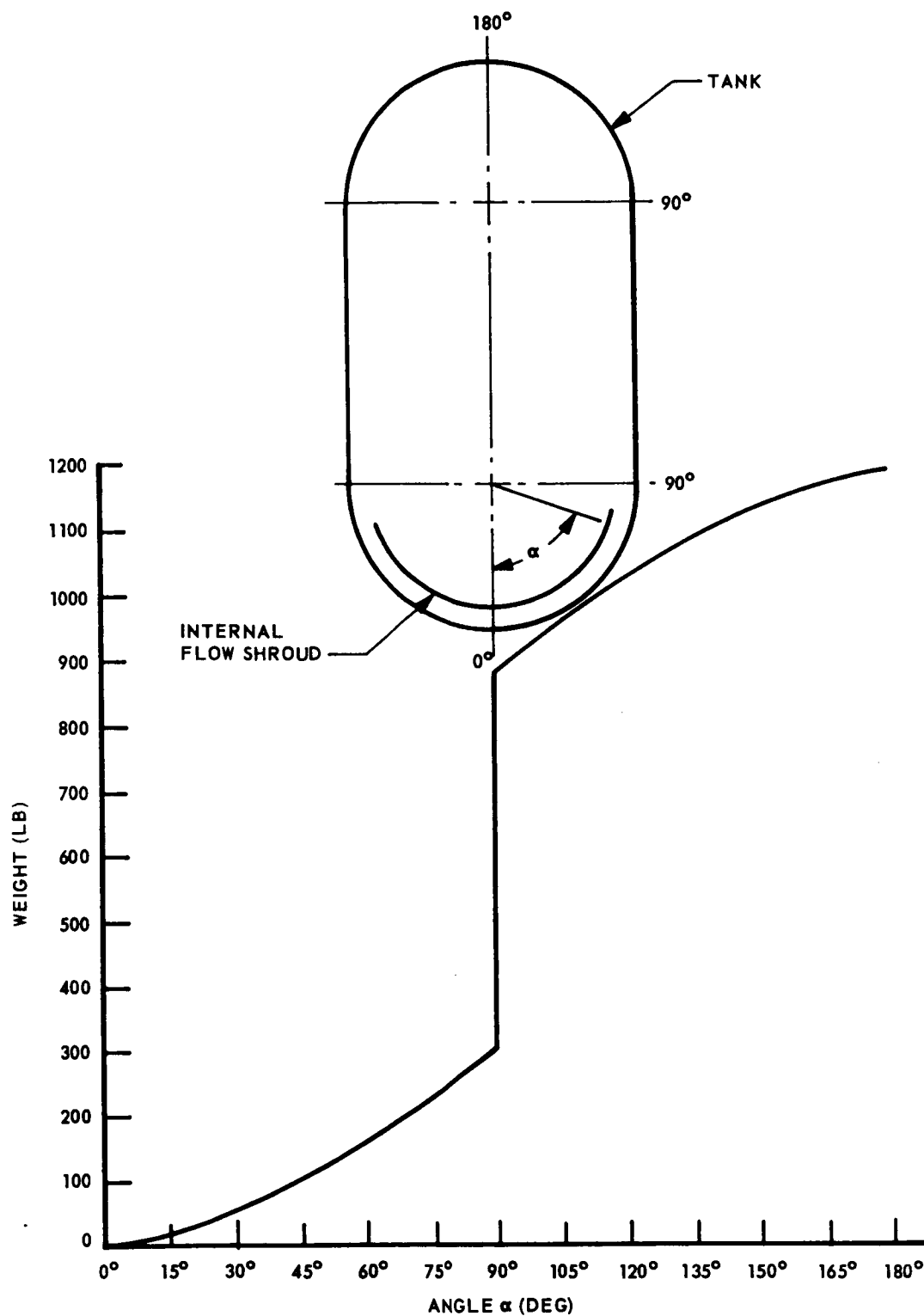
Fig. I-45 Internal Shroud Weight - Mission (3) Vehicle
