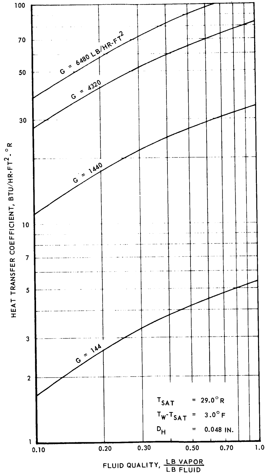
Fig. I-20 Heat Transfer Coefficients for Mist Flow
