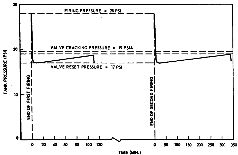
Fig. VI-14a Tank Pressure History for Mission (2) Vehicle (Stratified Model)
