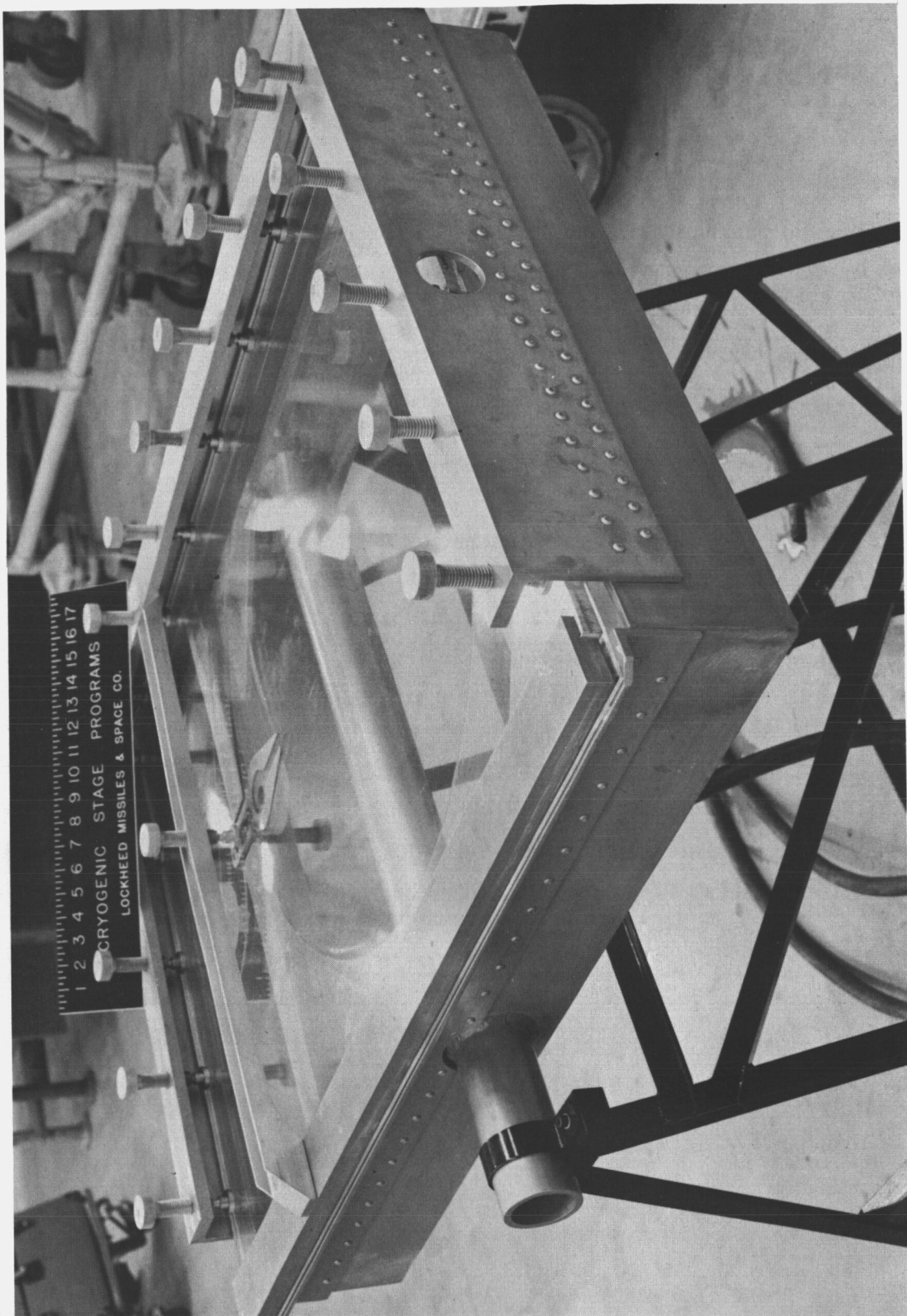
Fig. H-1 Two-Dimensional Flow Test Apparatus
