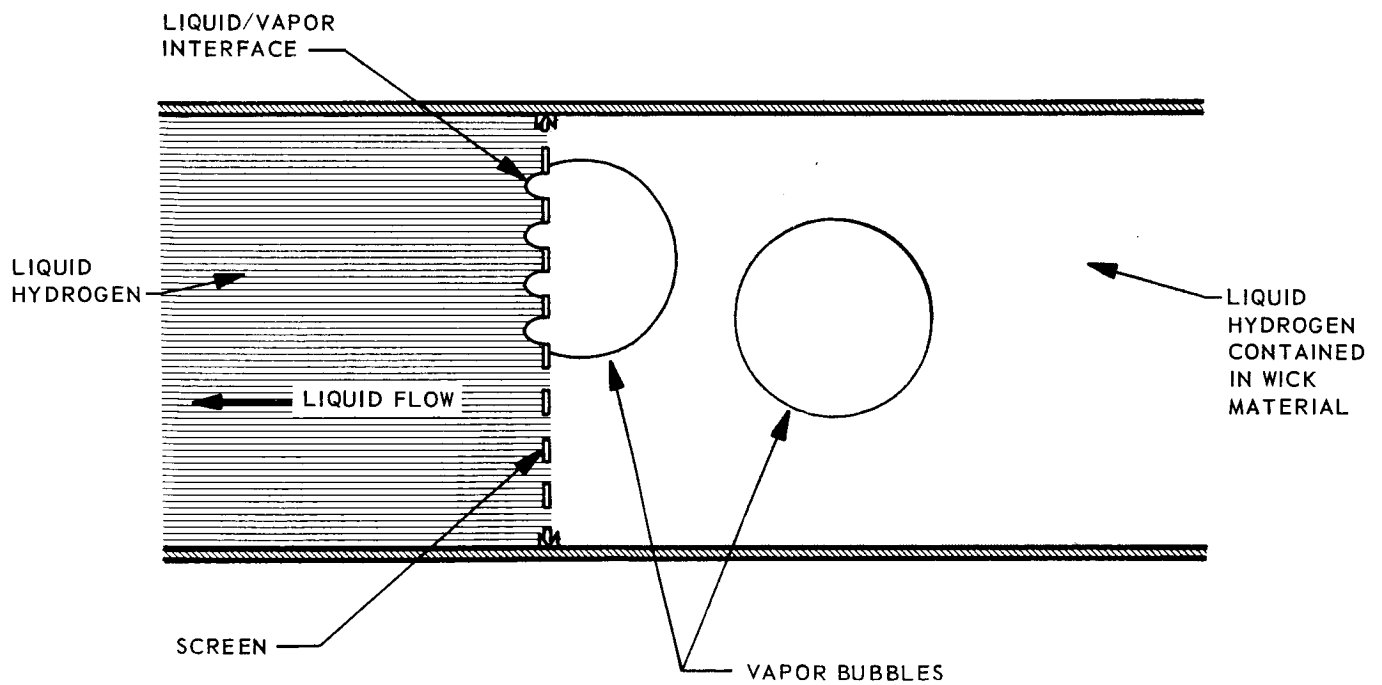
Fig. I-4 Principle of Operation of Wick Device
