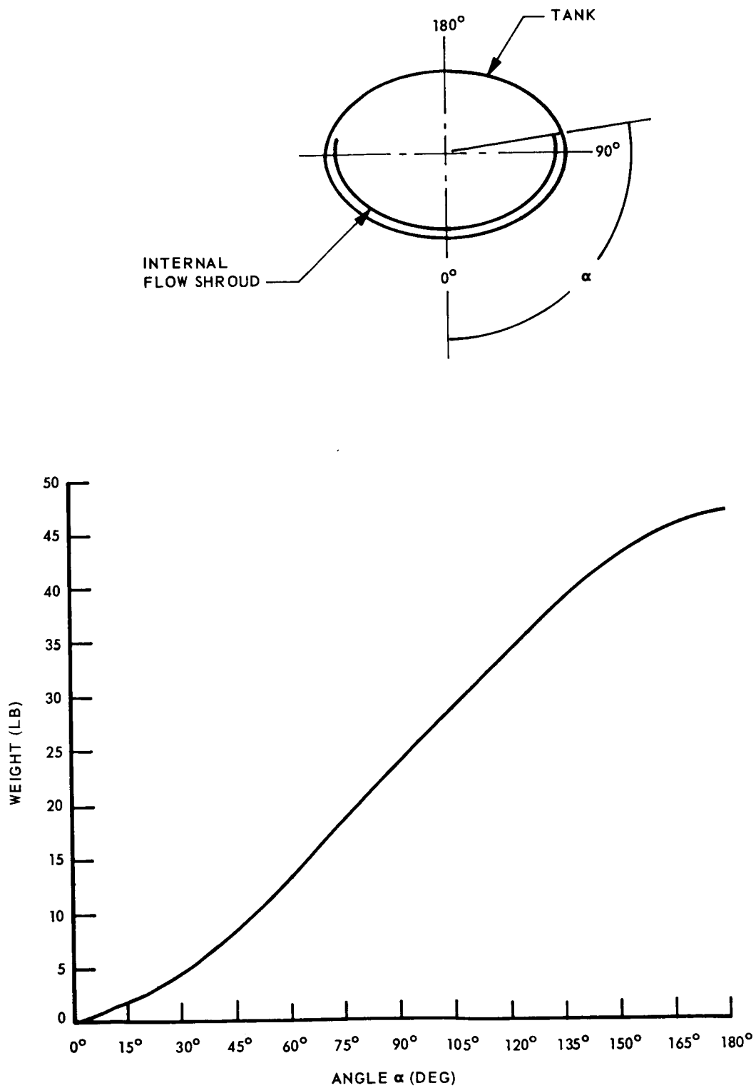
Fig. I-44 Internal Shroud Weight — Mission (2) Vehicle
