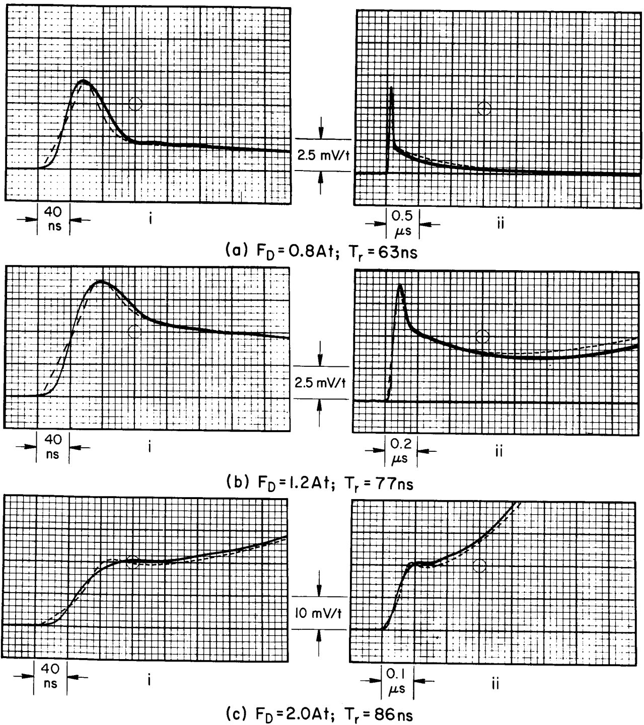
FIG. 9 EXPERIMENTAL (Solid Line) AND COMPUTED (Dashed Line) \dot{\phi}(t) WAVEFORMS OF UNLOADED CORE E-6 DURING THE BEGINNING OF SWITCHING, USING F(t) WITH T_r \approx 65\text{ ns} AND VARIOUS VALUES OF AMPLITUDE F_D
