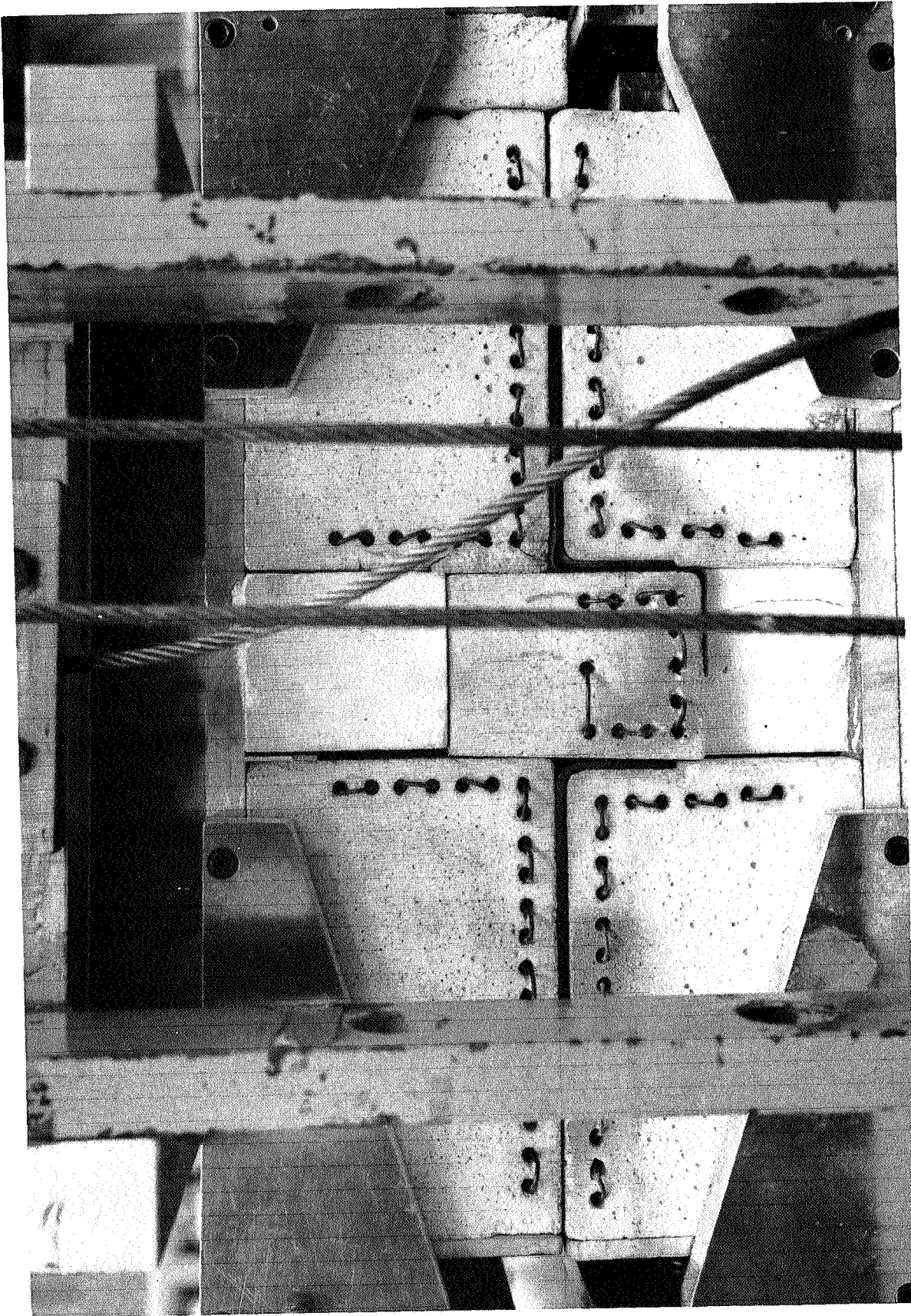
Figure 18 Zee Section Being Relieved in the Universal Forming Die. Note the stainless steel buffer plates and the 1 1/2-degree springback allowance on the left side of the punch block.
