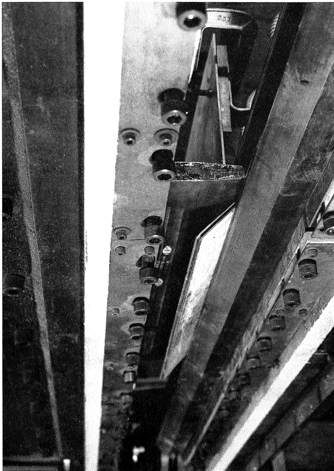
Figure 16 Channel Being Formed on the Press Brake Note the steel plates on both sides of the beryllium specimen.
