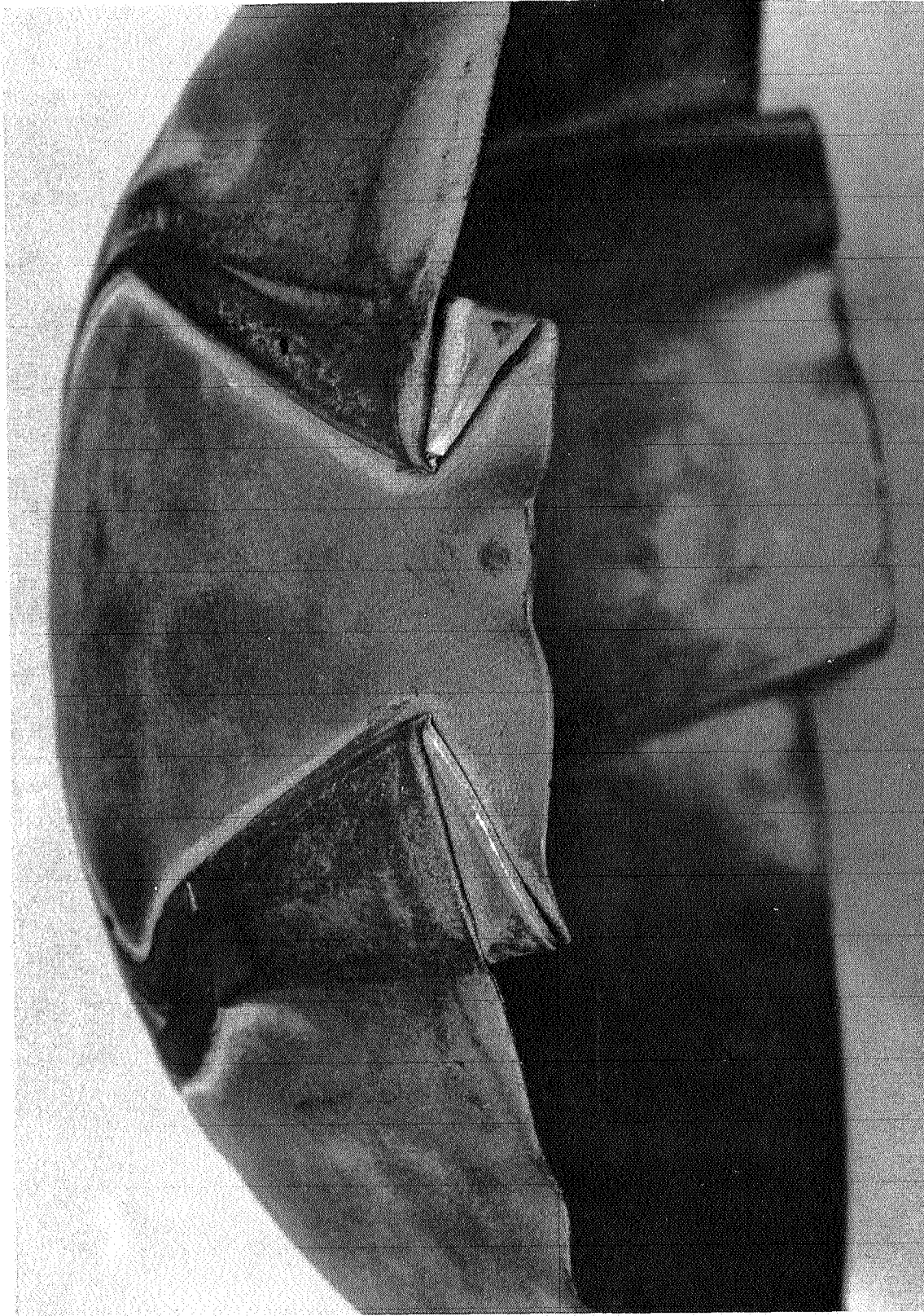
Figure 33 Experimental Hemispherical Segment - .020" Material. Note severe folding of the material.
