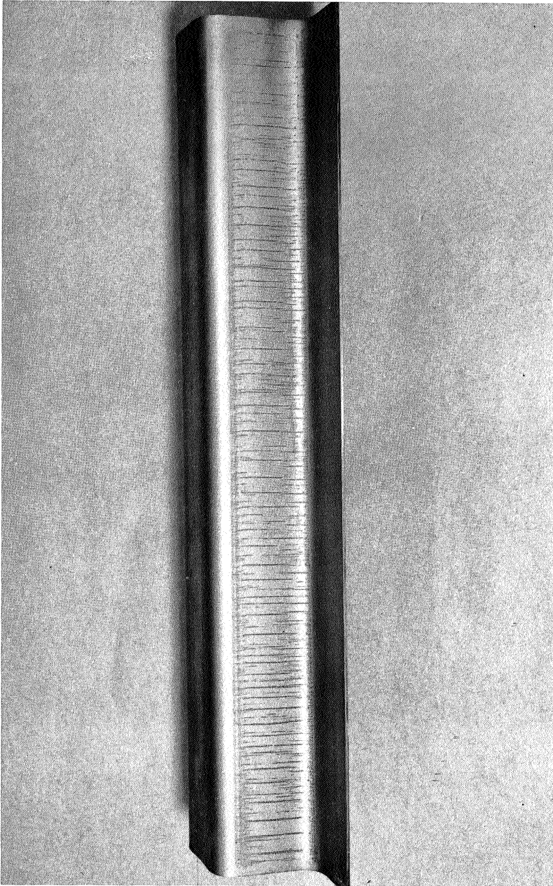
Figure 20 Hat Section formed in the Universal Forming Die without Buffer Strips or Lubricant. Note the severe galling.
