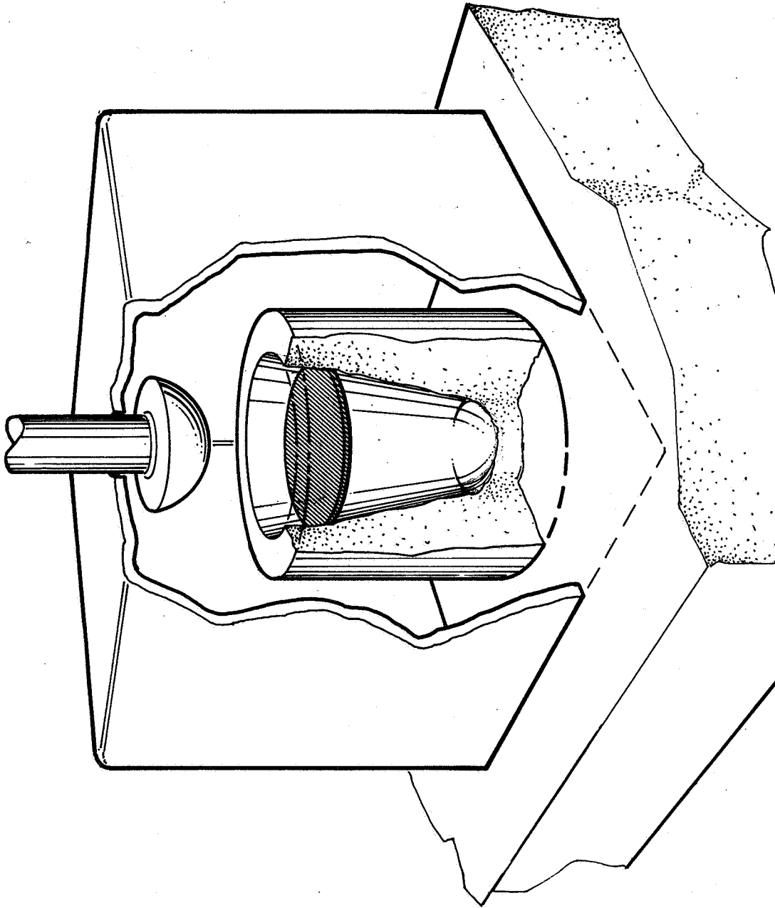
Figure 31 Experimental Punch and Die - Preliminary Spherical Radius Forming - 3.0" Radius
