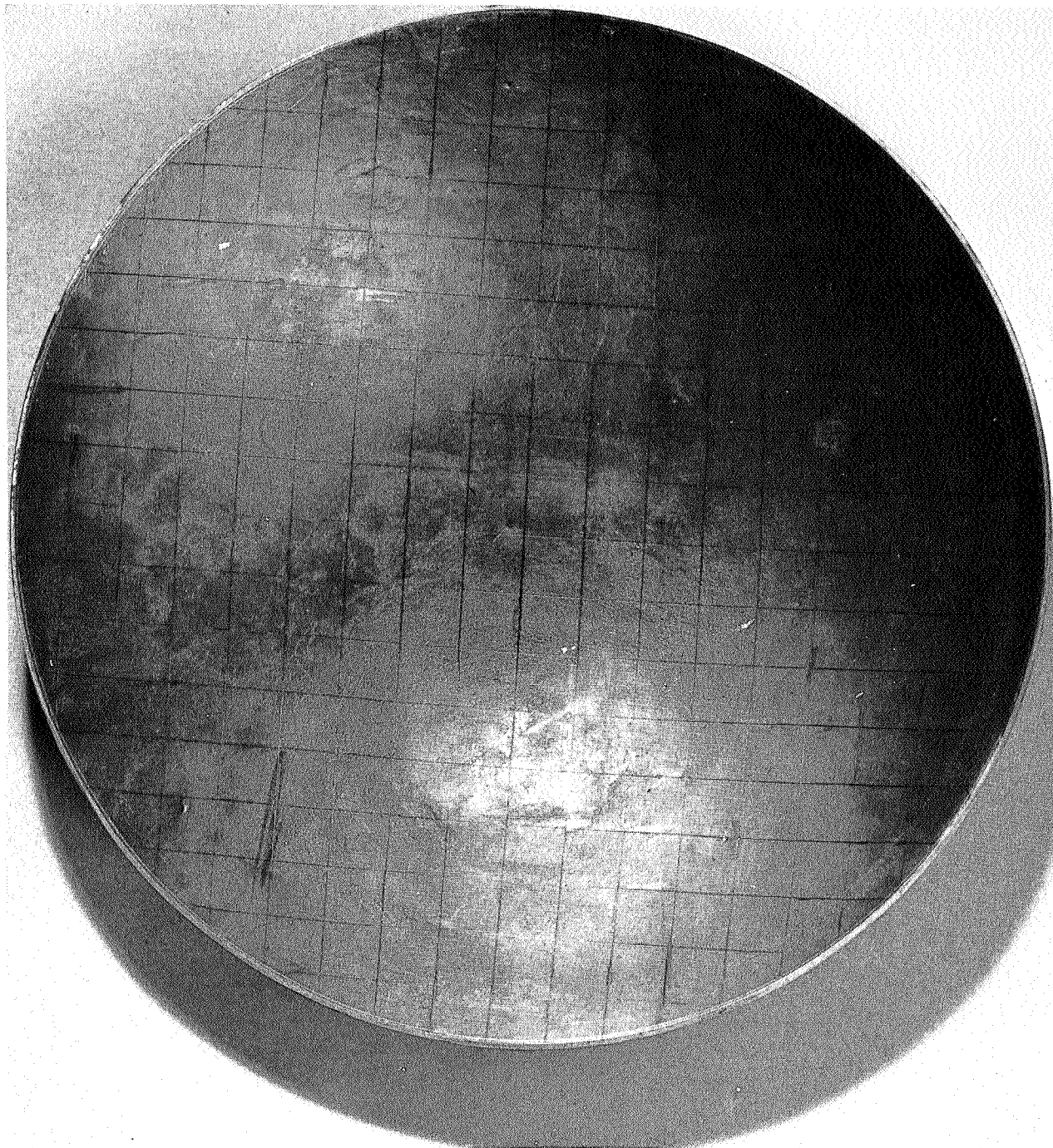
Figure 37 Scribed Inner Surface of the Formed Spherical Segment - 1.00" Grid - .120" Material - 12.0 Radius - 100 R/t
