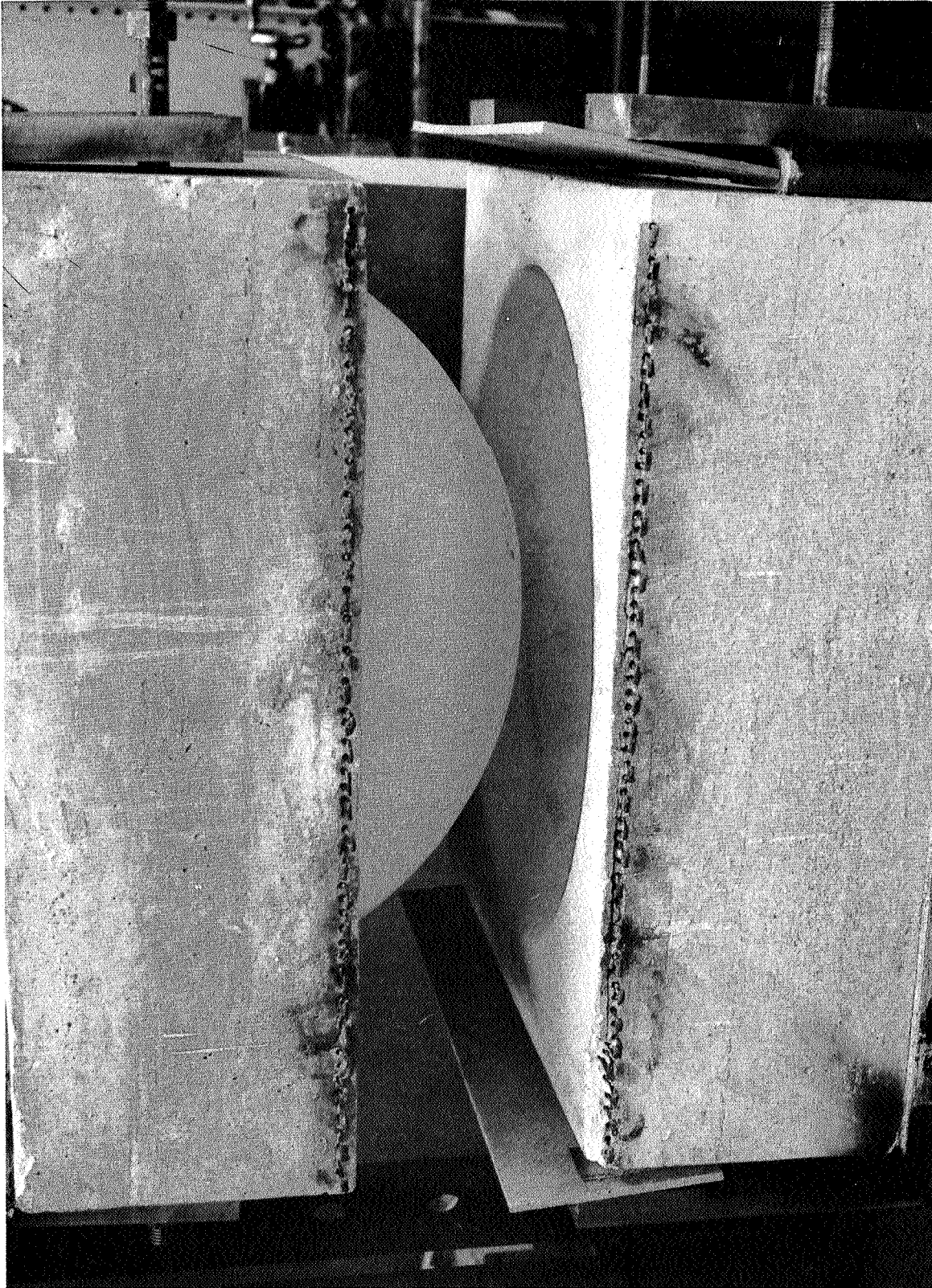
Figure 34 "Glassrock" Spherical Forming Die - 12.0" Radius
