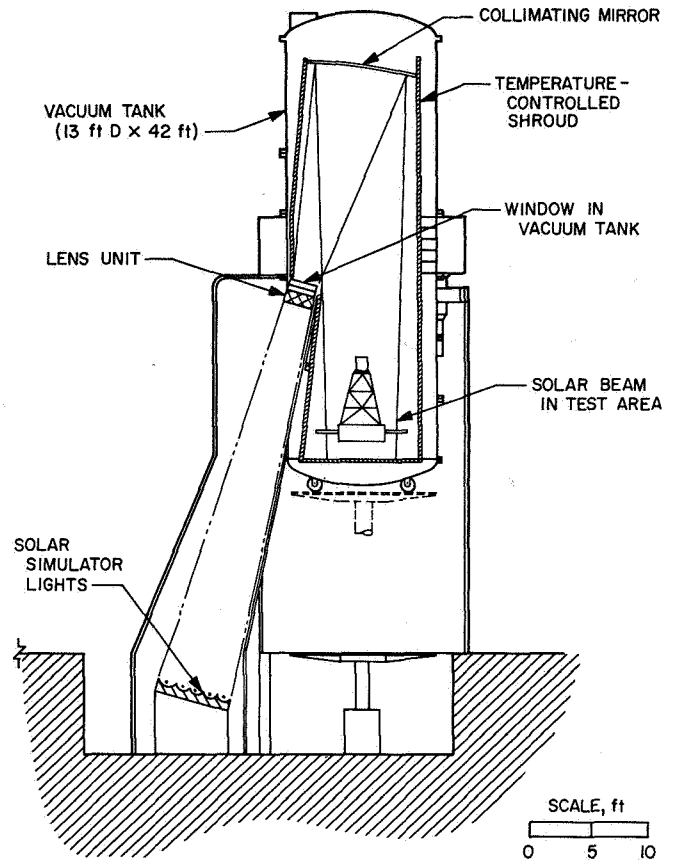
Figure 1. The JPL 10-ft space simulator
