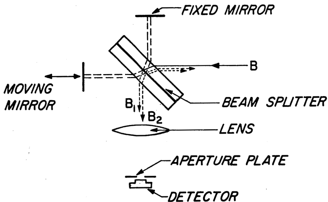
Fig. 1 Basic Instrument
