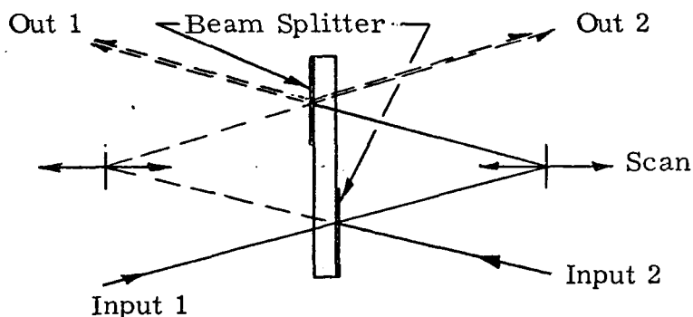
Fig. 19 Skewed Michelson
