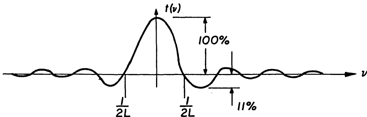
Fig. 9 Scanning Function
