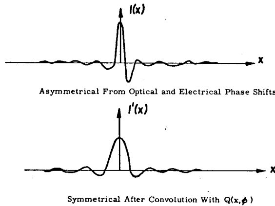
Fig. 18 Asymmetrical Corrections
