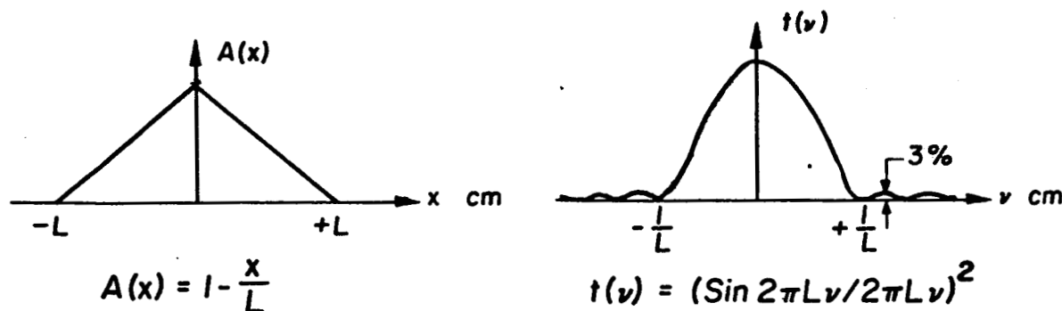
Fig. 10 Triangular Apodization
