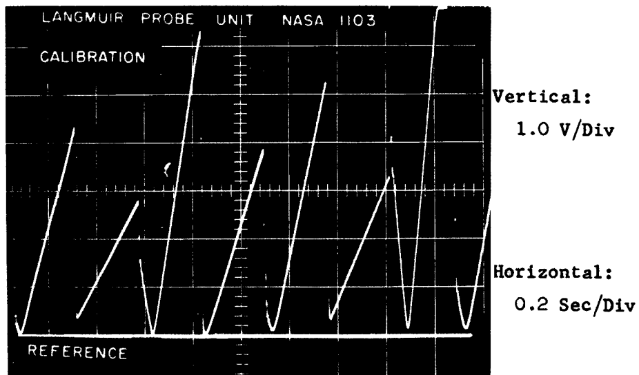
Figure 56. Calibration waveforms, Langmuir probe. R_d = 22 Meg.
