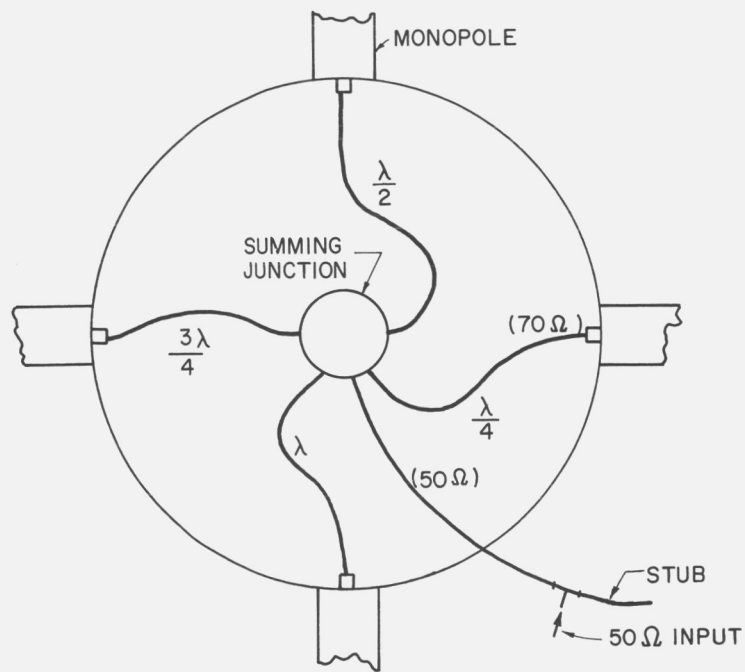
Figure 64. Antenna matching network.
