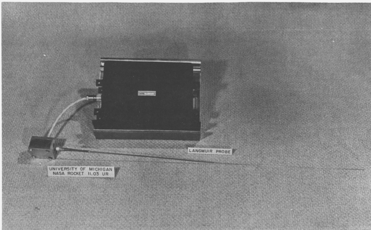
Figure 48. Langmuir probe.
