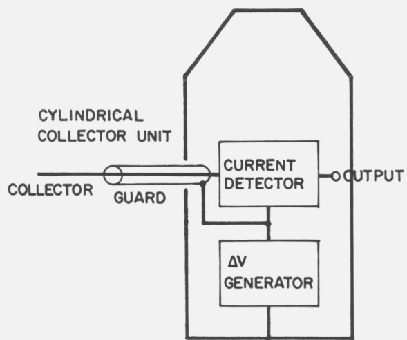
Figure 49. Langmuir probe experiment.
