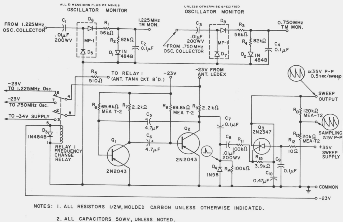
Figure 19. Sweep generator board.
