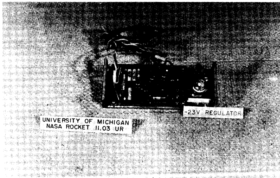
Figure 43. -23 volt regulator.
