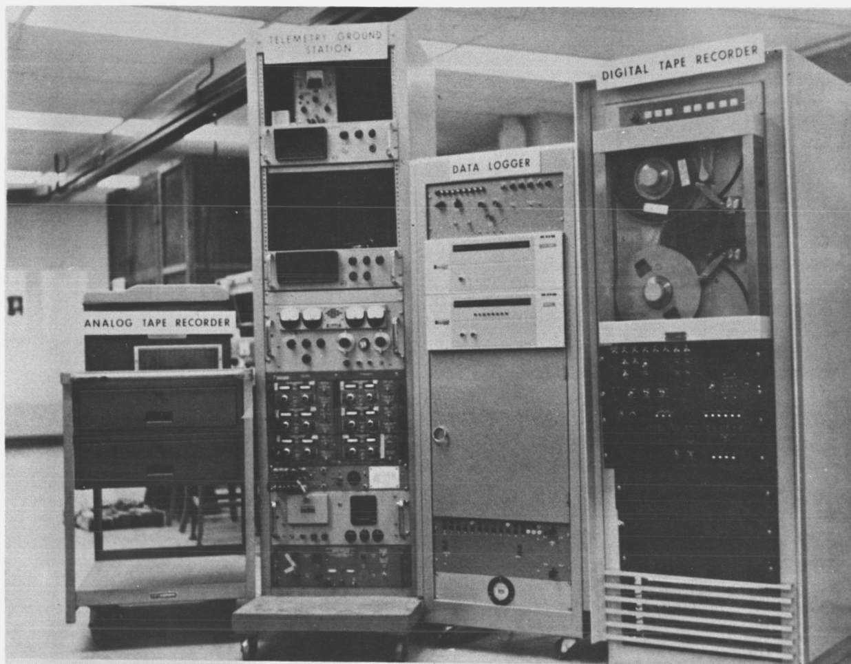
Figure 80. Data logger equipment.
