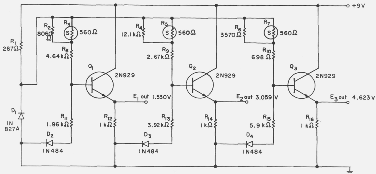
Figure 32. VCO calibrator.
