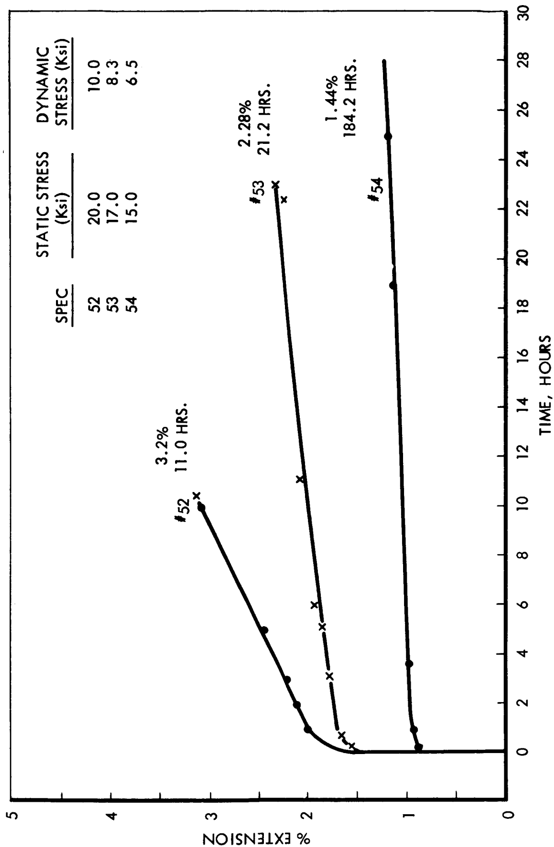
FIGURE 9 CREEP OF TZC UNDER DYNAMIC LOAD CONDITIONS, TEST TEMPERATURE 1800°F, VACUUM ENVIRONMENT <1 \times 10^{-7} TORR, A \approx 0.45 .
