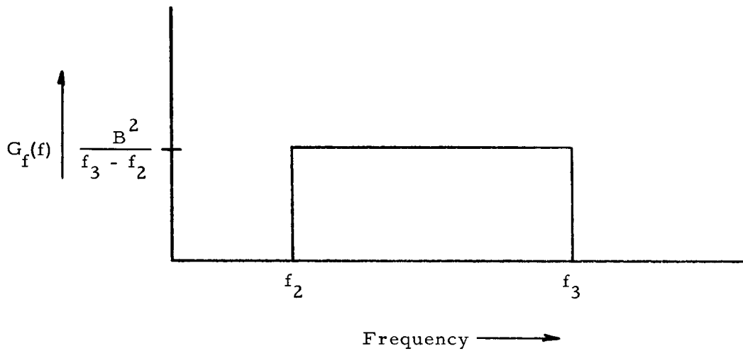
Figure 7-13. Ideal Bandpassed White Gaussian Flutter Spectrum
