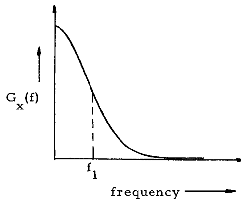
Figure 7-10. Gaussian Shaped Spectral Density
