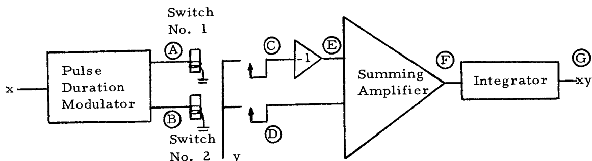
Figure 3-8. Time Division Multiplier
