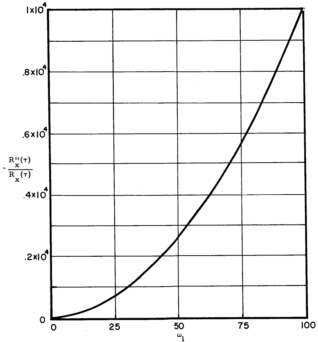
Figure 7-7. Data Related Phase Error Term for Sinusoidal Data
