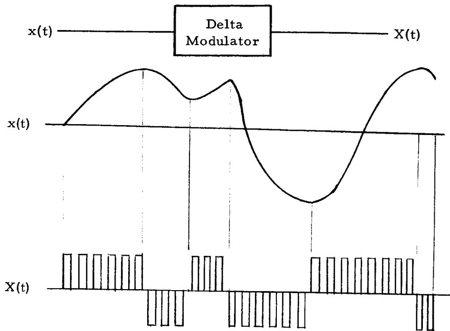
Figure 5-1. Delta Modulation Pulse Code
