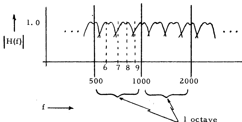
Figure 4-8. Filter Frequency Responses for 1/3 Octave Spectral Analysis
