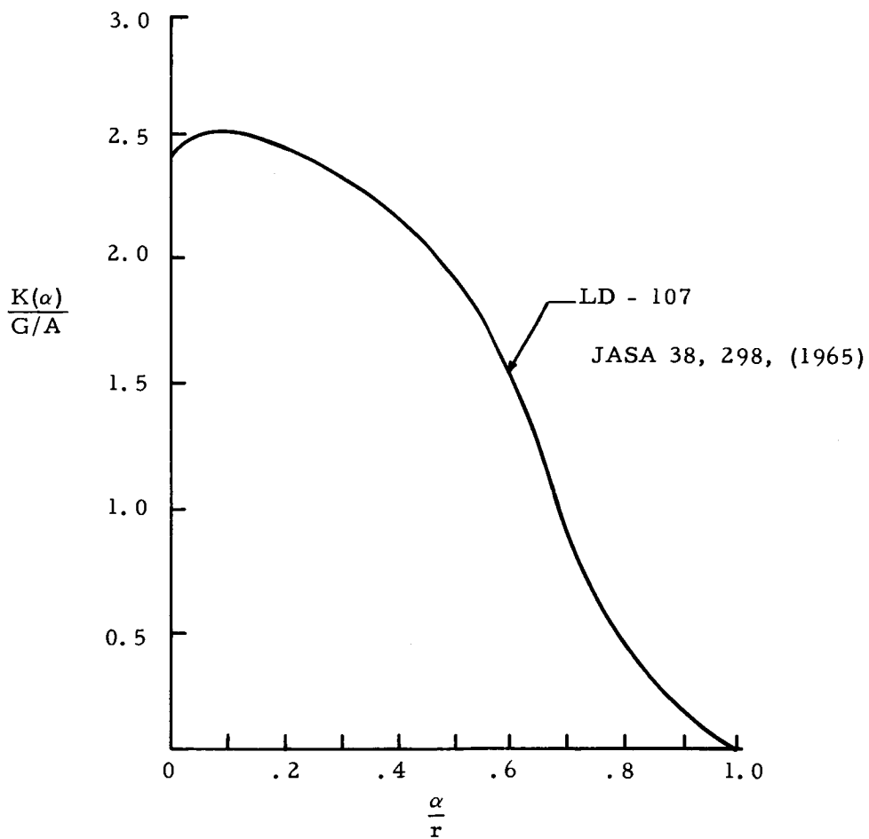
Figure 7-4. Transducer Sensitivity versus Distance from Center ( \alpha )
