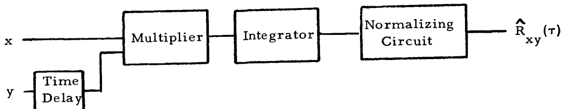
Figure 3-1. Block Diagram of an Analog Correlation Analyzer
