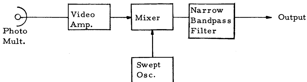
Figure 6-6. Block Diagram of a Correlation System
