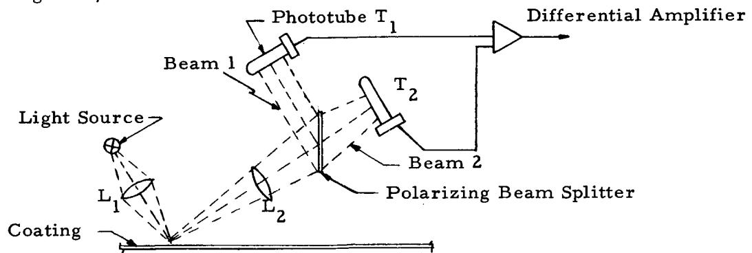
Figure 6-1. Functional Diagram of a Magneto-Optical Playback System
