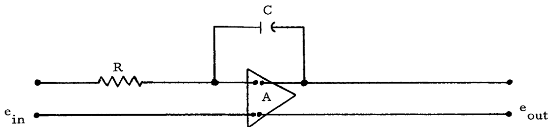
Figure 3-10. Operational Amplifier Integrator
