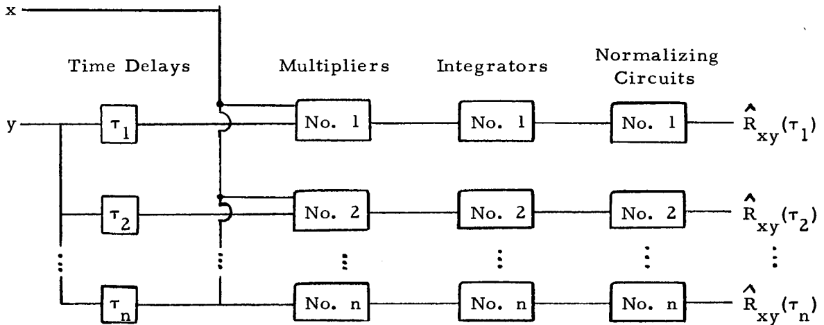
Figure 3-2 Block Diagram of a Real Time Correlation Analyzer
