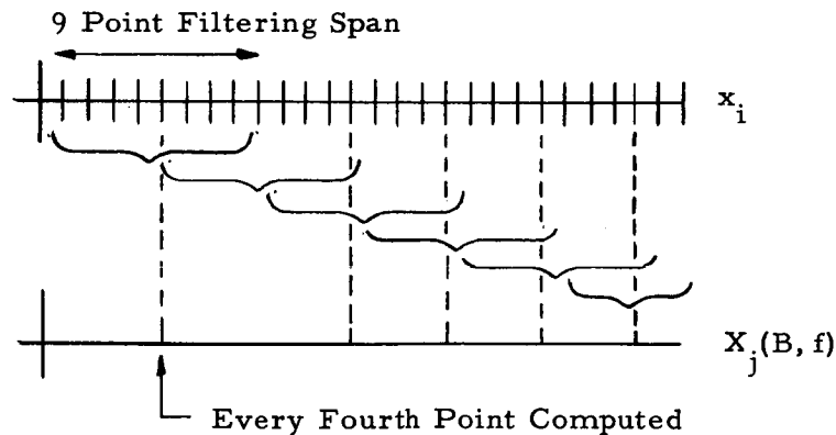
Figure 4-3. Illustration of Decimation
