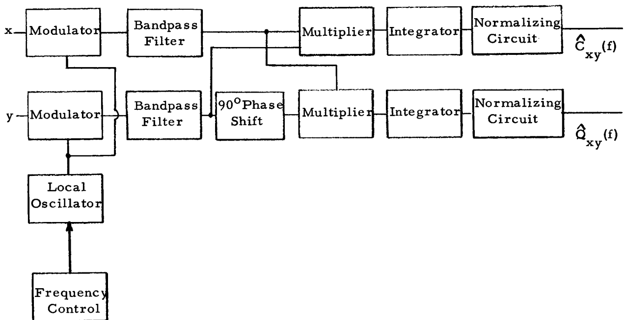
Figure 3-14. Cross-Spectral Density Analyzer Using Heterodyne Techniques
