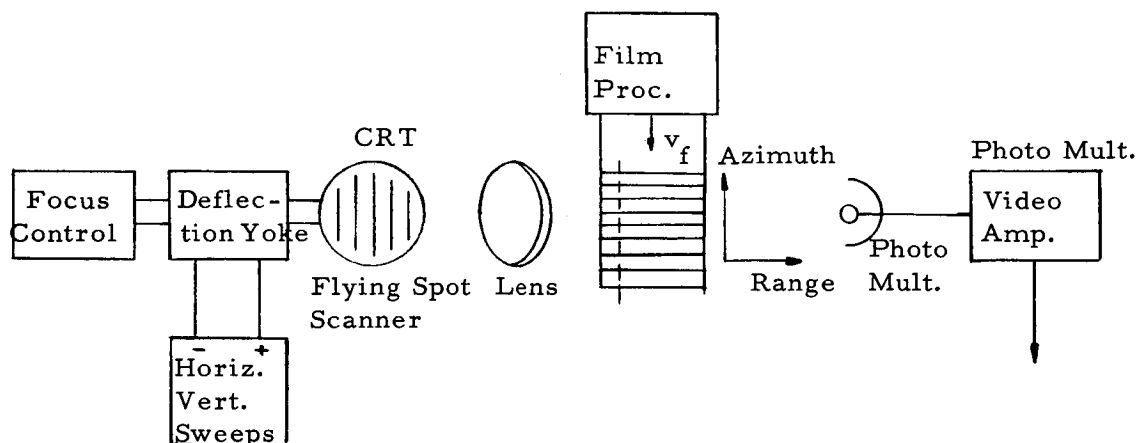
Figure 6.5. Block Diagram of a Film Readout System
