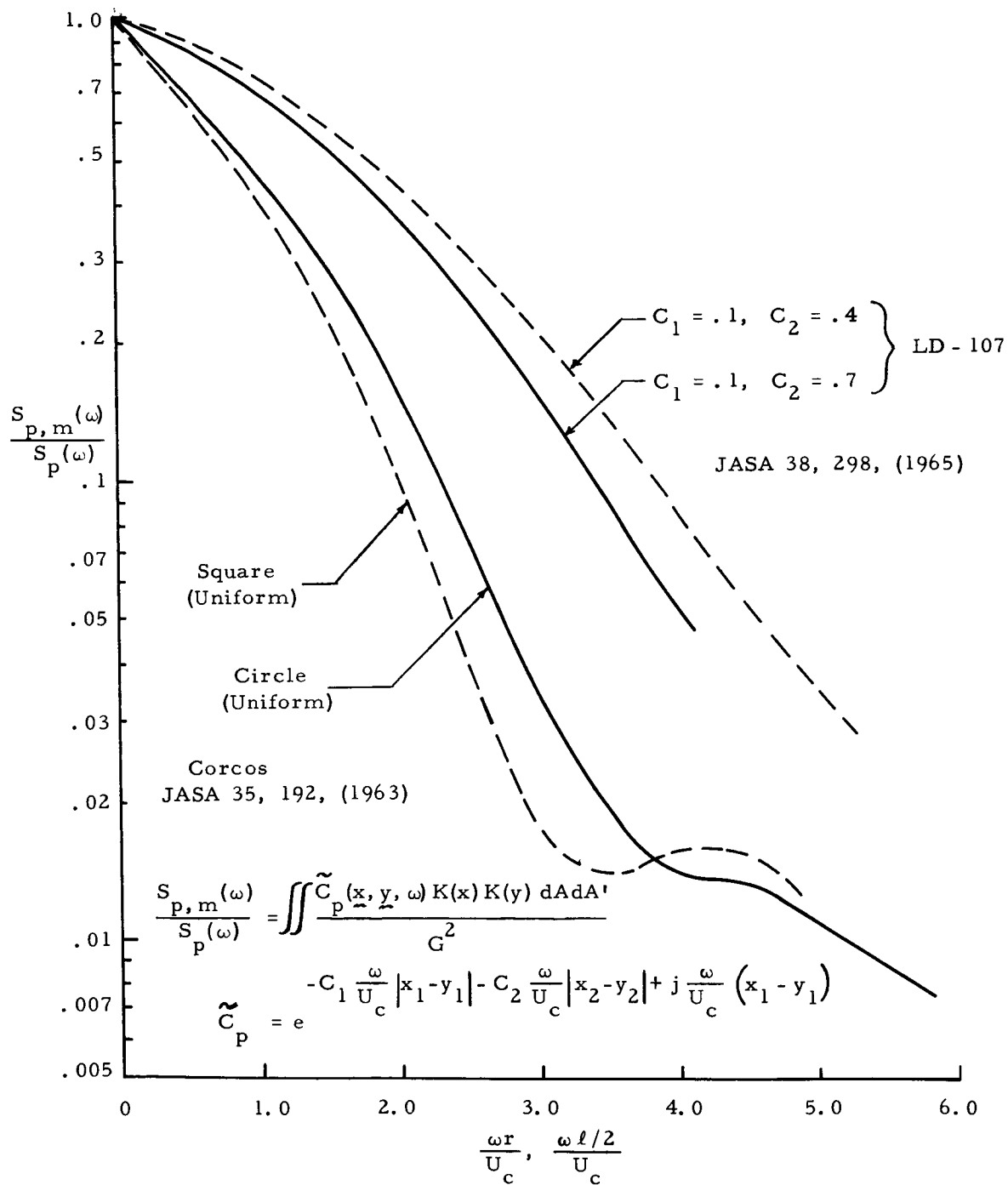
Figure 7-5. Correction Factor for Finite Size Transducer
