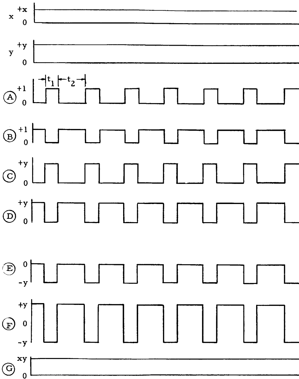
Figure 3-9. Waveforms in a Time Division Multiplier
