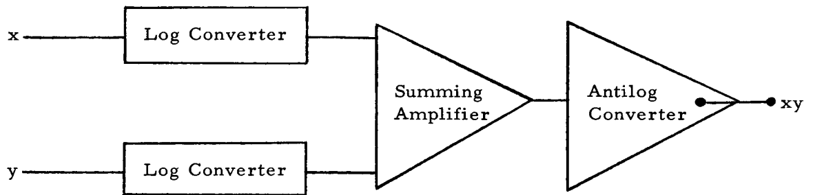
Figure 3-5. Logarithmic Multiplier
