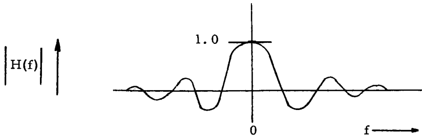
Figure 4-4. Filter Frequency Response of Sin x/x Form
