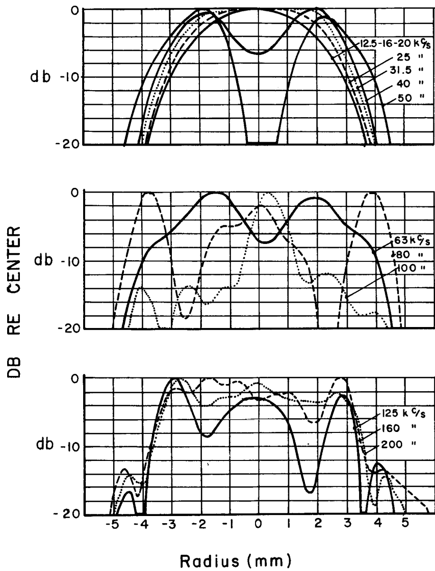
Figure 7-6. Sensitivity of B & K 4134 Microphone
