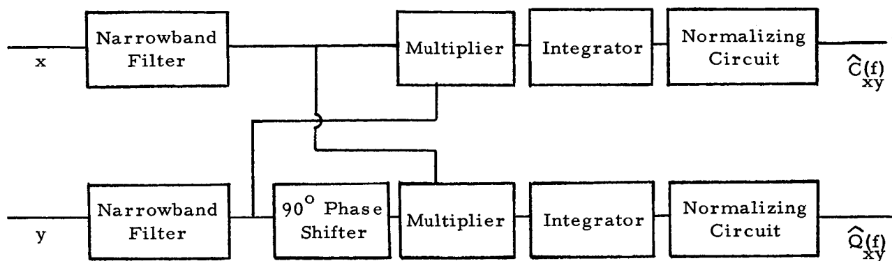
Figure 3-11. Block Diagram of an Analog Cross-Spectral Density Analyzer
