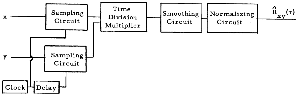
Figure 5-4 Analog Sampling Hybrid Correlator
