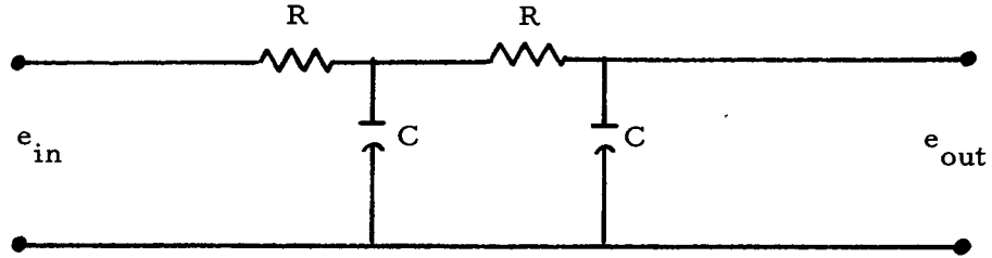
Figure 3-13. 90^\circ Phase Shift Circuit for Narrowband Signals
