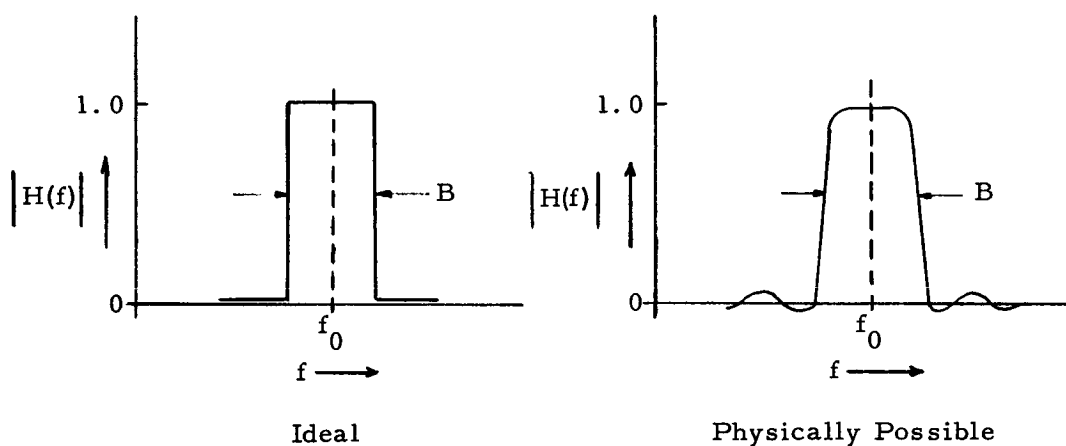
Figure 4-2. Spectral Analysis Filter
