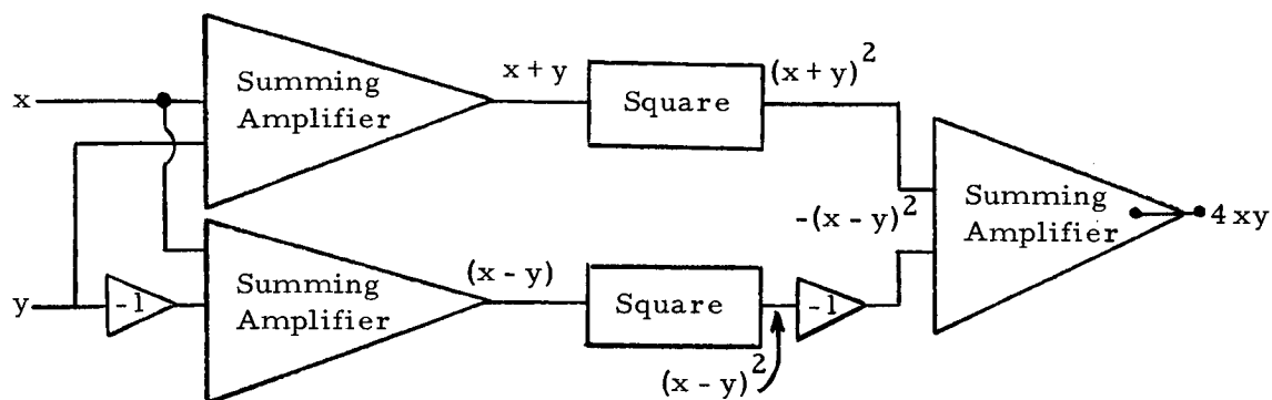
Figure 3-7. Quarter Square Multiplier
