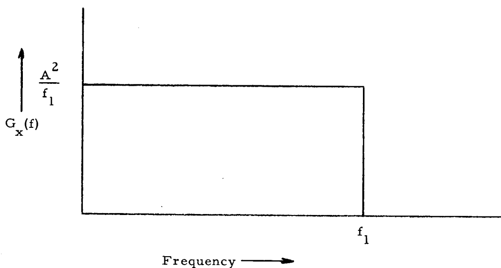
Figure 7-8. Spectral Density of Ideally Low Passed White Gaussian Noise
