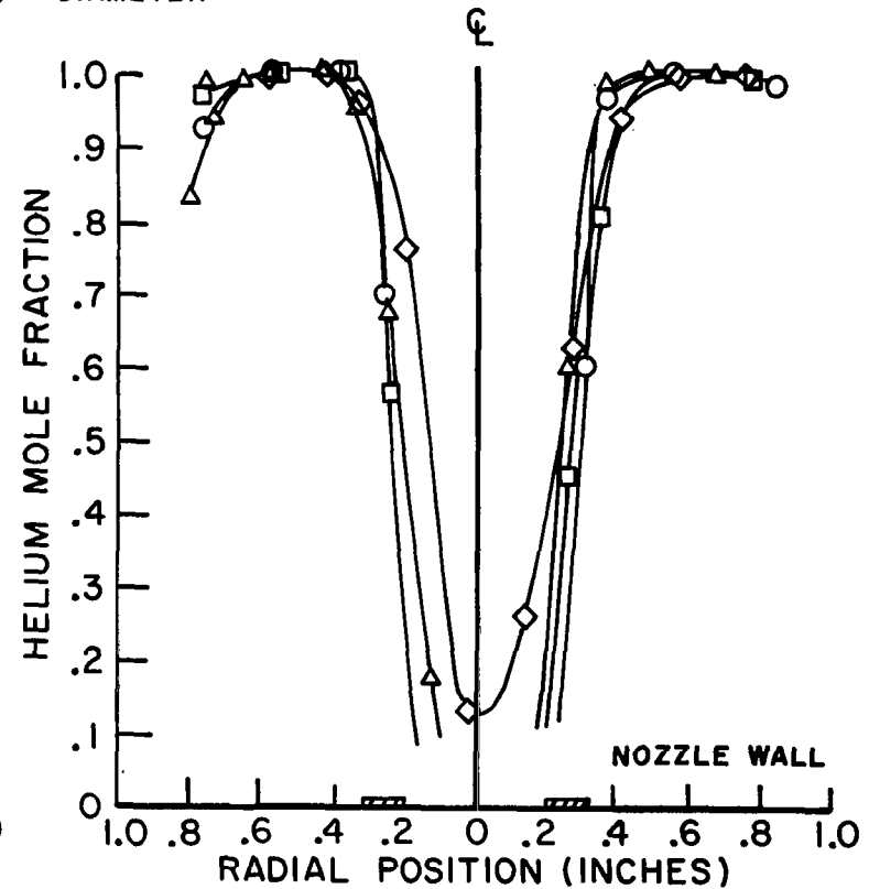
PROFILES OF ARGON JET MIXING ISOTHERMALLY WITH COAXIAL HELIUM FLOW
