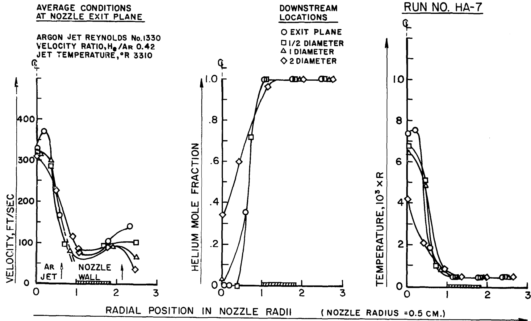
HALF-PROFILES OF ARGON ARCJET JET MIXING WITH COAXIAL HELIUM FLOW
