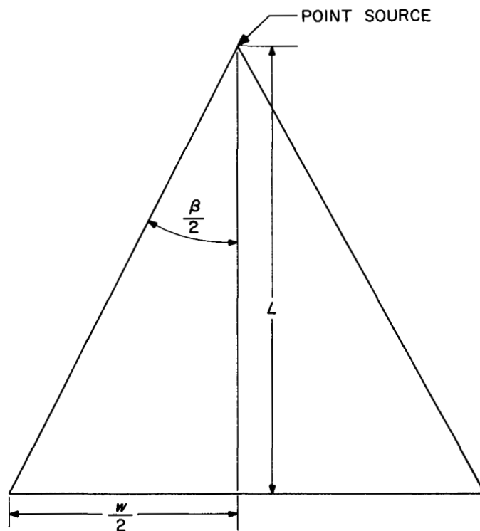
Fig. 29. Sheet geometry on deflector (simplified)
