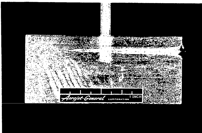
Cross-section view of a T-weld specimen showing the weld nugget through the blade. The weld specimen has braze on the right side at the simulated blade-to-disc joint.
