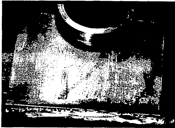
Bottom view of the same joint shows no evidence of erosion or weld burnthrough.
