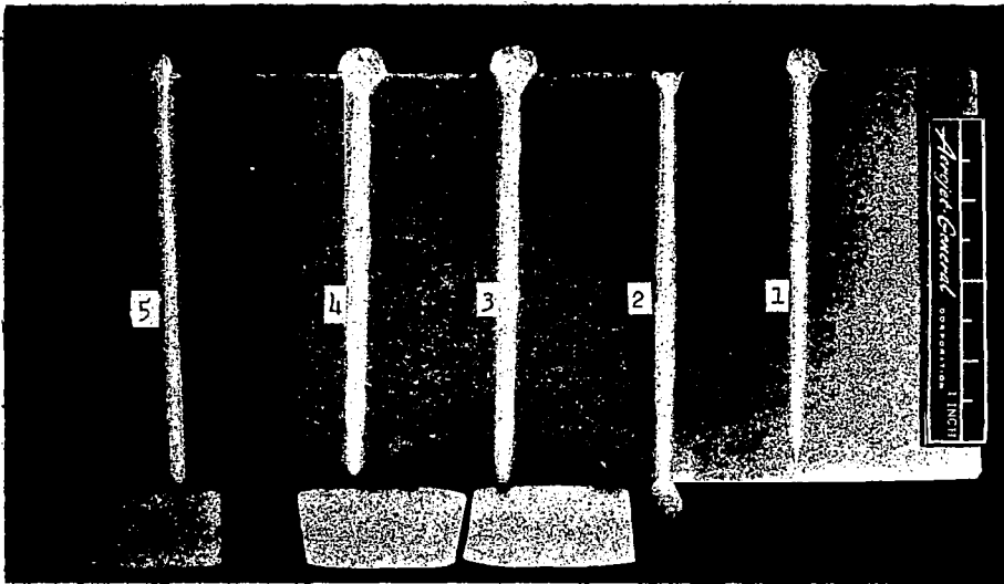
Welds No. 1 to 5 demonstrate the effect of minor electron-beam weld schedule changes on the nugget configuration. The test block is 1.3-in. thick. The schedules used are shown below.
