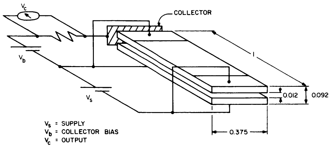
FIG. 1 ELECTRON MULTIPLIER
