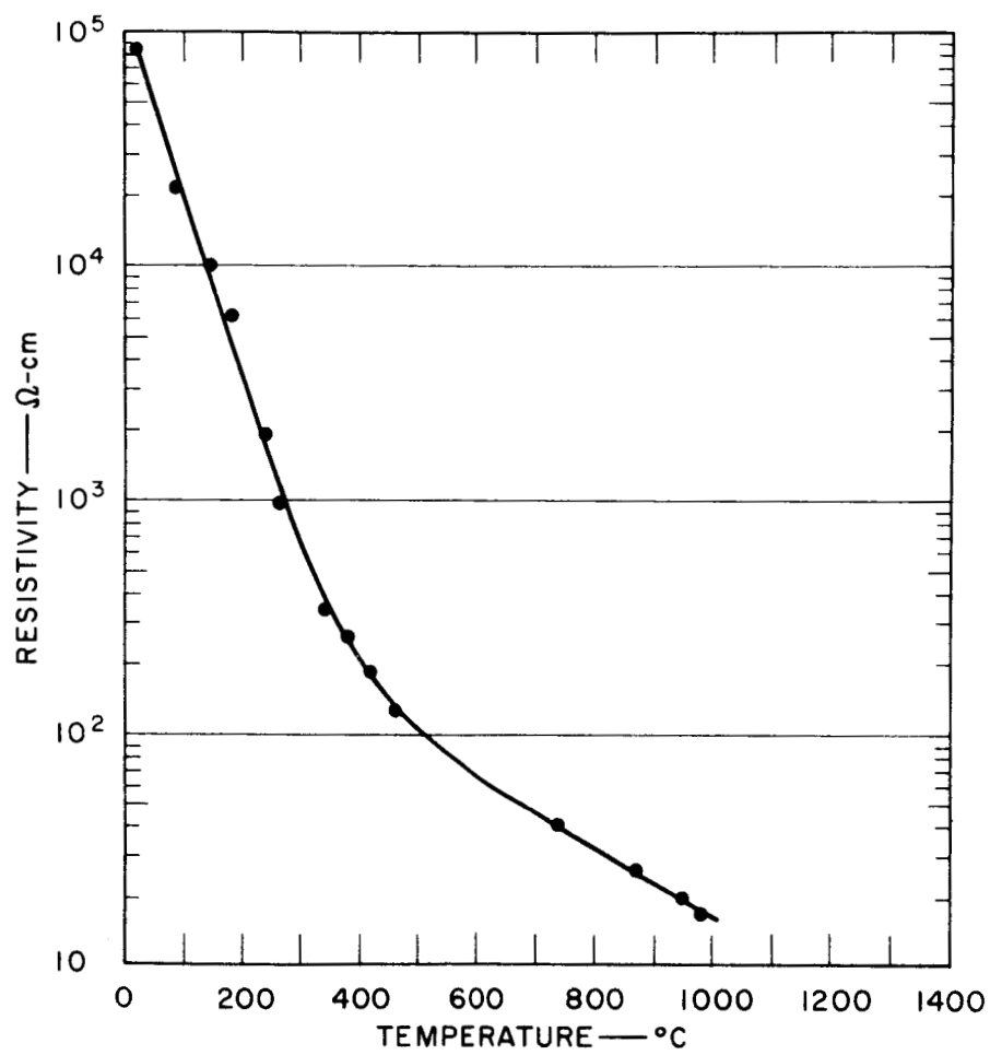
FIG. 8 DYNODE RESISTIVITY vs. TEMPERATURE
