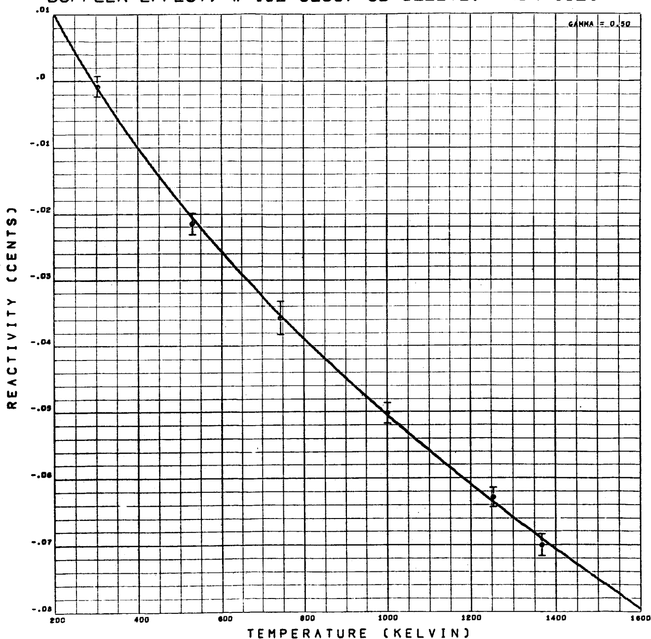
Figure 6. Experimental Points and Least-squares Fit for Doppler Measurements on W 182 , Single Run.
