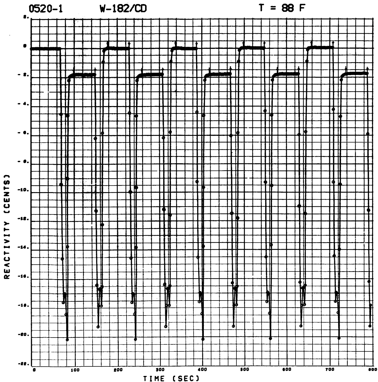
Figure 15. Reactivity vs Time Determined from Power History for Run 0520-1 (Room Temperature)
