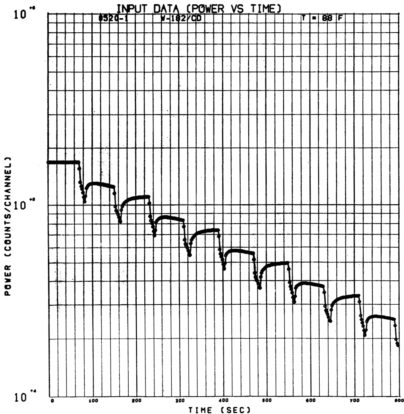
Figure 14. Power History from Typical Oscillator Run (0520-1)
