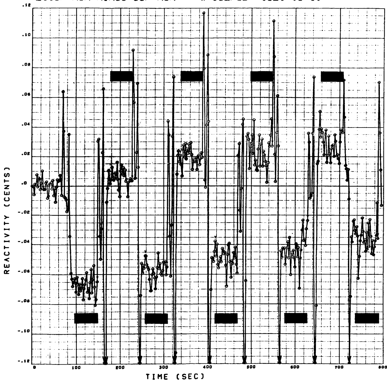
Figure 17. Pointwise Reactivity Difference, 1368°K Run Minus Room-Temperature Run, Magnified Scale
