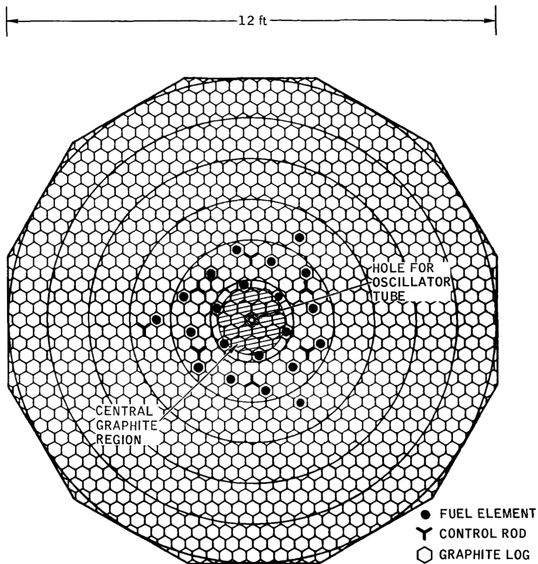
Figure 3. SGR-CA Critical Core Loading for 10.6-in. Lattice Spacing (Sample is inserted into full-height axial hole at center of core. Cross hatching denotes central graphite region providing 1/E spectrum in axial hole. All control rods are withdrawn during measurement except one at far left.)
