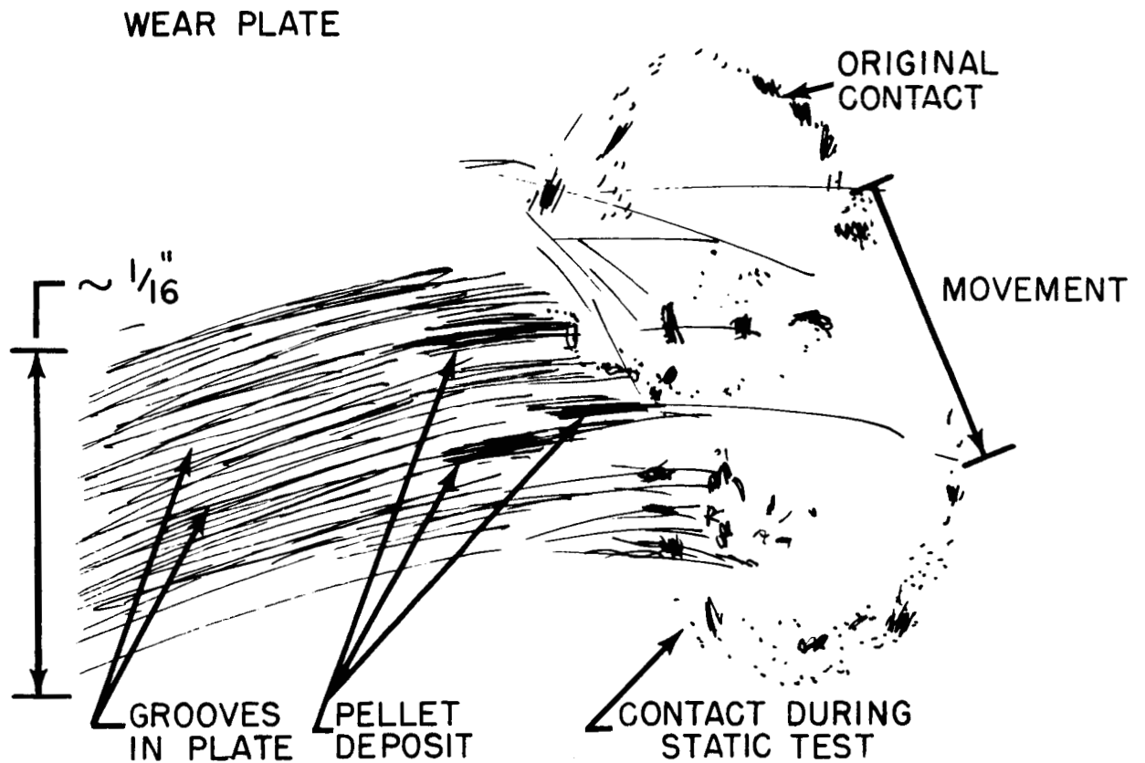
Fig. 2 - Description of Probable Motion of the Pellet Surface on the Wear Plate Surface.
