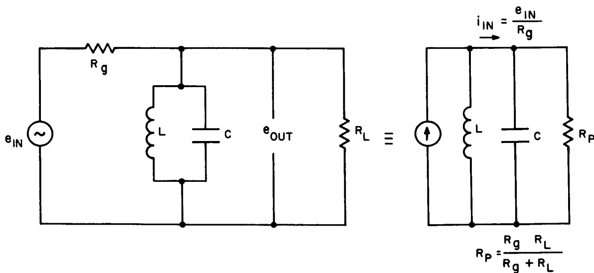
Figure 6-44. Single-Pole Tuned Circuit
