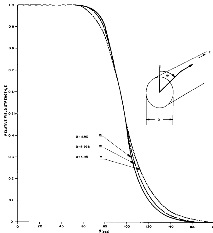
Figure 6-42. Relative Voltage Pattern for an Axial Dipole on a Cylinder ( \lambda = 0.187 m)
