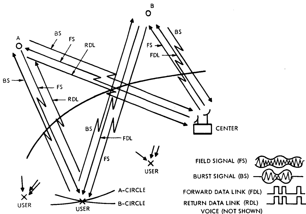
Figure 2-2. Traffic Control
