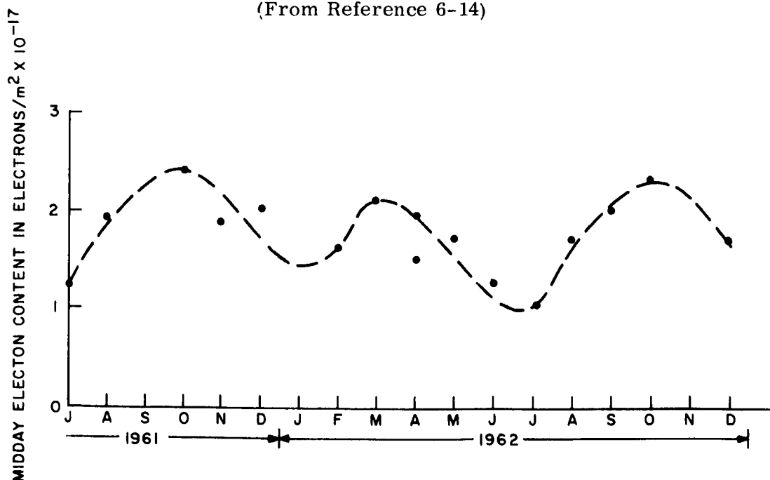
Figure 6-16. Seasonal Variation of Midday Electron Content, July 1961 to December 1962.
