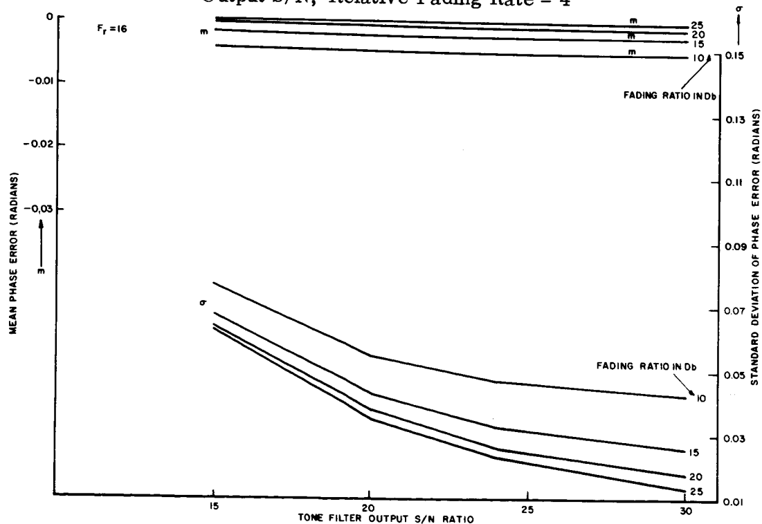
Figure 6-71. Mean and Standard Deviation of Phase Error vs. Tone Filter Output S/N, Relative Fading Rate = 16
