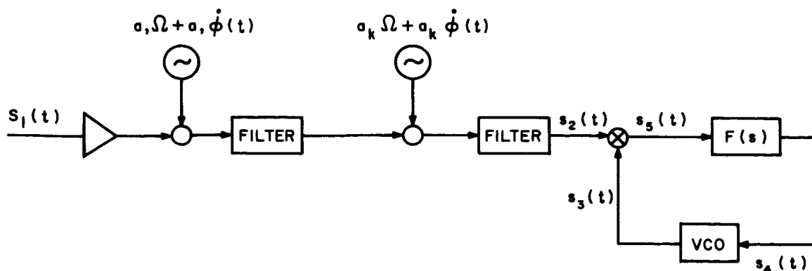
Figure 6-50. Typical Phase-Lock Receiving System
