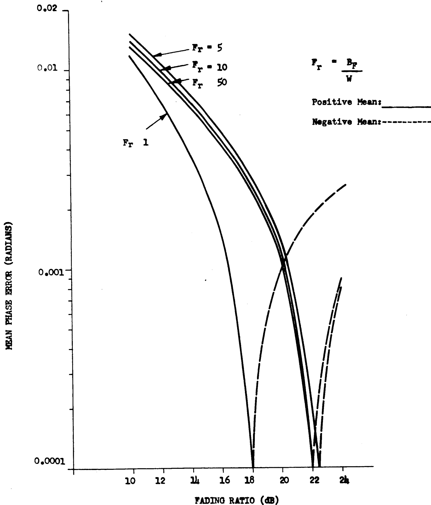
Figure 60-1 MEAN PHASE ERROR VS. FADING RATIO
