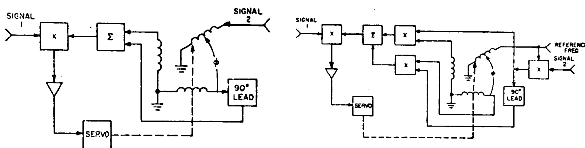
Figure 2-11. Phase Measurement Using a Resolver
