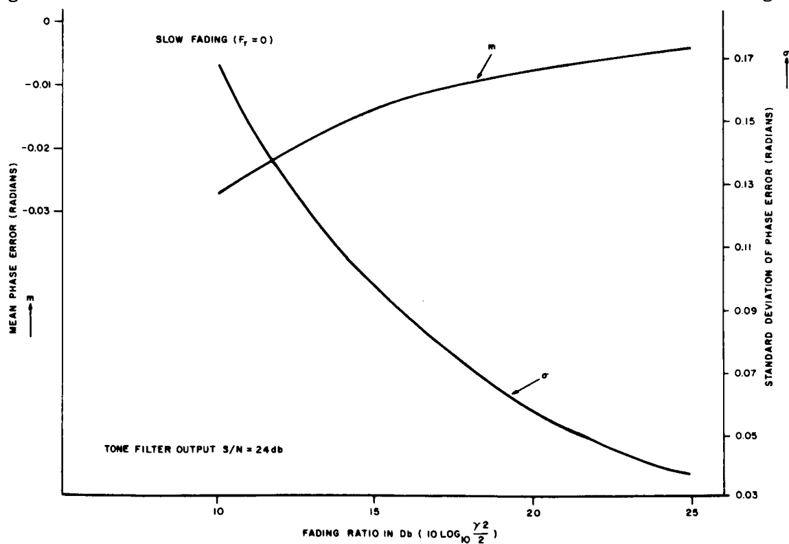
Figure 6-61. Mean and Standard Deviation of Phase Error vs. Fading Ratio, Tone Filter Output S/N = 24 dB
