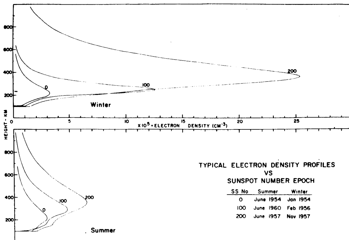
Figure 6-13. Solar Cycle Changes in Noon N(h) Profiles (From Ref. 6-12) (After J.W. Wright, 1962, Dependence of the Ionospheric F Region on the Solar Cycle, Nature 194, 461.)
