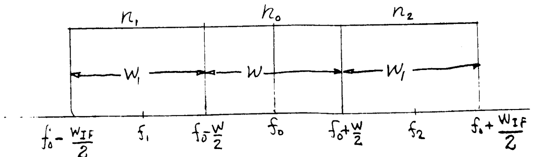
Figure 6B-1. Decomposition of the Power Spectrum of n(t)
