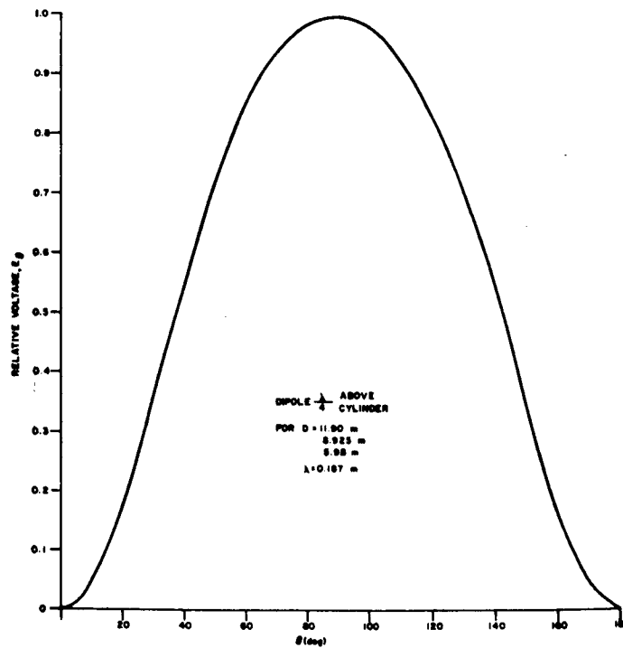
Figure 6-41. E_0 Pattern for \phi = 0^\circ
