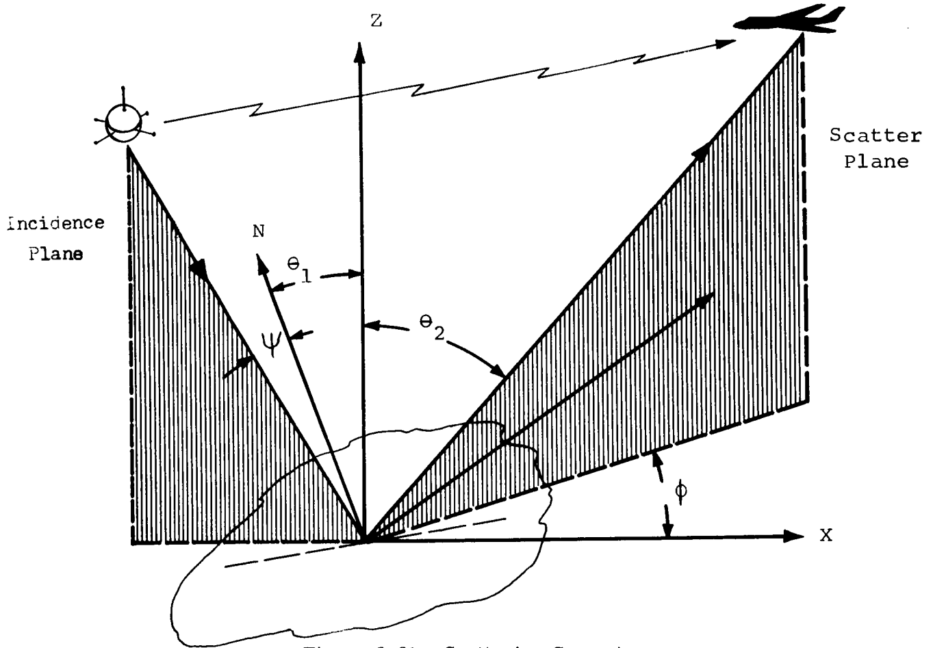
Figure 6-31. Scattering Geometry
