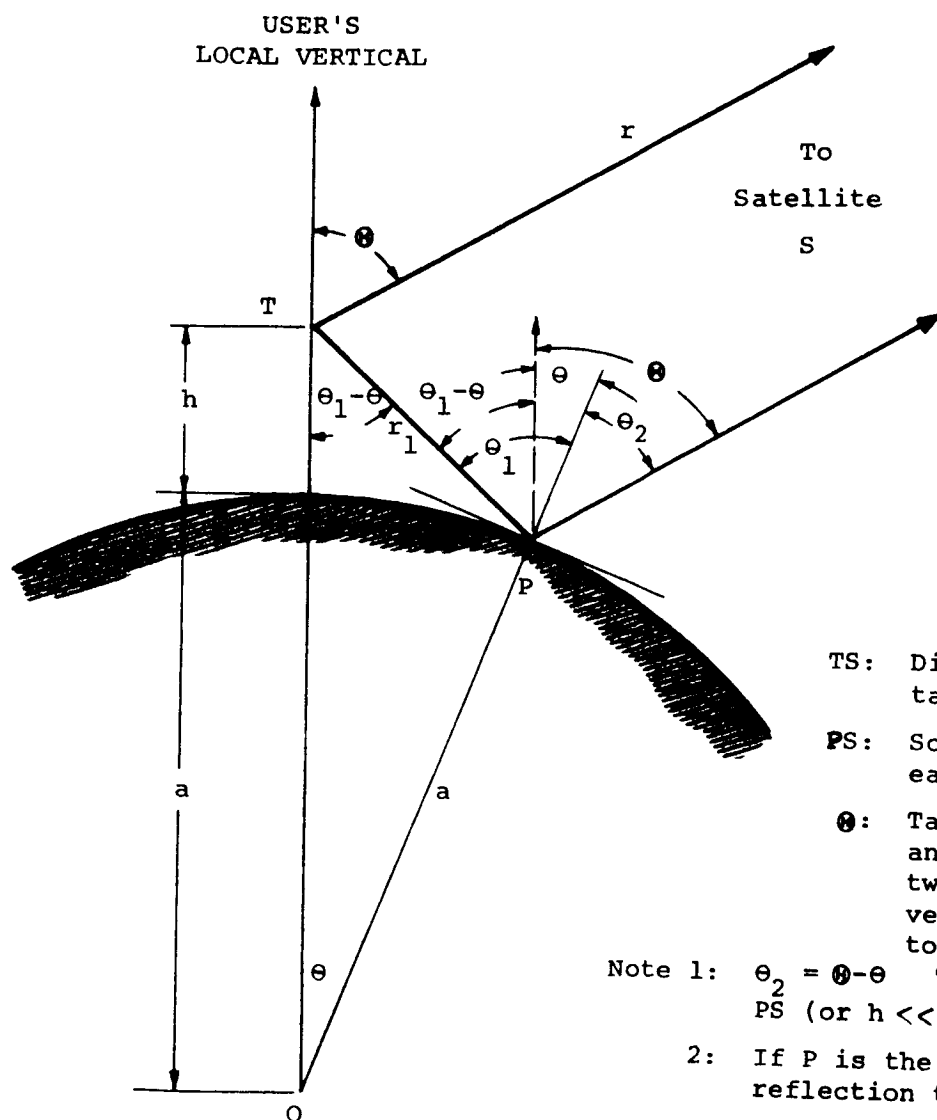
Figure 6-32. Multipath Geometry
