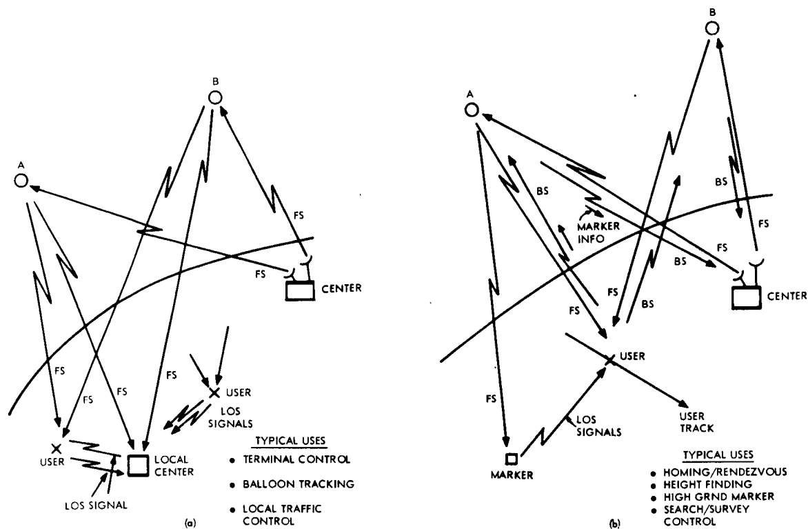
Figure 2-4. Relative Navigation
