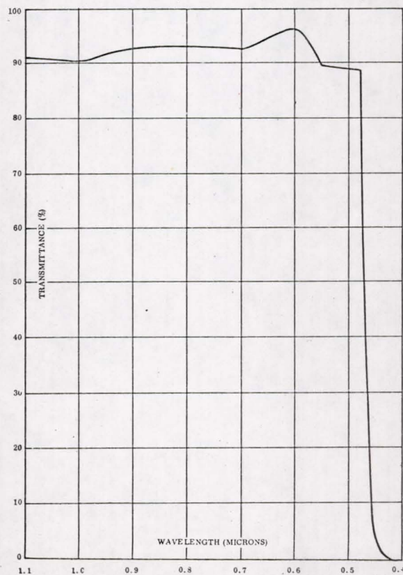
Figure 2-2. Transmittance Test Results
