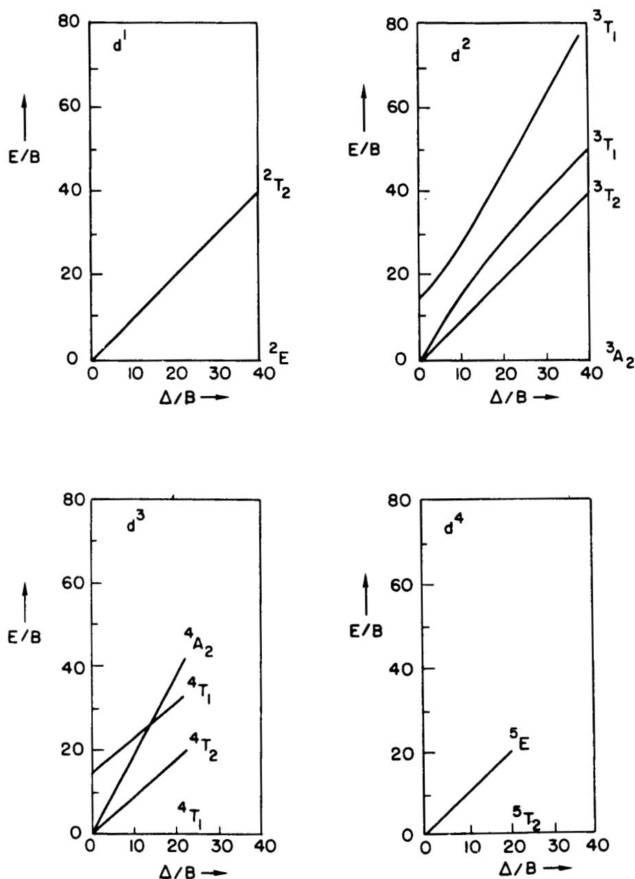
FIG. 10. CRYSTAL FIELD LEVELS OF MAXIMUM SPIN FOR d^n CONFIGURATIONS IN TETRAHEDRAL SITES. (Manganese has only one sextet state, so quartet levels are also shown.)
