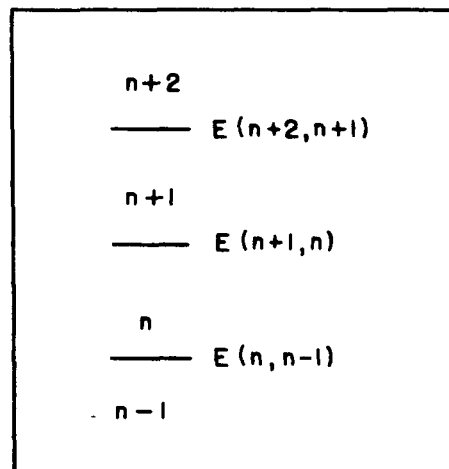
FIG. 4. RELATION BETWEEN CHARGE STATES AND ENERGY LEVELS.
