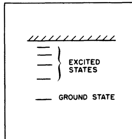
FIG. 2. EXCITED STATES OF A HYDROGEN-LIKE DONOR (SCHEMATIC).
