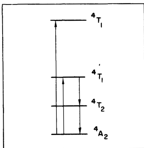
FIG. 14. POSSIBLE ASSIGNMENTS OF THE LUMINESCENT TRANSITION IN ZnS:Co.
