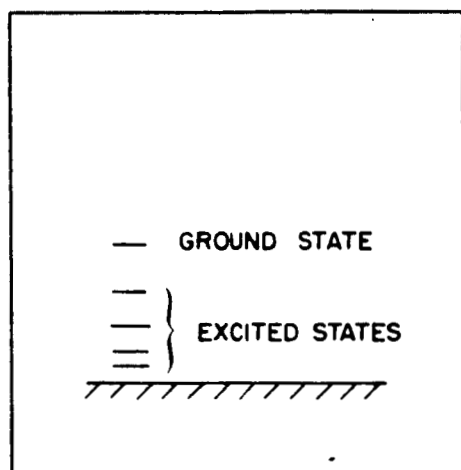
FIG. 3. EXCITED STATES OF A HYDROGEN-LIKE ACCEPTOR (SCHEMATIC).
