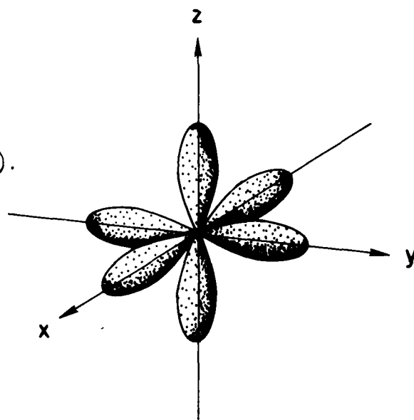
FIG. 9. A SET OF p-ORBITALS, p_x, p_y, p_z .
