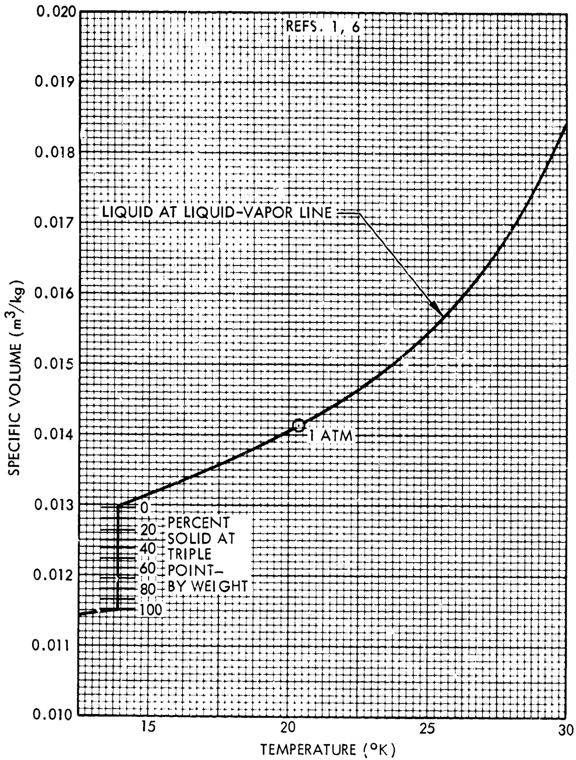
Fig. 3-22 Specific Volume of Liquid and Solid-Liquid Mixtures of Saturated Parahydrogen
