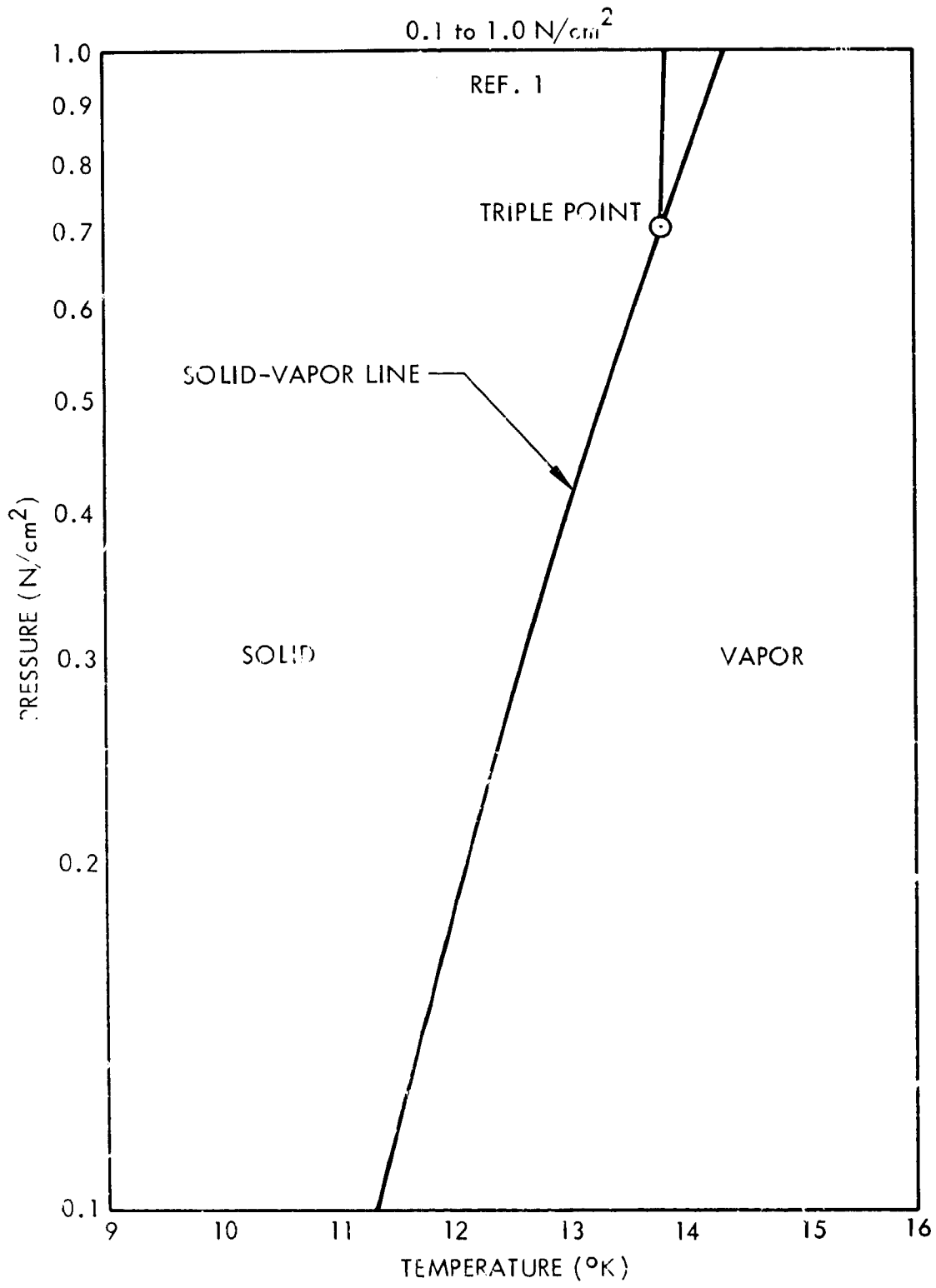
Fig. 3-3 Parahydrogen Pressure-Temperature Phase Diagram (0.1 to 1.0 N/cm 2 )
