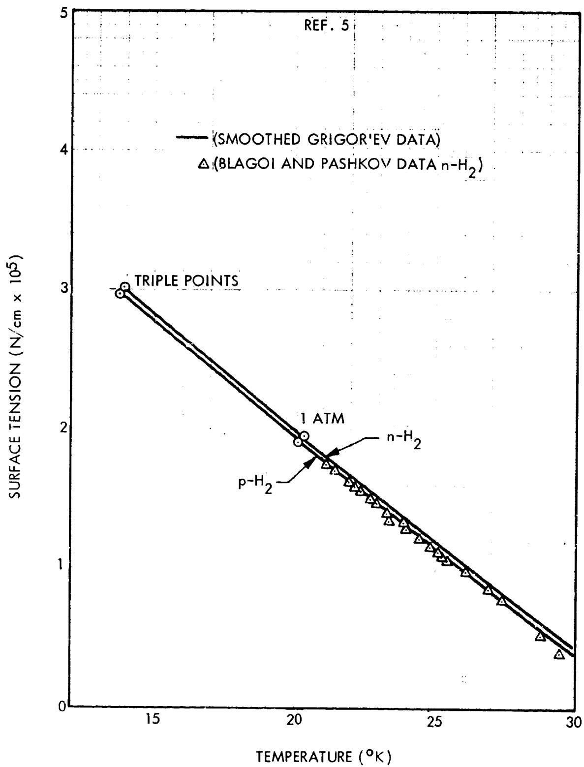
Fig. 3-27 Surface Tension Properties of Parahydrogen
