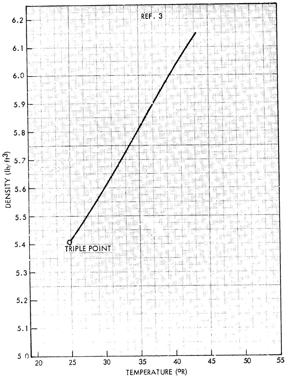
Fig. 2-21 Density of Solid Parahydrogen Along the Melting Line
