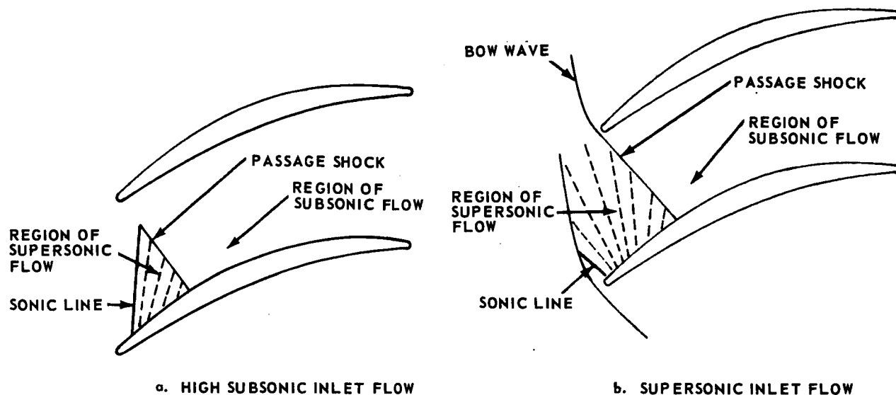
Figure 19 Assumed Blade Passage Flow Configurations
