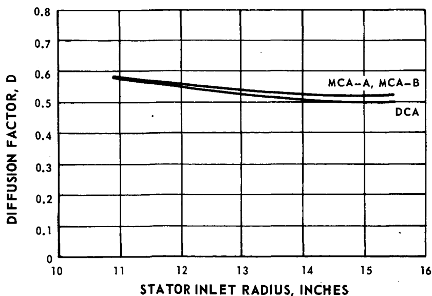
Figure 24 Blade Loading for MCA and DCA Stators
