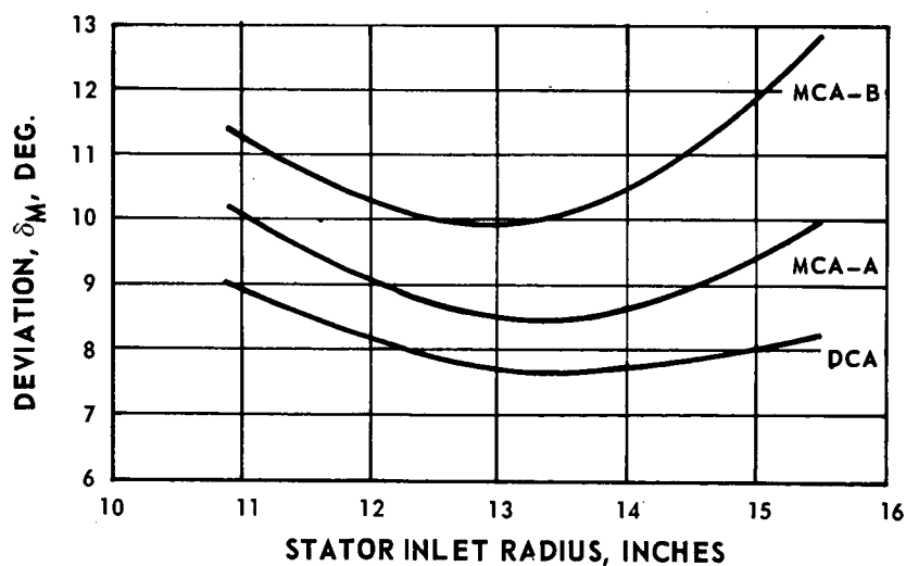
Figure 27 Estimated Deviation Angle for MCA and DCA Stators
