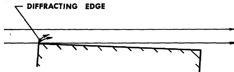
(c) \beta > 0
