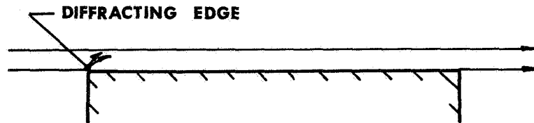
(b) \beta = 0
