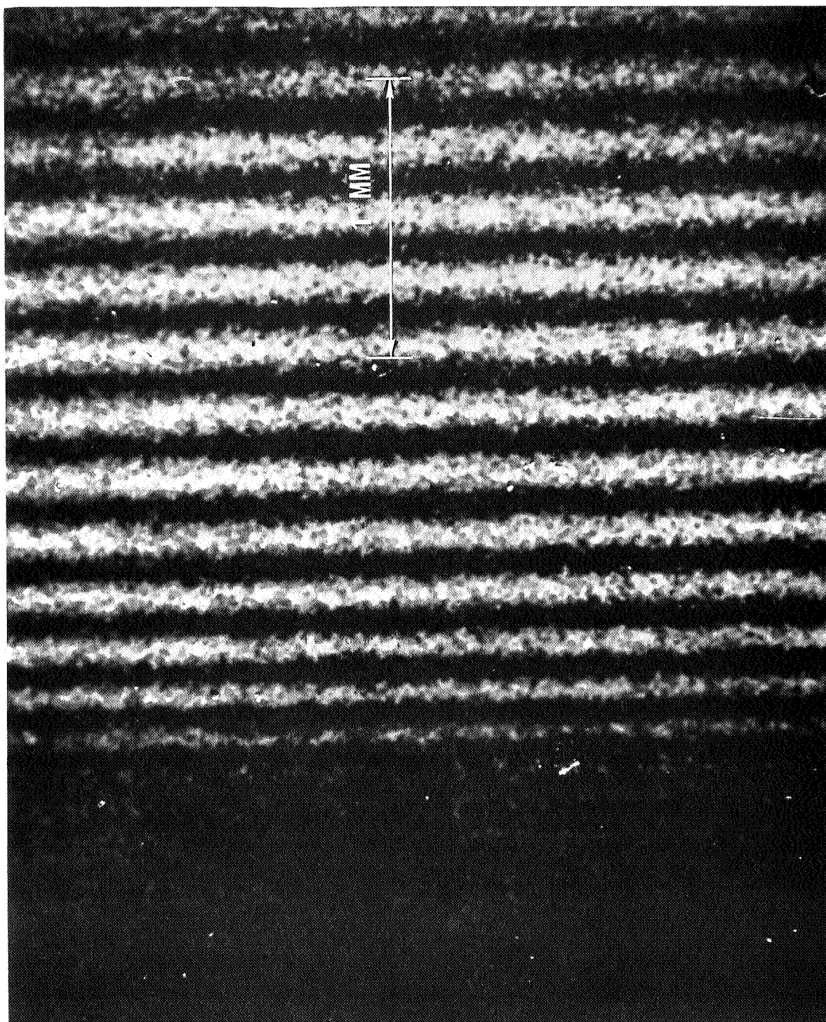
Fig. 10. Enlarged Interferogram of Narrow Fringes Oriented Parallel to the Wall. ( M_s = 5.51 , p_1 = 11 Torr, t = 488 \mu sec, Magnification \sim 100 ).
