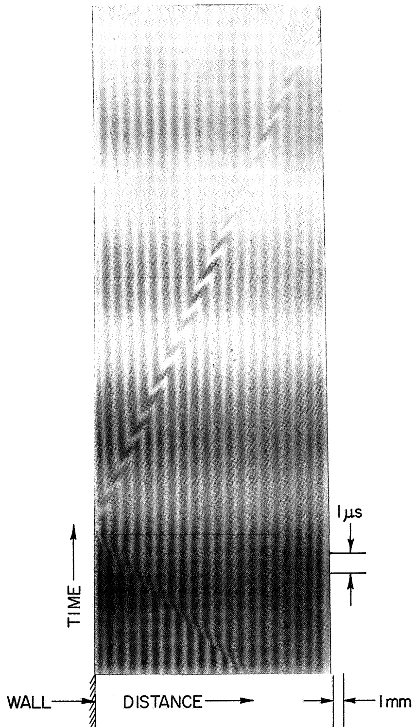
Fig. 6. Time-Resolved Interferogram of End Wall Region (M = 7.44, p_1 = 5 \text{ Torr})
