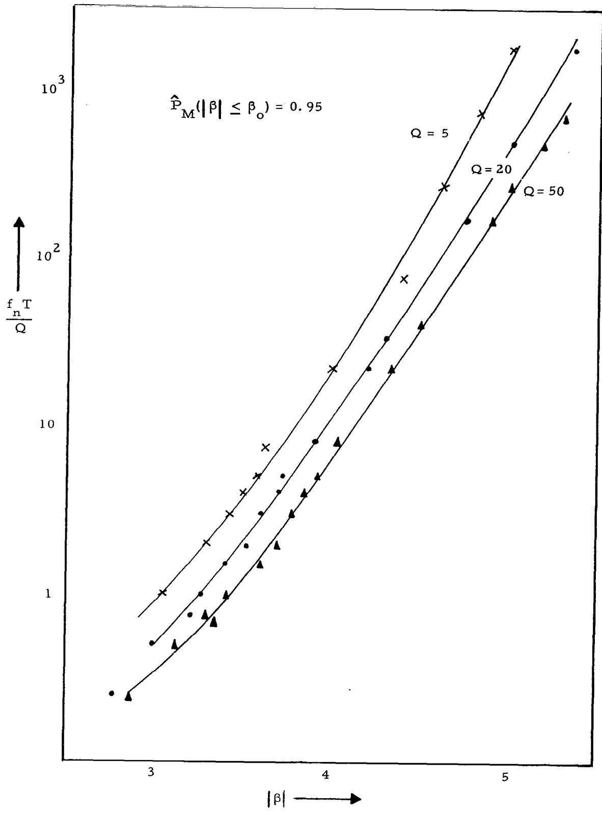
Figure 7. Response Maxima of a Single Degree-of-Freedom System to Stationary White Noise
