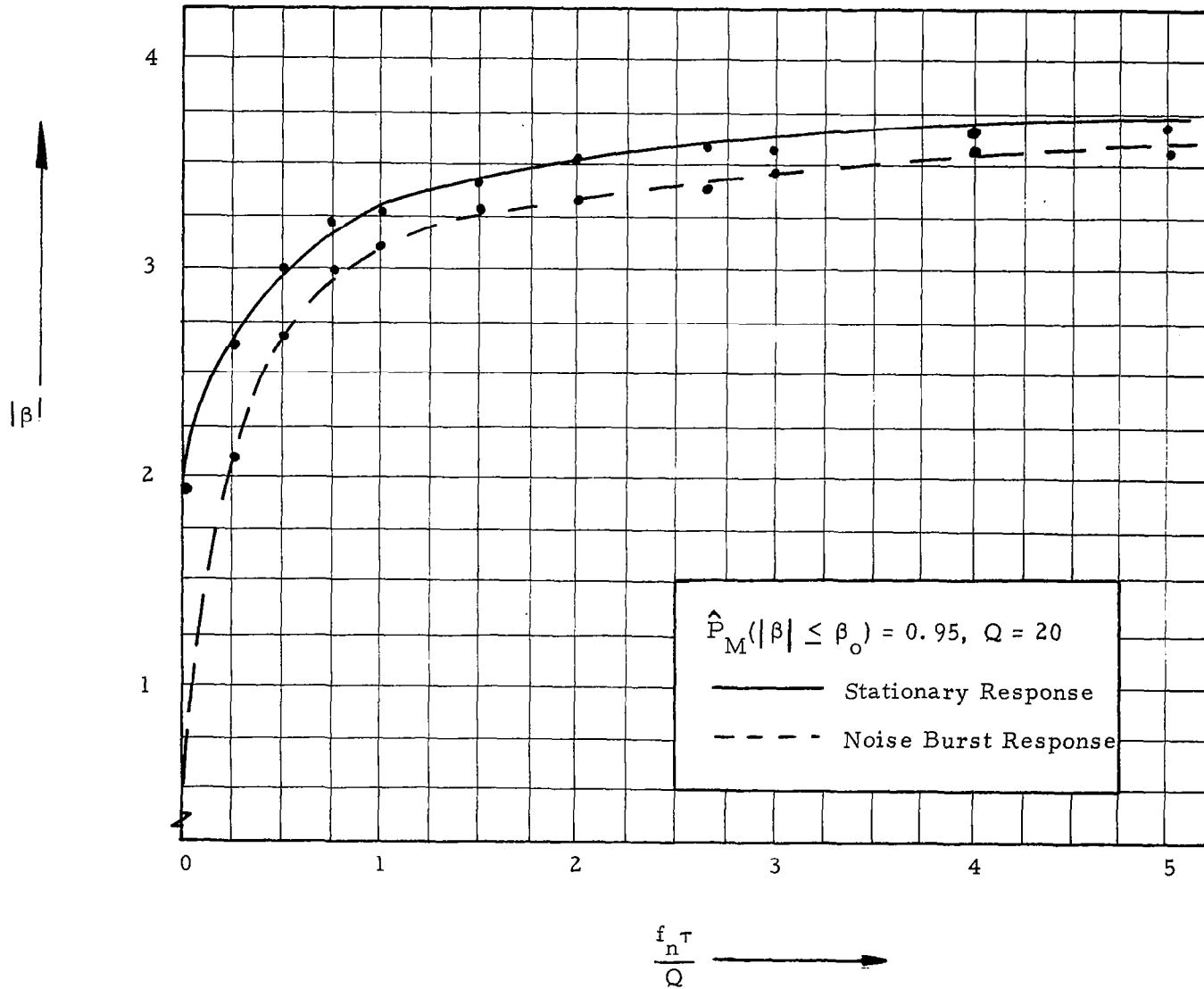
Figure 11. Response Maxima of a Single Degree-of-Freedom System to a Rectangular Burst of White Noise
