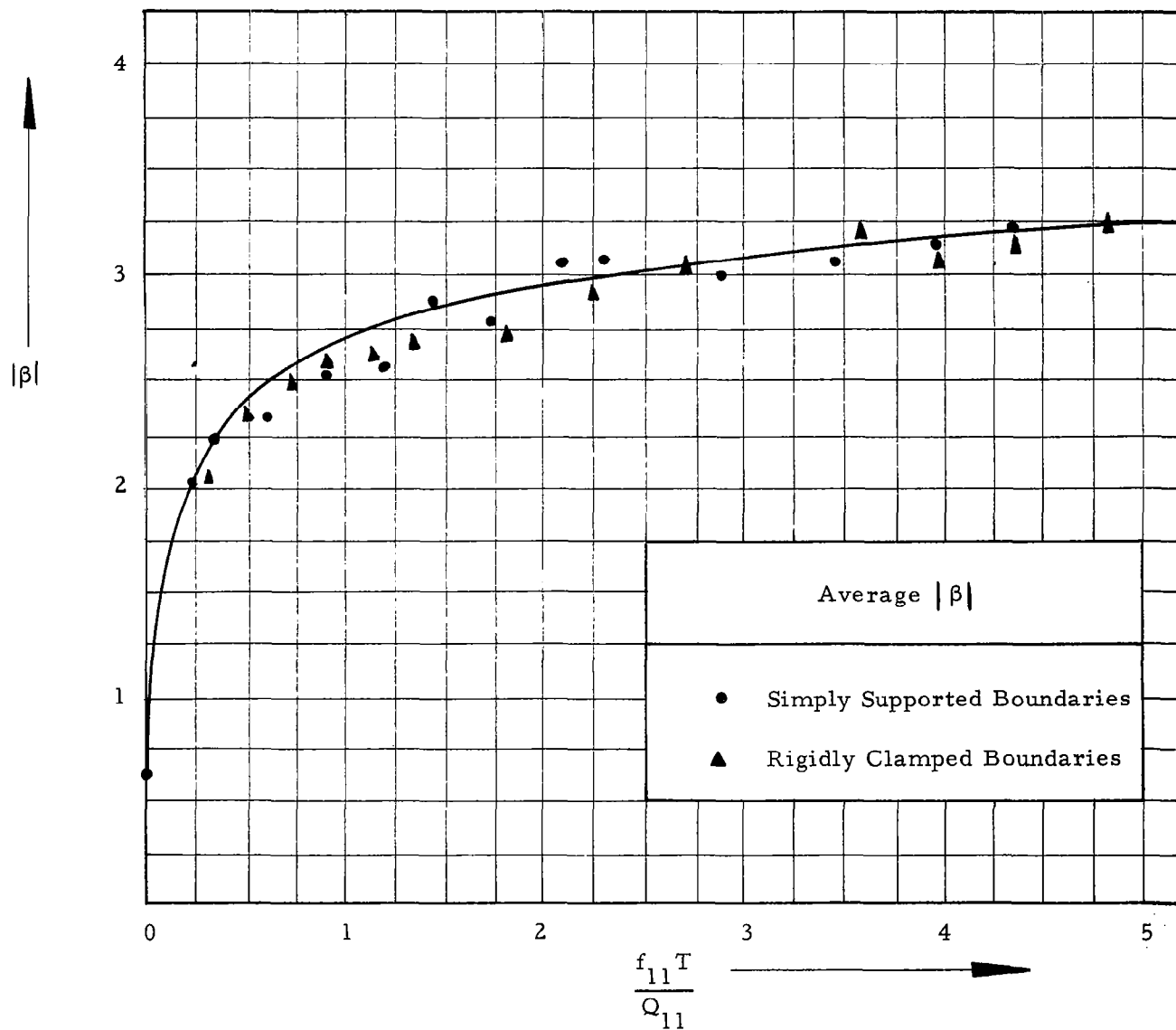
Figure 18. Maximum Response of a Square Plate to White Noise Correlated Perfectly in Space and Time
