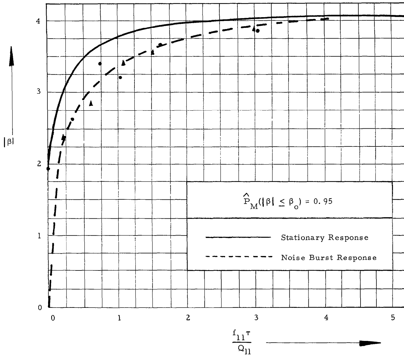
Figure 22. Maximum Response of a Square Plate to Rectangular Bursts of White Noise Correlated Perfectly in Space and Time
