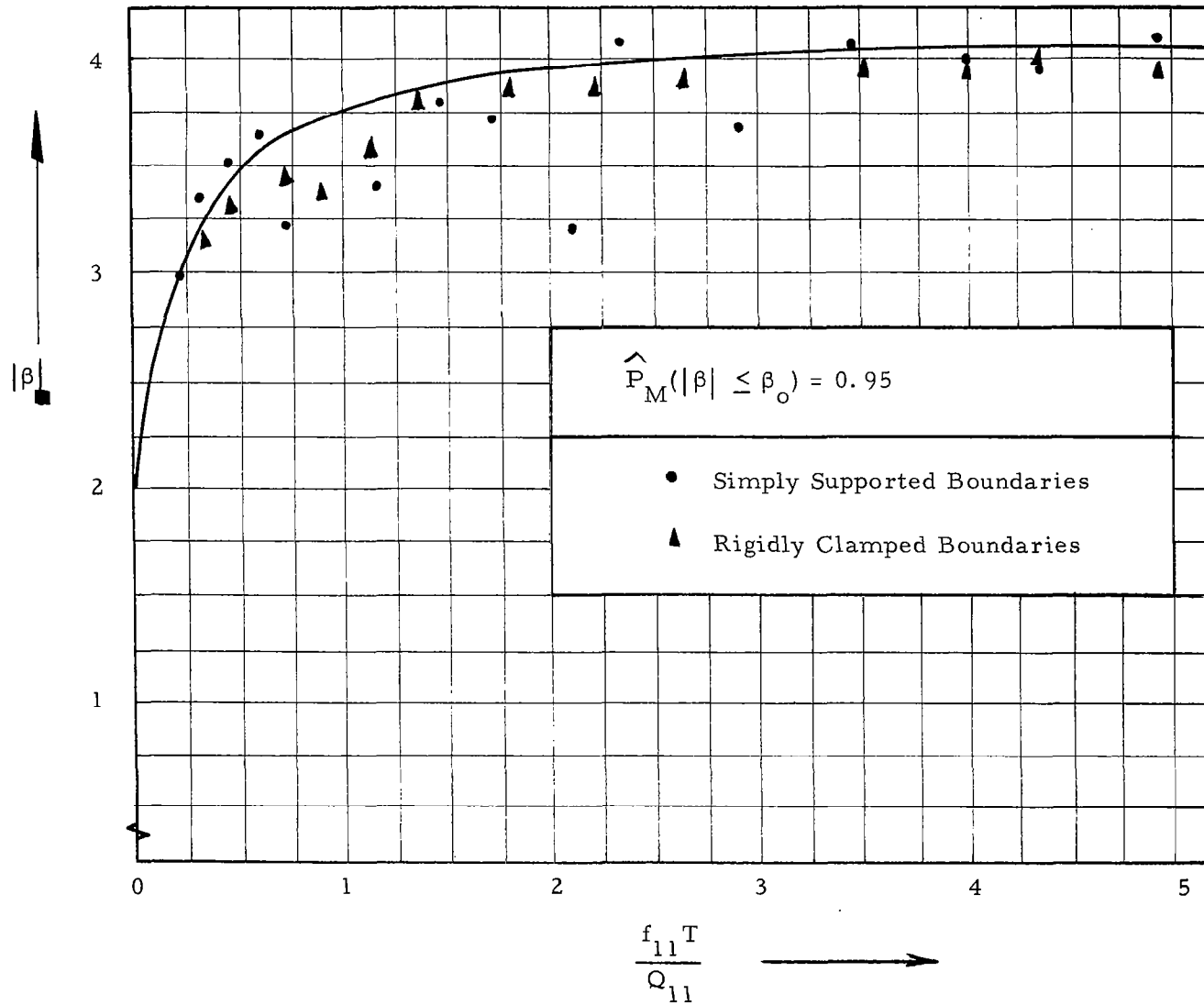
Figure 19. Maximum Response of a Square Plate to White Noise Excitation Correlated Perfectly in Space and Time
