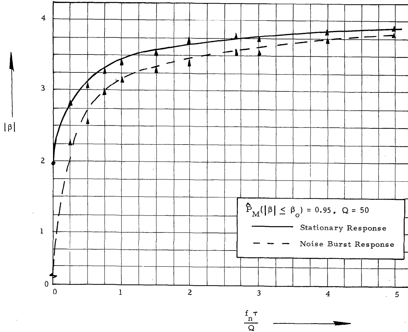
Figure 10. Response Maxima of a Single Degree-of-Freedom System to a Rectangular Burst of White Noise
