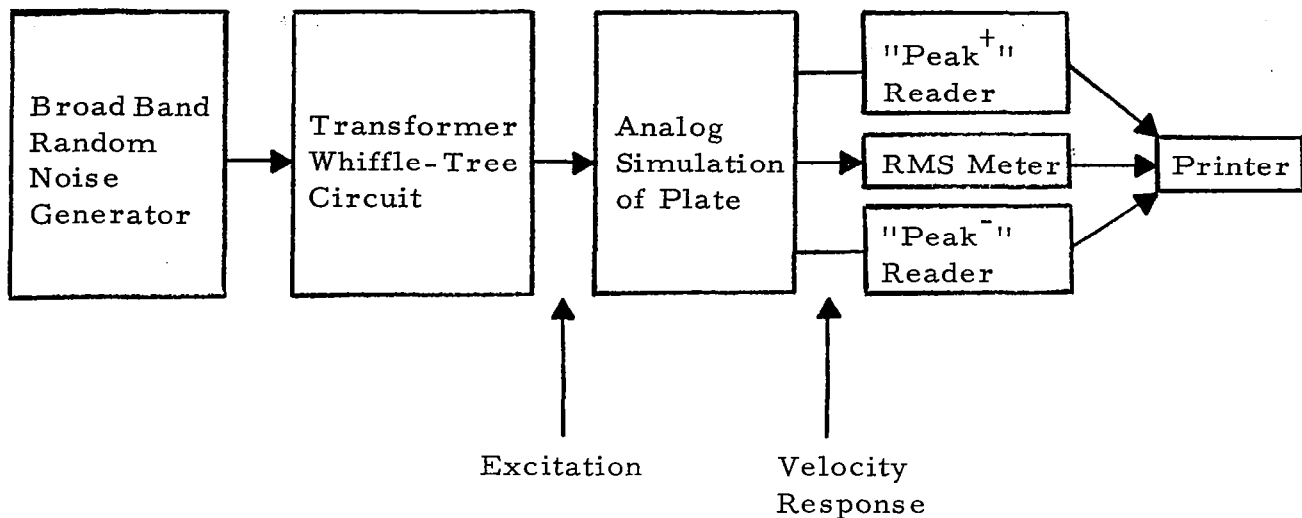
Figure 12. Block Diagram of Analog Simulation Study
