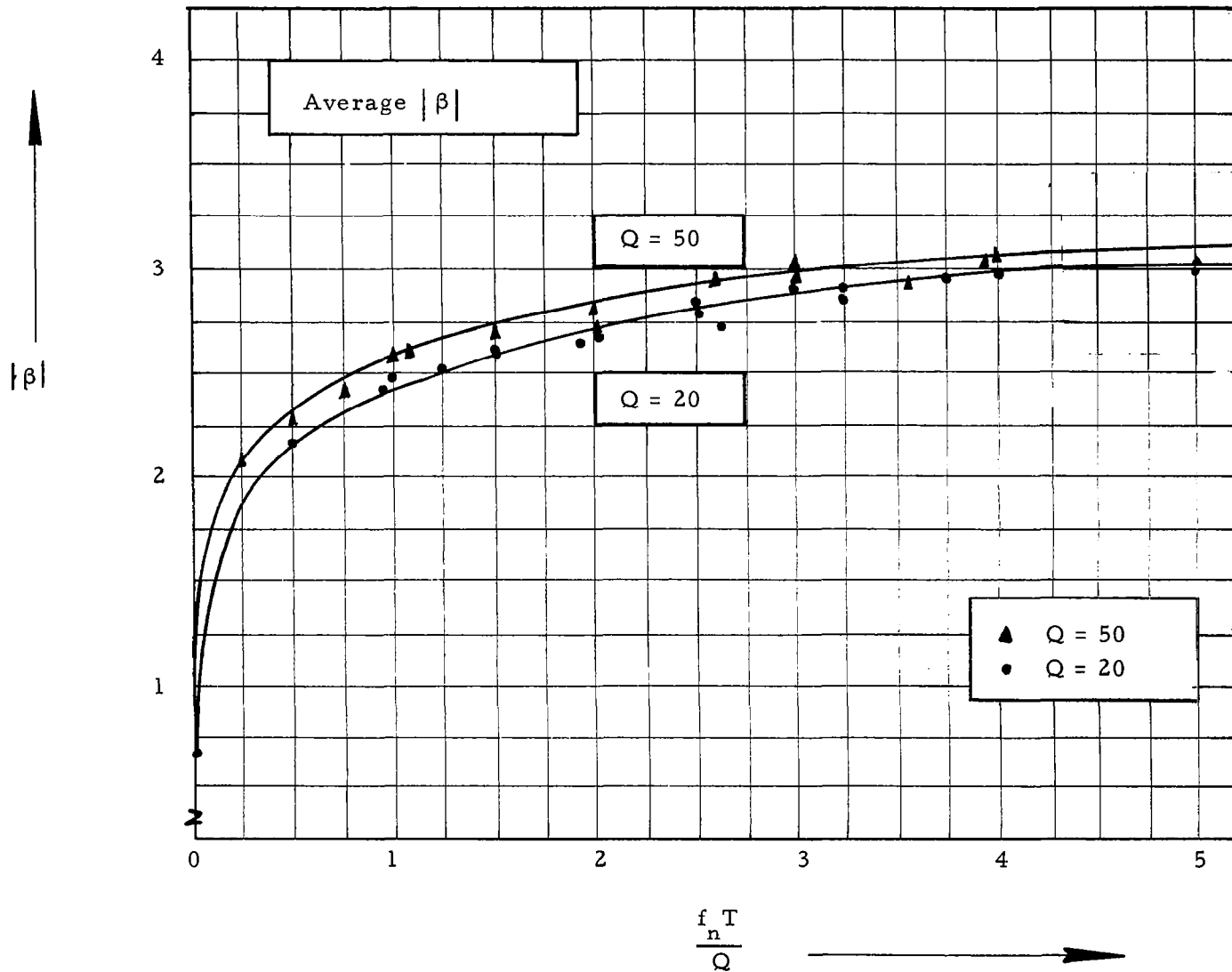
Figure 9. Average Response Maxima of Single Degree-of-Freedom System to Stationary White Noise
