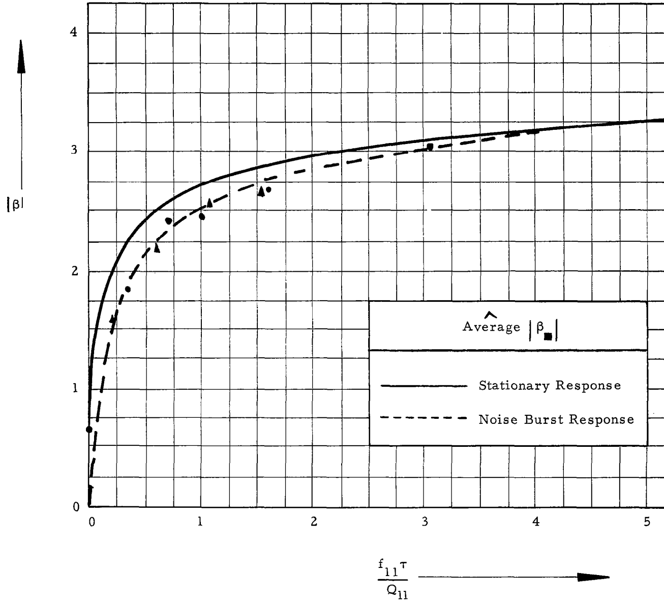
Figure 21. Maximum Response of a Square Plate to Rectangular Bursts of White Noise Correlated Perfectly in Space and Time
