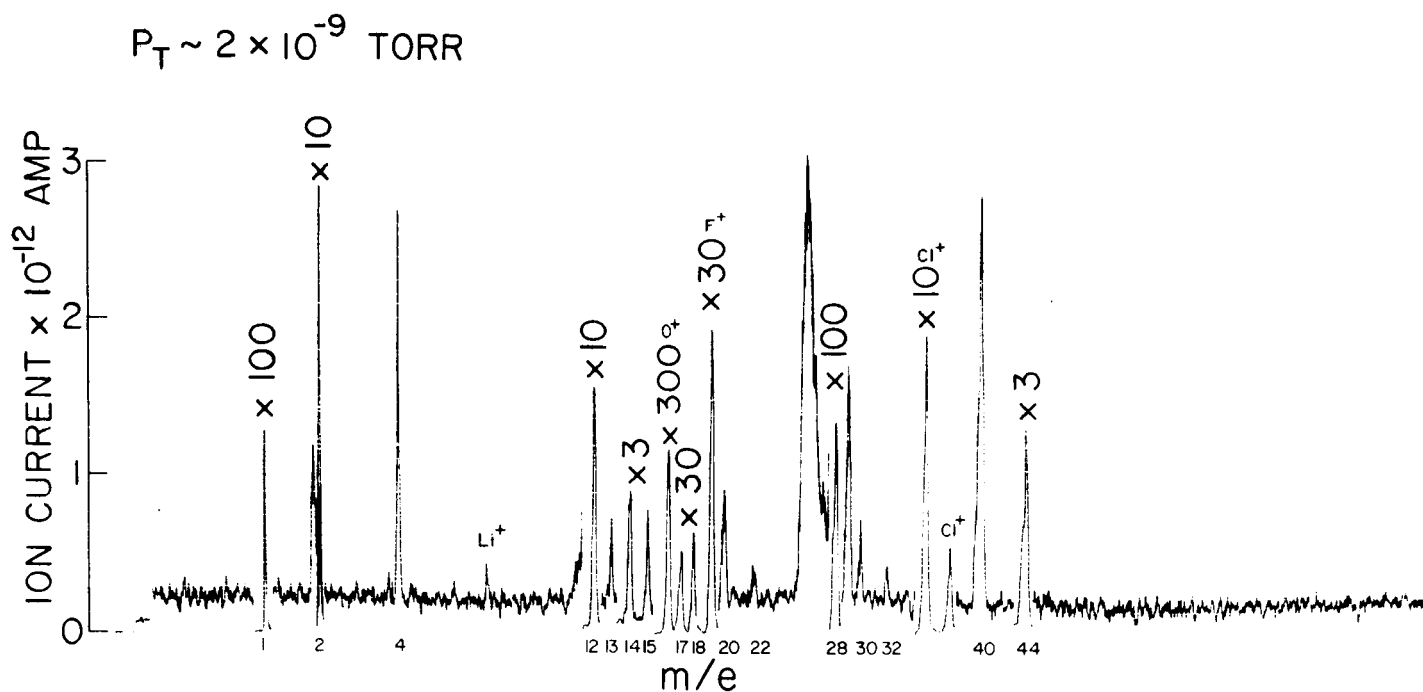
Figure 10 - Residual Gas Spectrum in UHV System Prior to Activation of LHe Cryopump. The spectrum indicates that the limiting gases in the system are H and CO (mass peaks 1 and 28, respectively). The presence of He (mass 4) is due primarily from desorption within the 8 liter/sec getter ion-pump which had been previously exposed to considerable quantities of helium.
