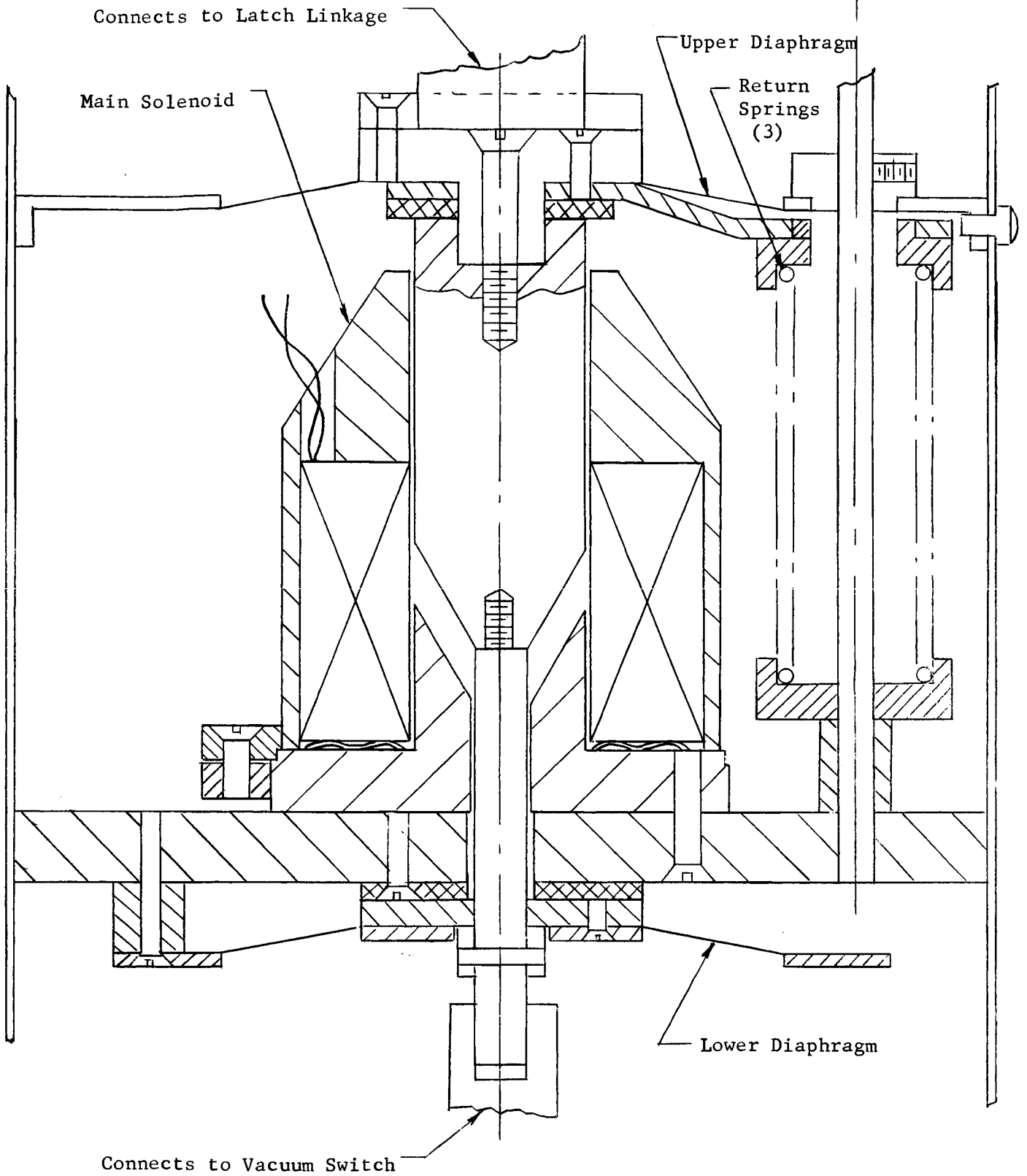
Figure 15. Main Solenoid & Diaphragms
