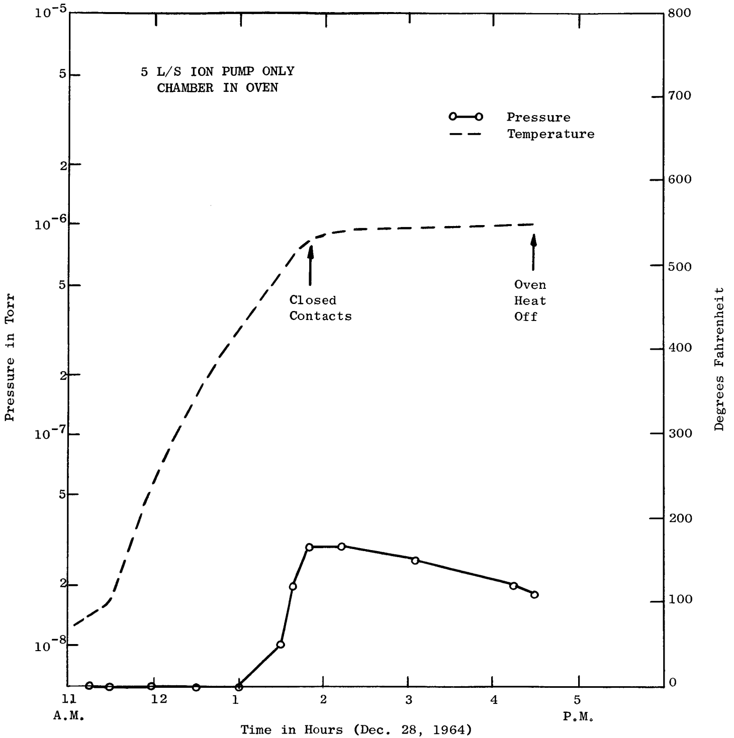
Figure 2. Materials Test Chamber - Temperature and Pressure vs. Time - 550°F Maximum.
