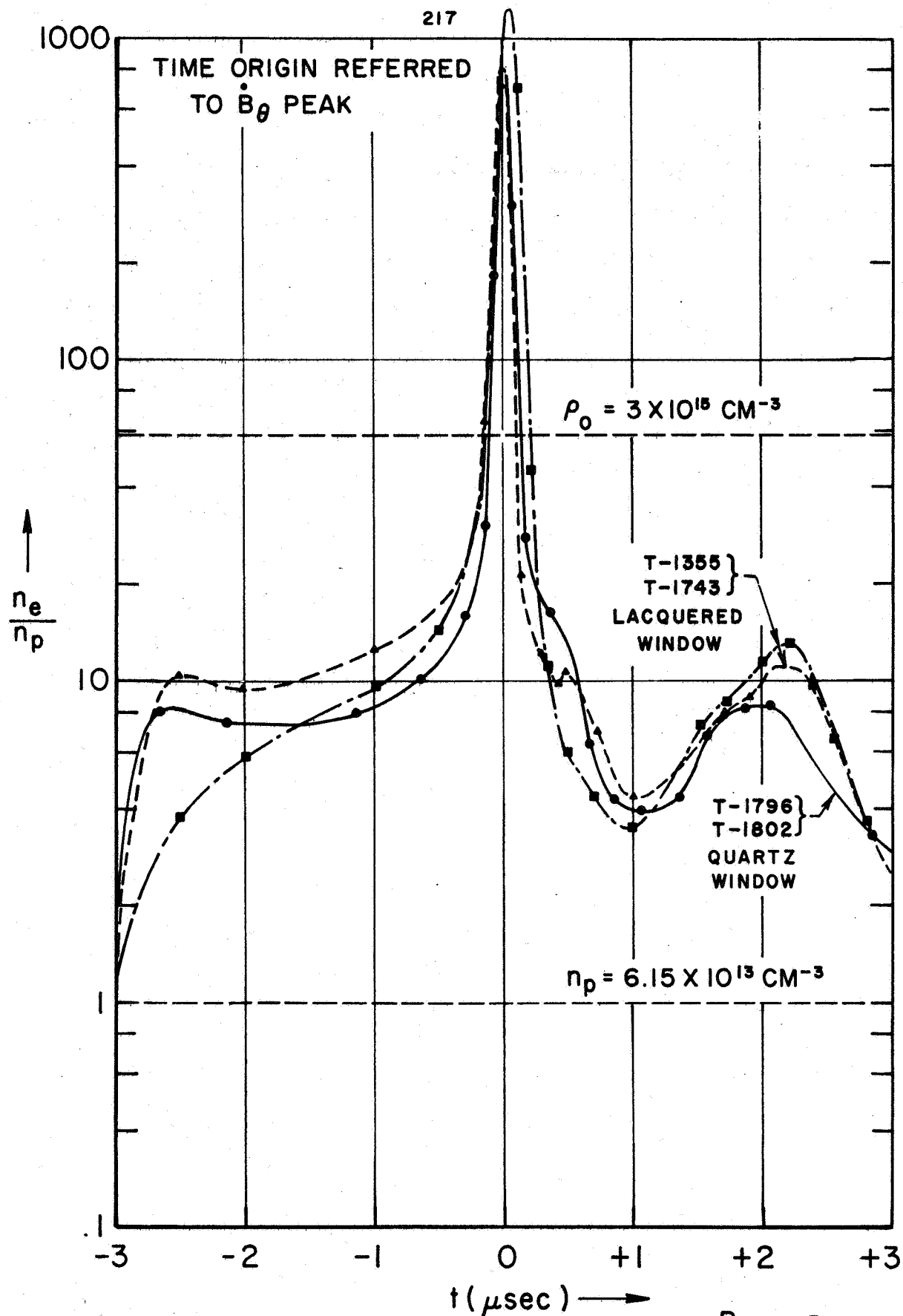
MEASURED ELECTRON DENSITIES AT CATHODE, ( \frac{R}{R_0} = .5, \frac{z}{h} \approx 0 ) FIGURE 6-38
