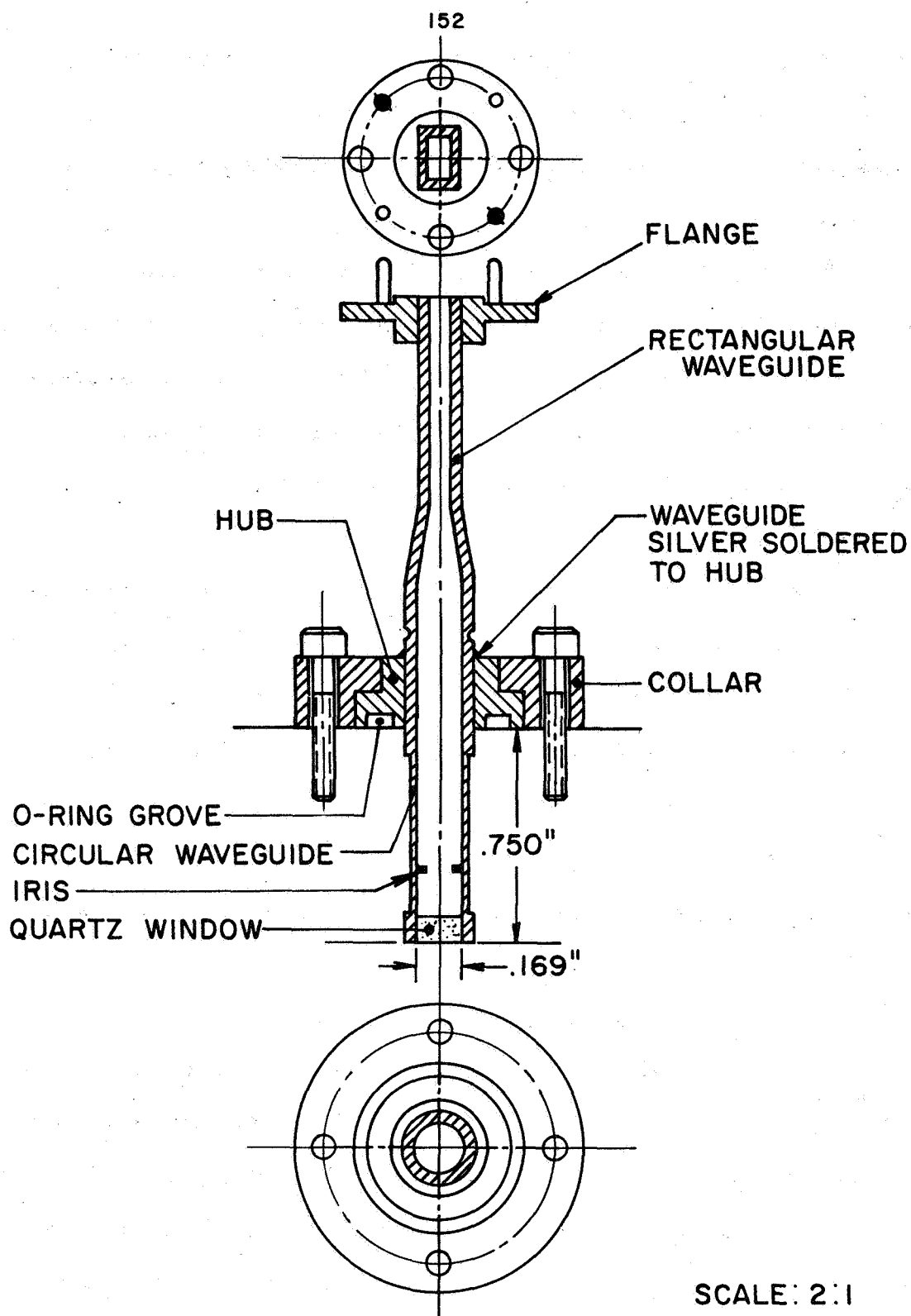
CROSS-SECTION VIEW OF 70 GHz HORN
