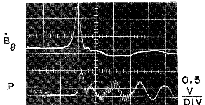
a) RESPONSE OF INSULATED PRESSURE PROBE TO A REFLECTED SHOCK
