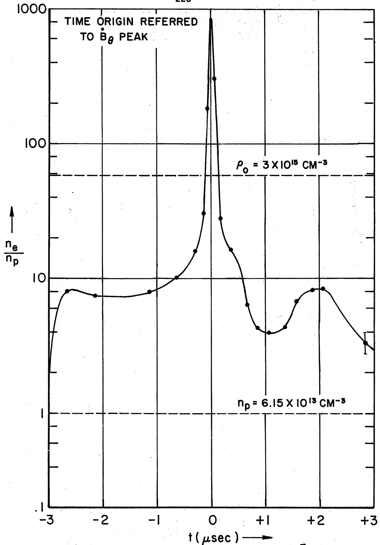
ELECTRON DENSITY AT CATHODE, (\frac{R}{R_0} = .5, \frac{z}{h} \approx 0) FIGURE 6-40
