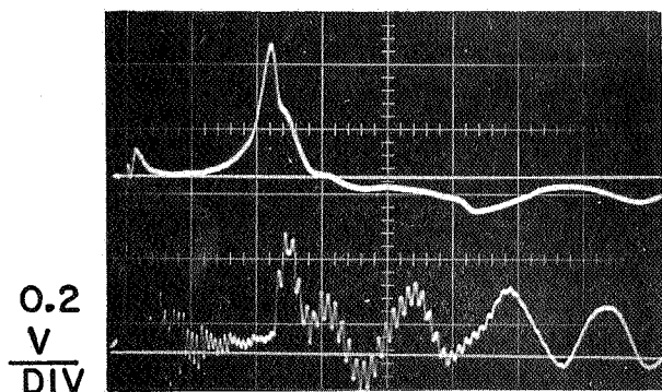
a) RESPONSE OF INSULATED PRESSURE PROBE TO A REFLECTED SHOCK
