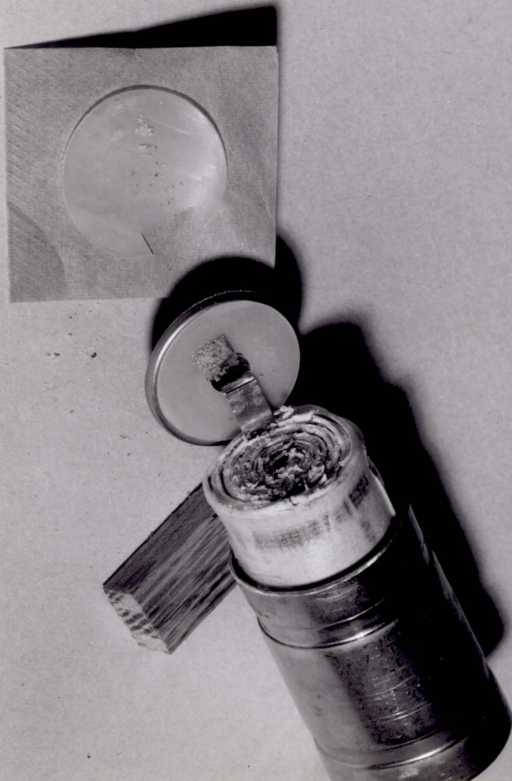
Cell No. 64 Sonotone, 18610 Cycles 10% Depth at 25°C
