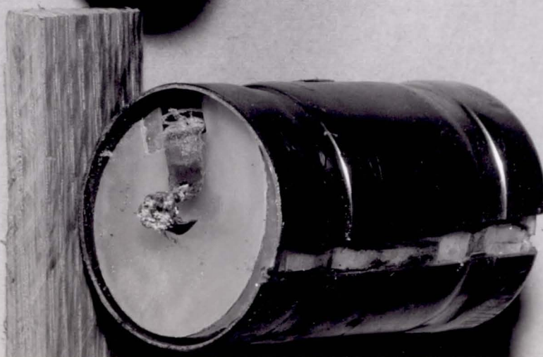
Cell No. R39 Sonotone, 19906 Cycles 10% Depth at 25°C
