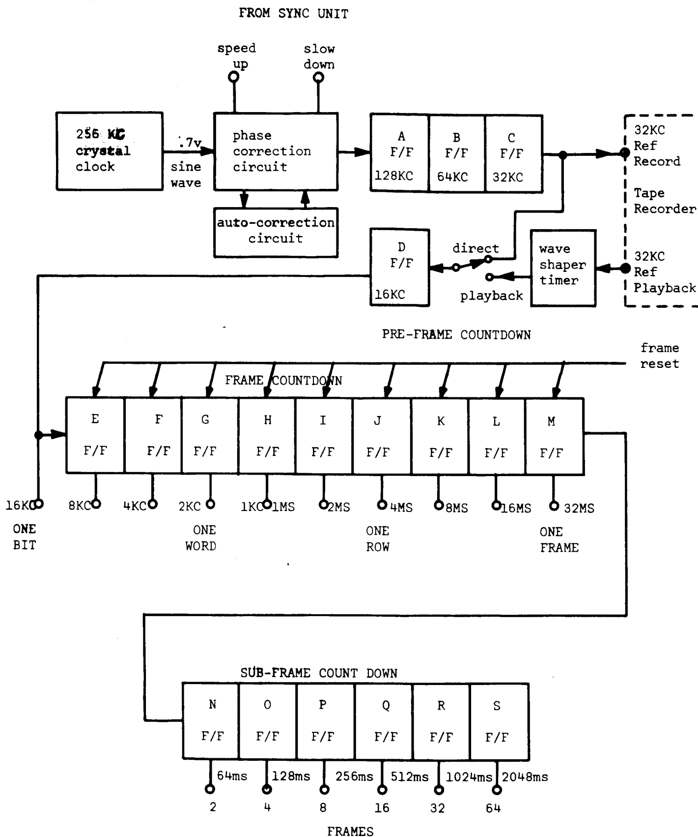
FIGURE 9.3 BLOCK DIAGRAM - TIME BASE
