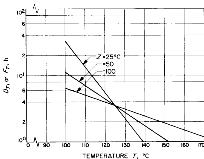
Fig. 5. Thermal destruction curves of different Z values, but with D_{125} = 3.5 h
