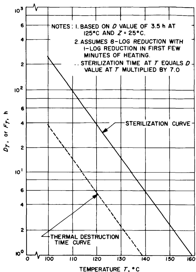
Fig. 4. Thermal destruction and equivalent sterilization time curves
