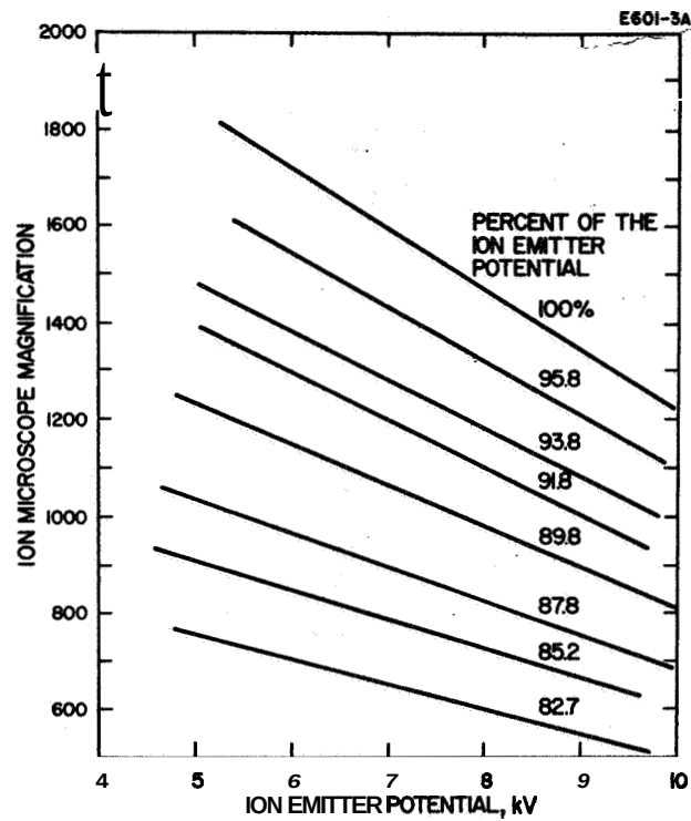
Fig. 34. Ion microscope calibration curves. The immersion lens first electrode is at t600 V. Parameter is the uni- potential lens potential in percent of the emitter potential.
