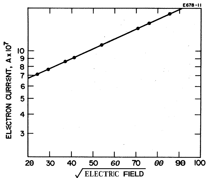
Fig. 10. Schottky effect: The electron current increases proportional to the square root of the electric field, according to i = i_0 \exp \left( \frac{e\sqrt{eE}}{kT} \right) .
