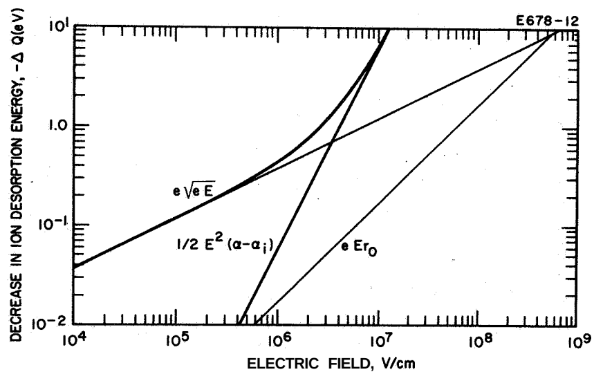
Fig. 14. Change in ion desorption energy with the applied electric field. Considered are the Schottky term e\sqrt{eE} , 1/2E^2(\alpha_o - \alpha_i) , and eEr_o .
