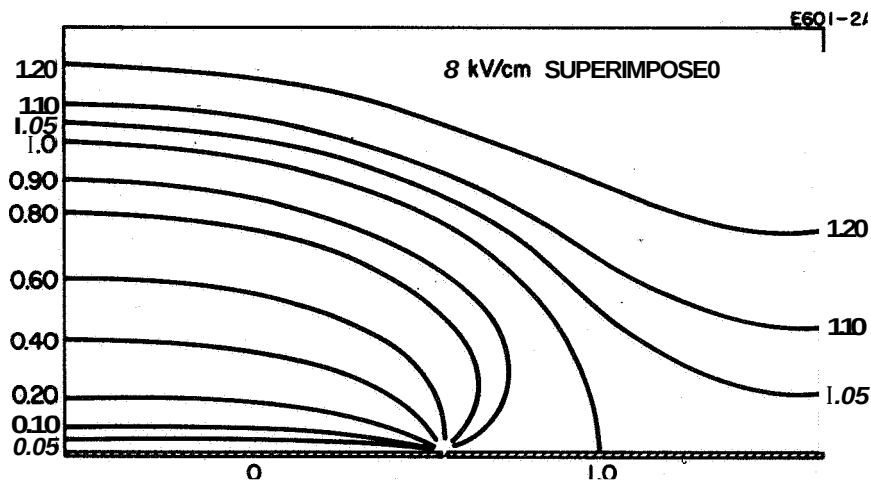
Fig. 49. Equipotential lines on a patch surface with normalized work functions. A field of 8 kV/cm is superimposed.
