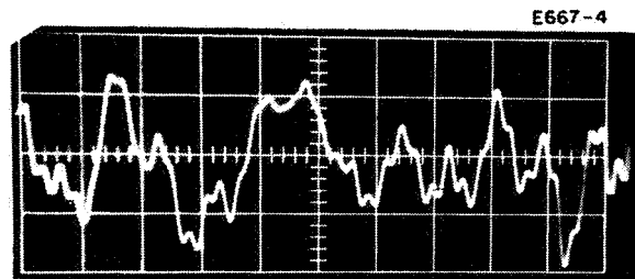
Fig. 32. Vibration diagram, measured at the emitter prior to placing the ion microscope on a 1000 lb concrete block.
