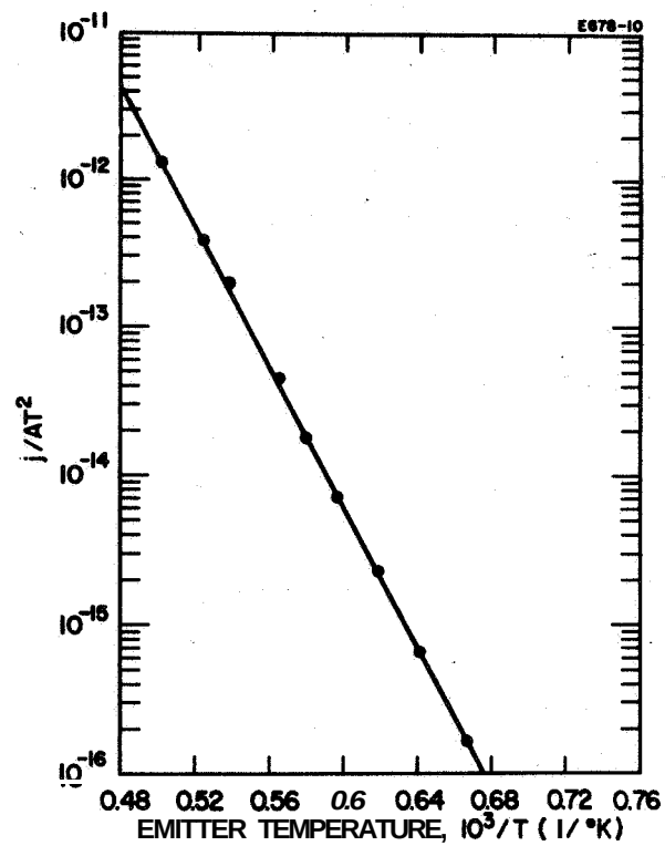
Fig. 11. Richardson plot for W-25% Re alloy. ( j is in A/cm^2 ).
