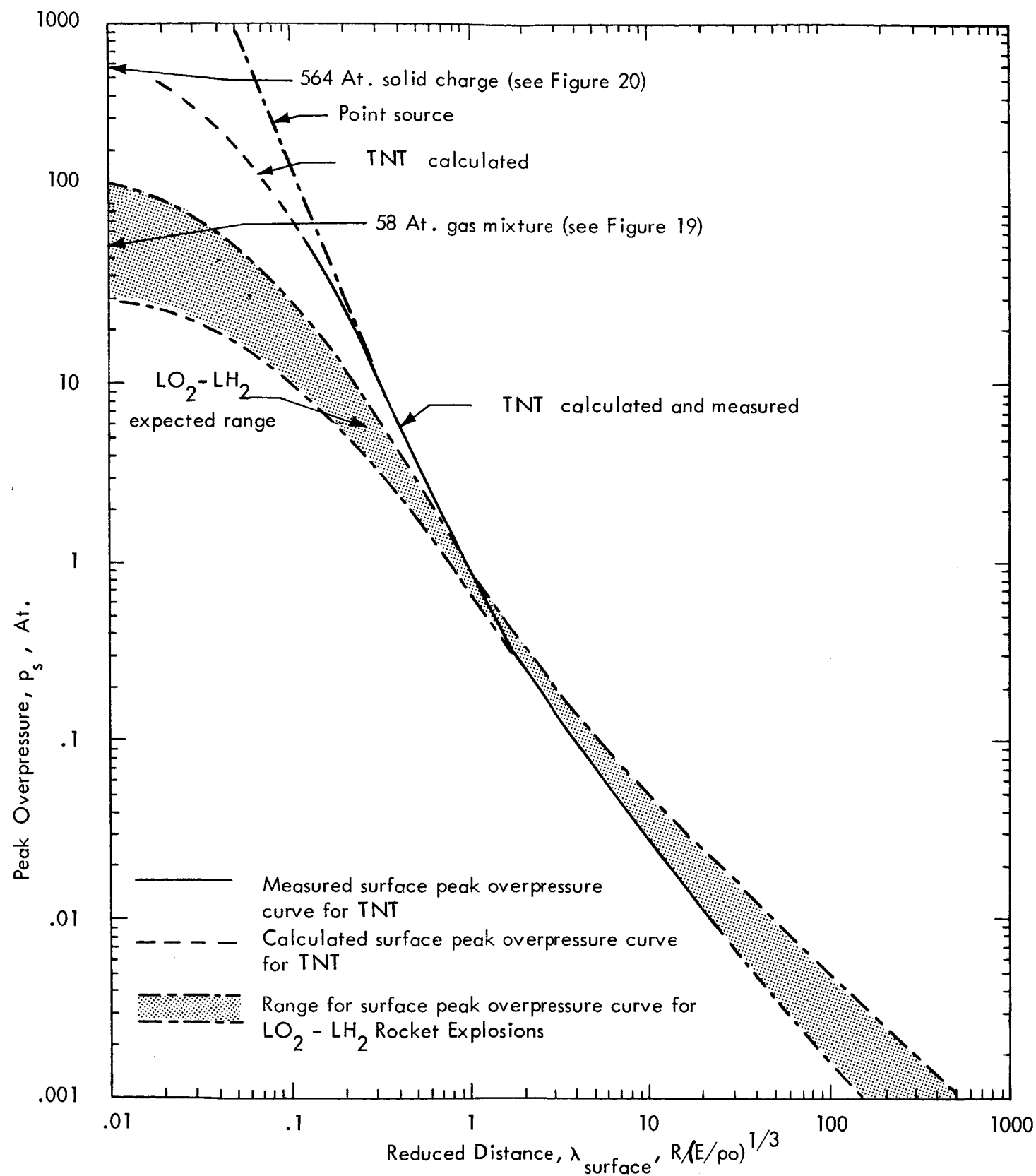
Figure 3. Range within which Surface Peak Overpressure Curve for Explosions of LO 2 - LH 2 Rockets is Expected to Fall, Compared with Measured Surface Peak Overpressure Curve for TNT Explosions of Equal Total Energy
