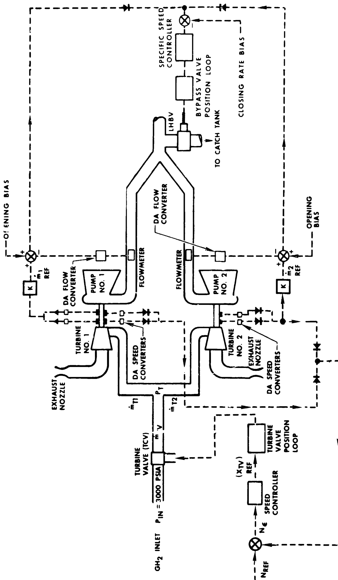
Figure 1. NFS-3 Feed System Schematic
