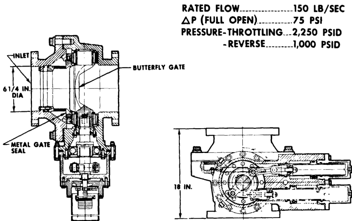
Figure 21. Liquid Hydrogen Bypass Valve
