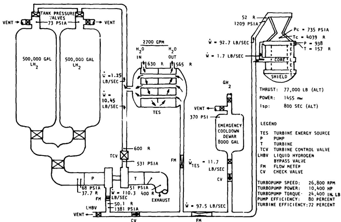
Figure 22. Full-Power Phoebus 1B Operating Parameters
