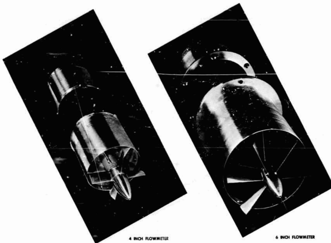
Figure 12. Liquid Hydrogen Turbine Flowmeters
